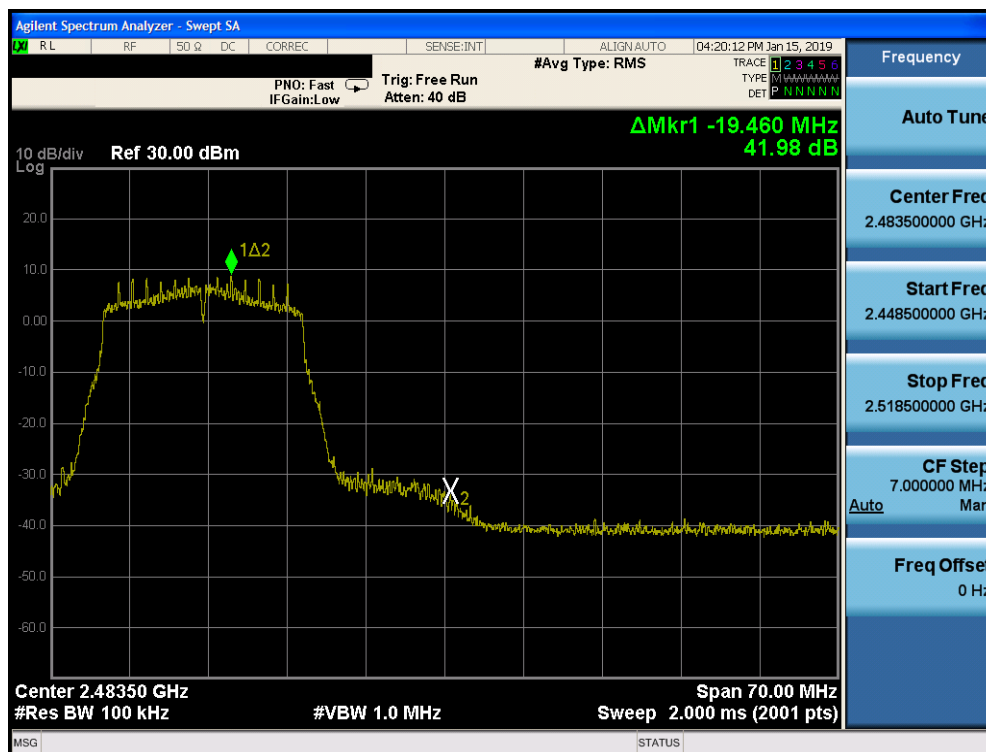
Plot 7-112. Band Edge Plot SISO CORE 1 (802.11n – Ch. 11)
