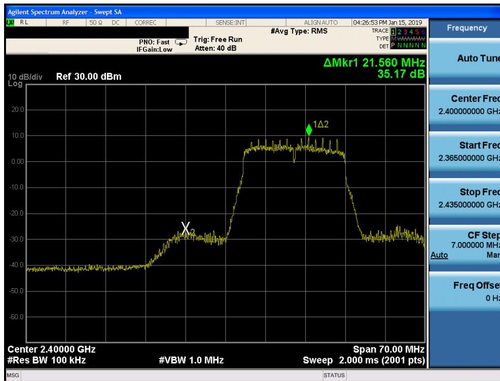
Plot 7-111. Band Edge Plot SISO CORE 1 (802.11n (2.4GHz) – Ch. 1)
