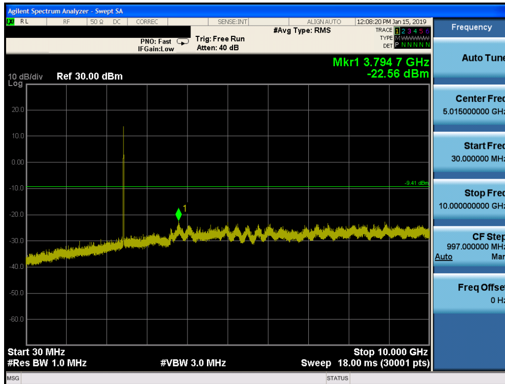
Plot 7-123. Conducted Spurious Plot SISO CORE 0 DIVERSITY (802.11b – Ch. 6)
