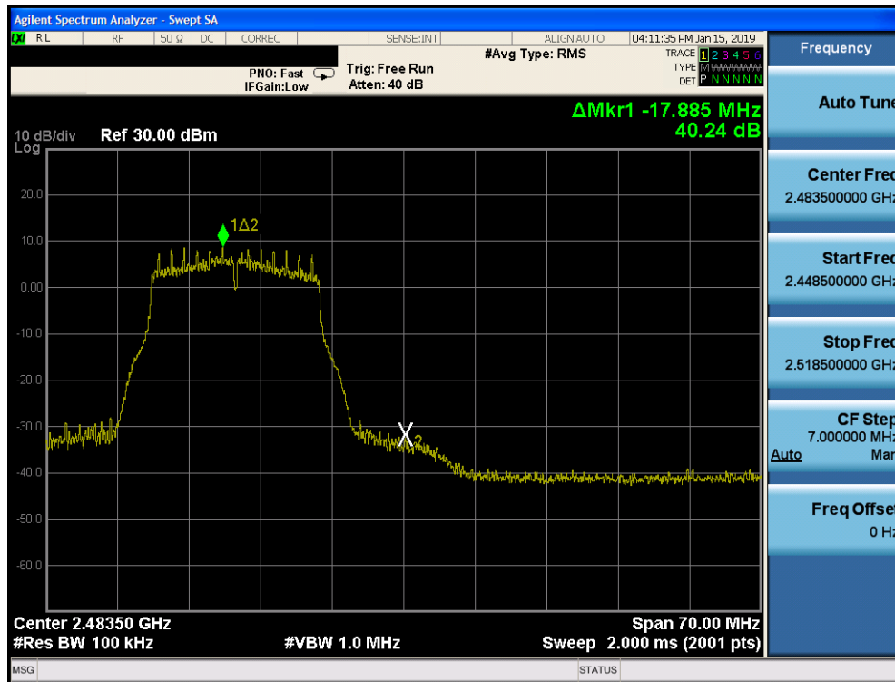
Plot 7-109. Band Edge Plot SISO CORE 1 (802.11g – Ch. 12)
