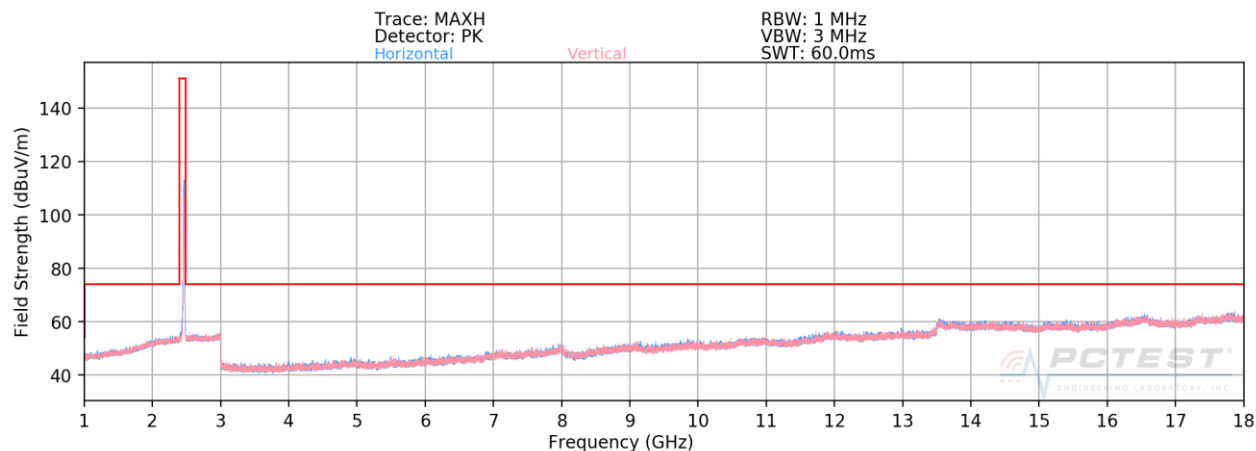
Plot 7-138. Radiated Spurious Plot above 1GHz SISO CORE 0 DIVERSITY (802.11b – Ch. 11)
