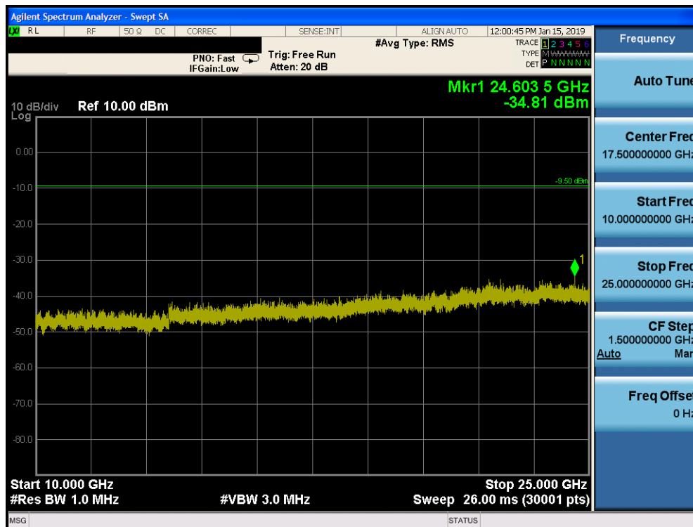
Plot 7-122. Conducted Spurious Plot SISO CORE 0 DIVERSITY (802.11b – Ch. 1)
