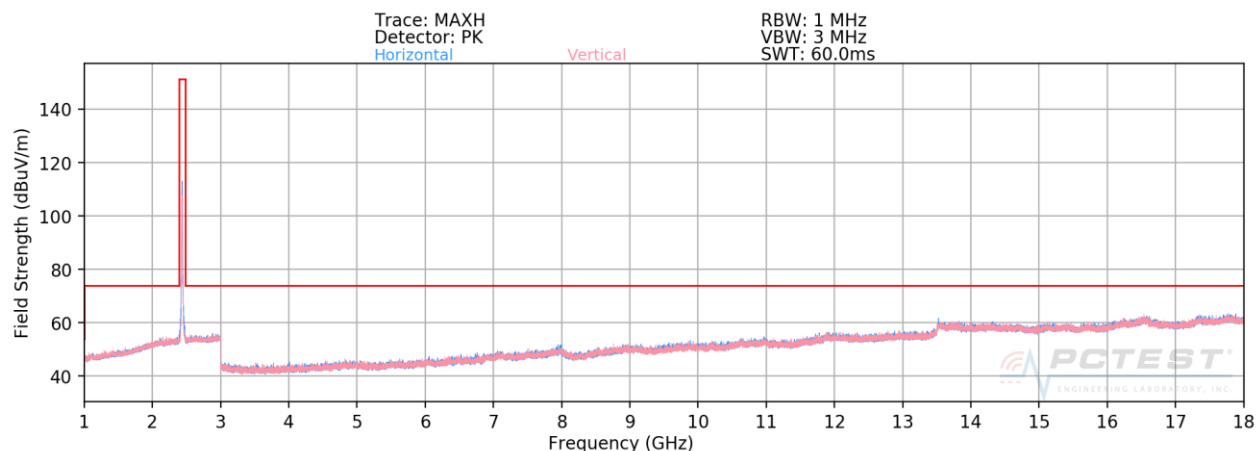
Plot 7-137. Radiated Spurious Plot above 1GHz SISO CORE 0 DIVERSITY (802.11b – Ch. 6)
