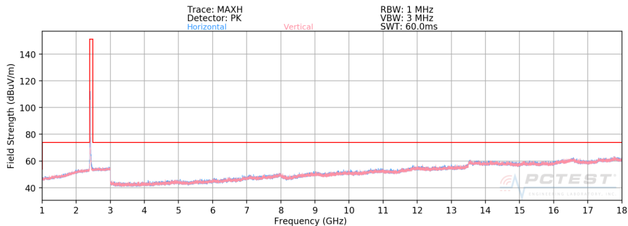
Plot 7-136. Radiated Spurious Plot above 1GHz SISO CORE 0 DIVERSITY (802.11b – Ch. 1)
