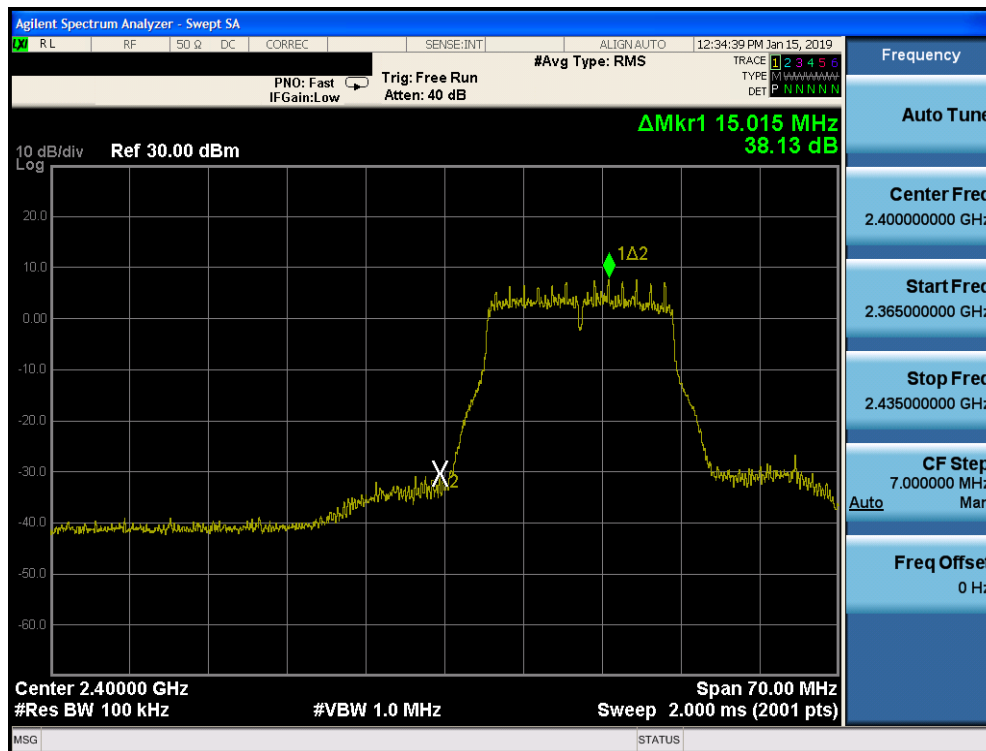
Plot 7-95. Band Edge Plot SISO CORE 0 DIVERSITY (802.11g– Ch. 1)
