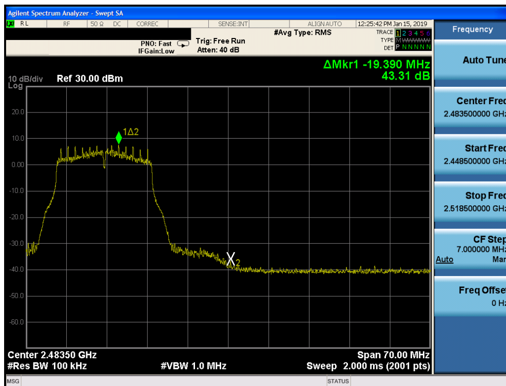
Plot 7-96. Band Edge Plot SISO CORE 0 DIVERSITY (802.11g – Ch. 11)
