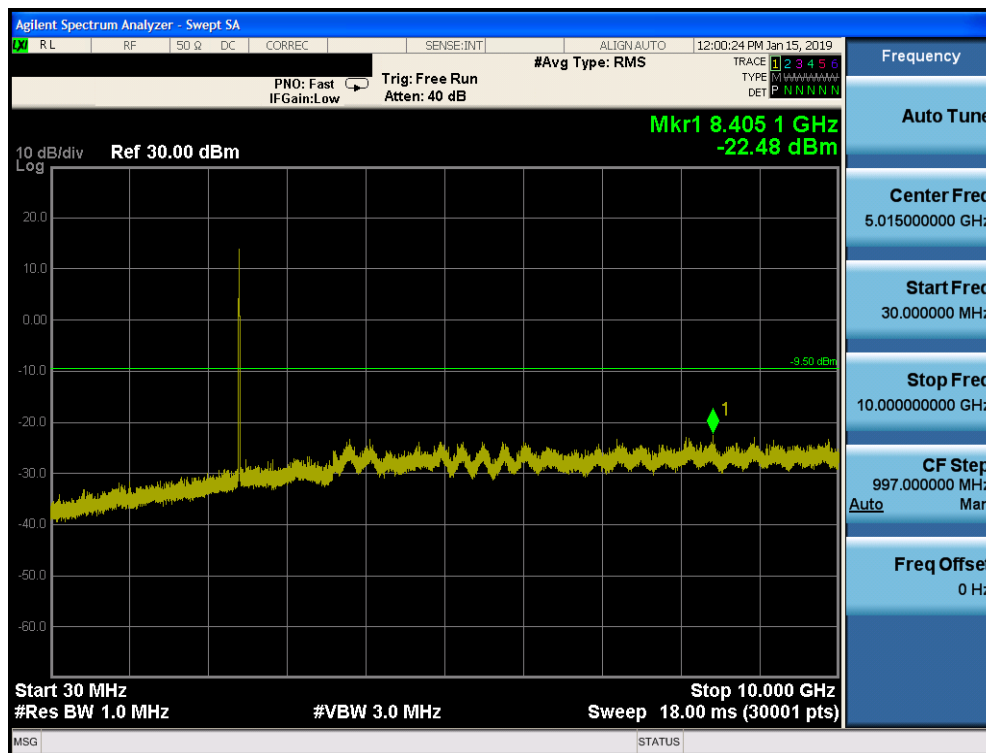
Plot 7-121. Conducted Spurious Plot SISO CORE 0 DIVERSITY (802.11b – Ch. 1)
