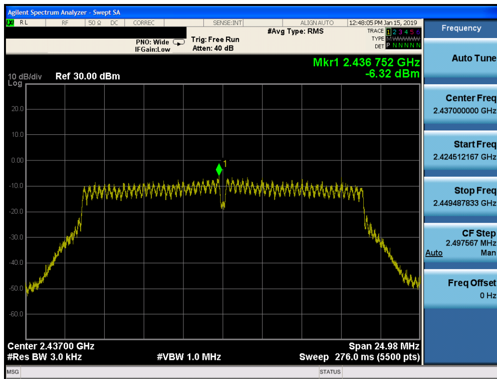
Plot 7-44. Power Spectral Density Plot SISO CORE 0 DIVERSITY (802.11n (2.4GHz) – Ch. 6)
