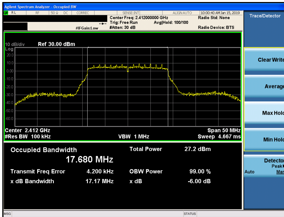
Plot 7-7. 6dB Bandwidth Plot SISO CORE 0 PRIMARY (802.11n (2.4GHz) – Ch. 1)
