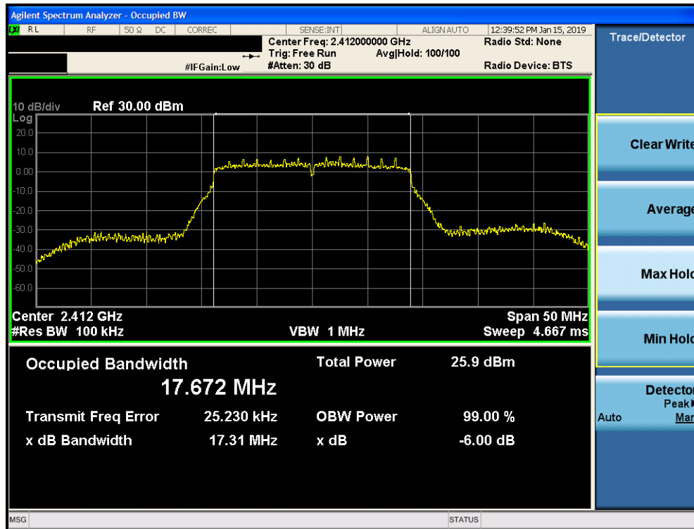
Plot 7-16. 6dB Bandwidth Plot SISO CORE 0 DIVERSITY (802.11n (2.4GHz) – Ch. 1)
