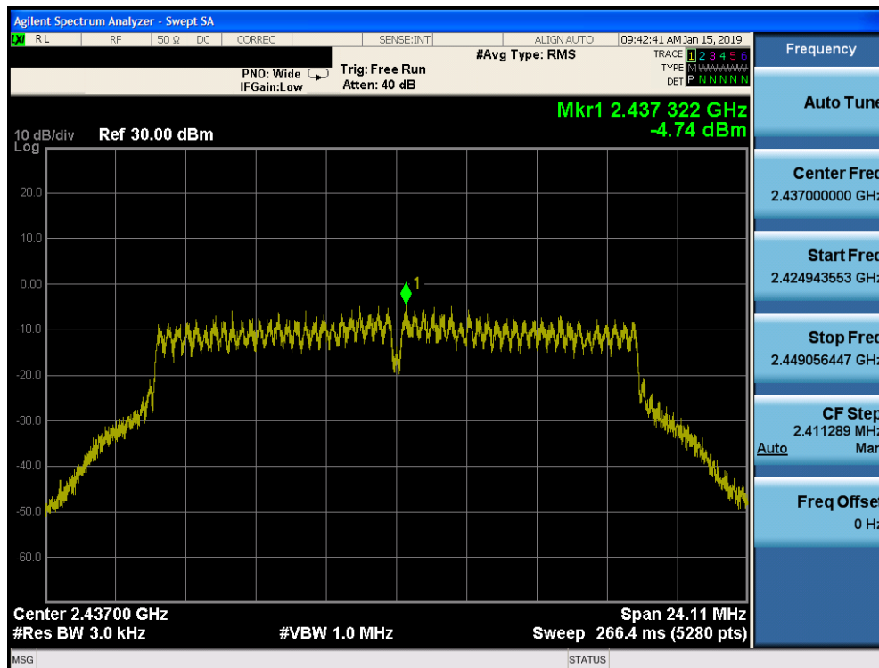
Plot 7-32. Power Spectral Density Plot SISO CORE 0 PRIMARY (802.11g – Ch. 6)
