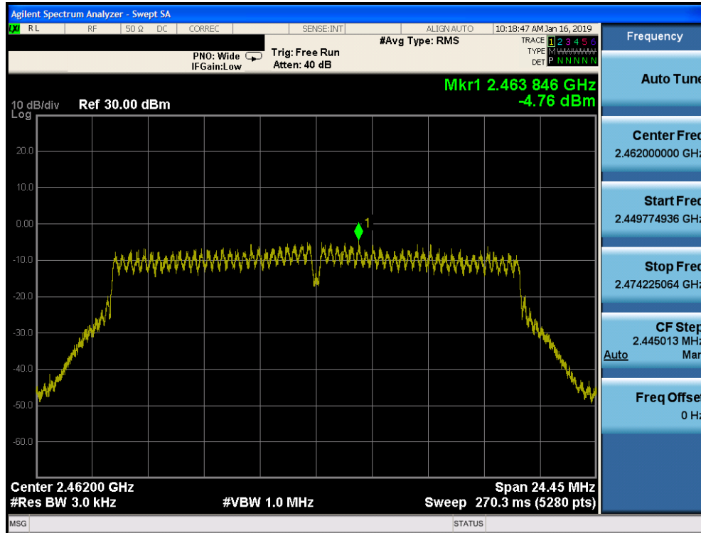
Plot 7-65. Power Spectral Density Plot CDD PRIMARY CORE 0 (802.11n (2.4GHz) – Ch. 11)
