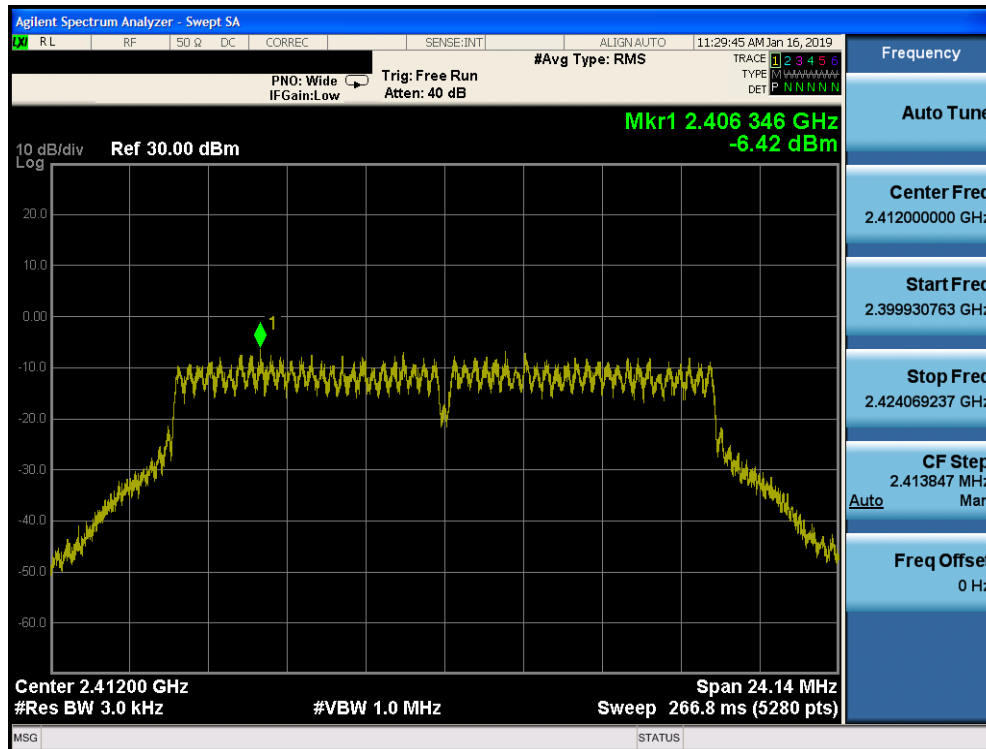
Plot 7-67. Power Spectral Density Plot CDD DIVERSITY CORE 0 (802.11g – Ch. 1)
