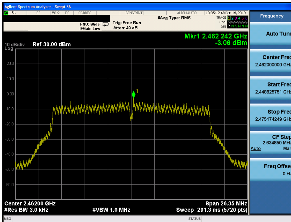
Plot 7-66. Power Spectral Density Plot CDD PRIMARY CORE 1 (802.11n (2.4GHz) – Ch. 11)
