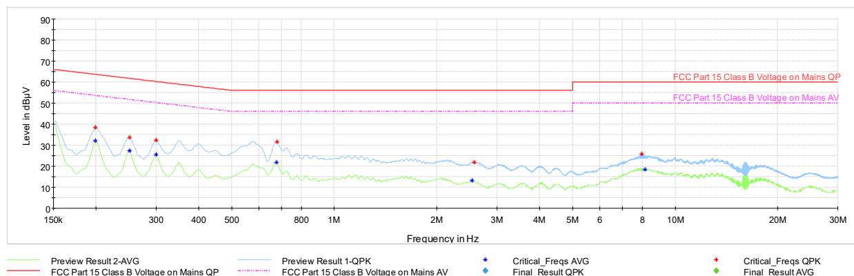
Plot 7-110. Line Conducted Plot with Bluetooth HDR4 – Ch.39 (N, with AC/DC Adapter)
