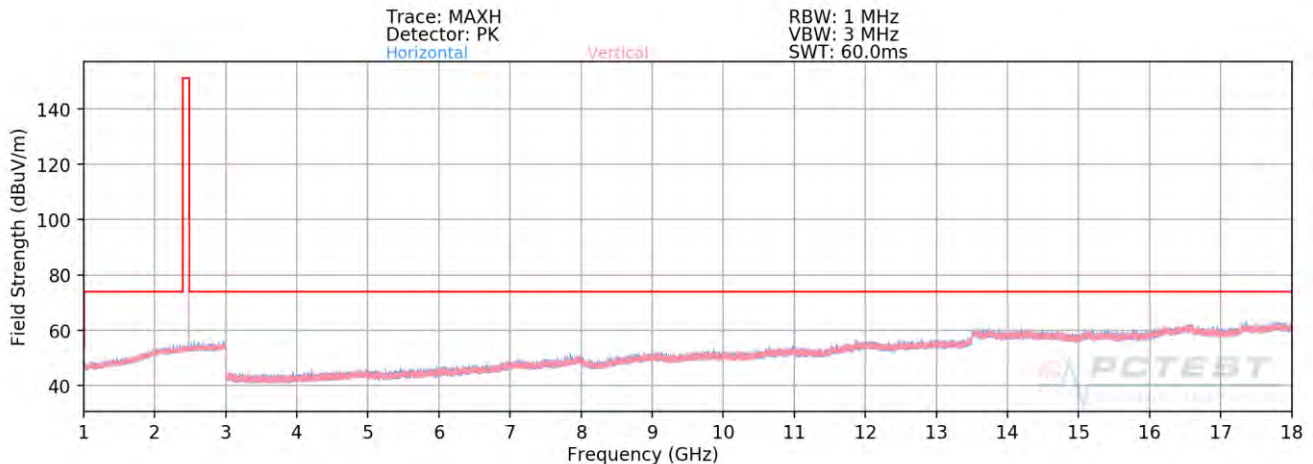
Plot 7-87. Radiated Spurious Plot 1-18GHz Ant-0 (4Mbps, HDR4, ePA – Ch. 75, Ant. Pol. H & V)
