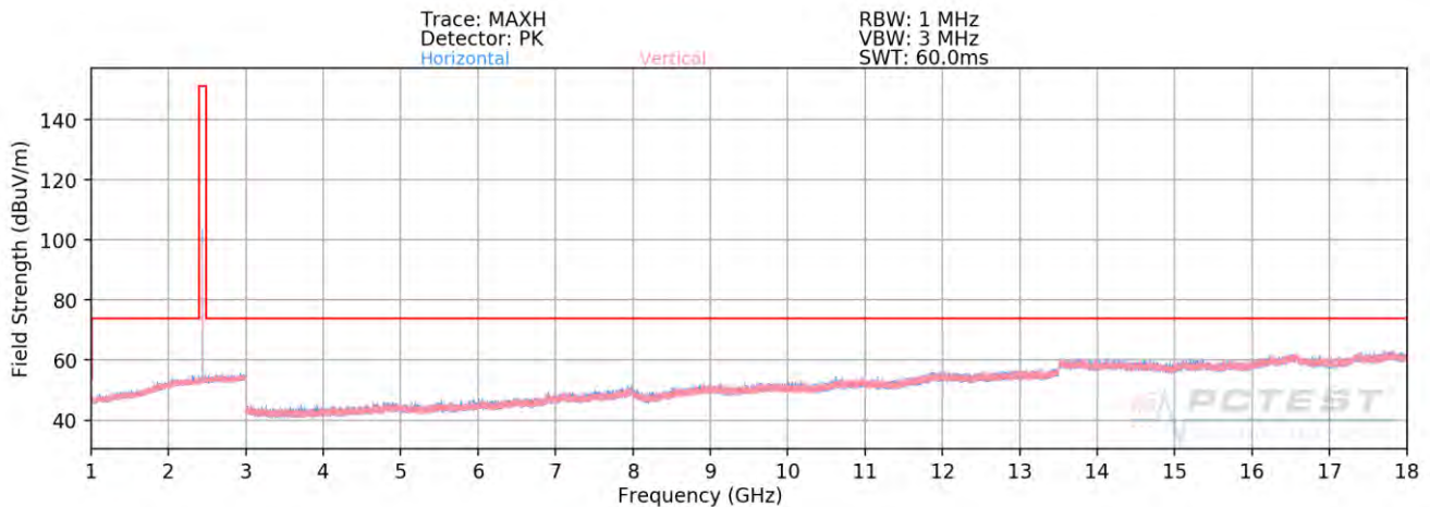
Plot 7-89. Radiated Spurious Plot 1-18GHz Ant-1 (4Mbps, HDR4, ePA – Ch. 38, Ant. Pol. H & V)
