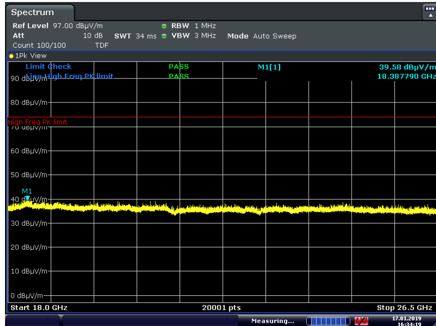
Plot 7-95. Radiated Spurious Plot Above 18GHz Ant-0 (4Mbps, HDR4, ePA – Ch.38, Ant. Pol. V)
