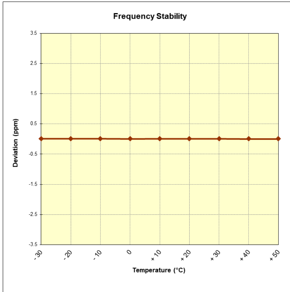
Figure 7-7. Frequency Stability Graph (Band 26)
