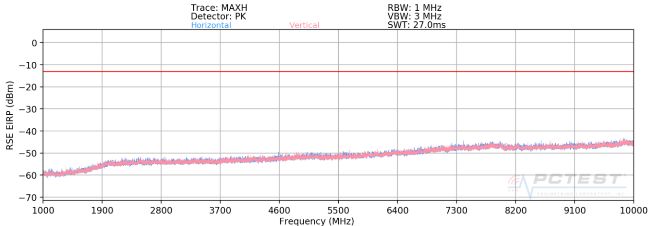
Plot 7-51. Radiated Spurious Plot above 1GHz (Band 14)
