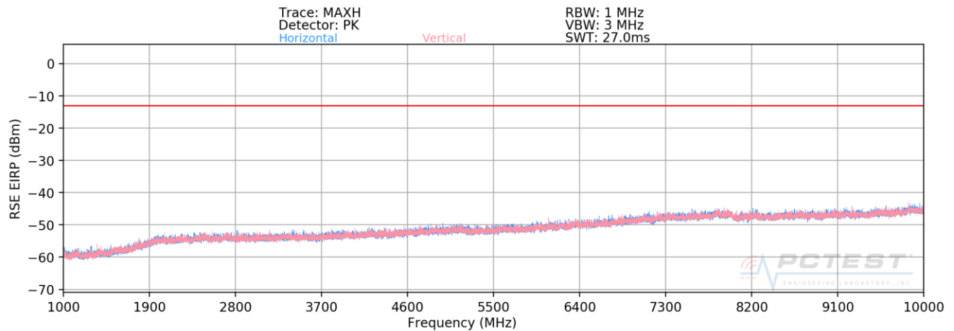
Plot 7-50. Radiated Spurious Plot above 1GHz (Band 26)
