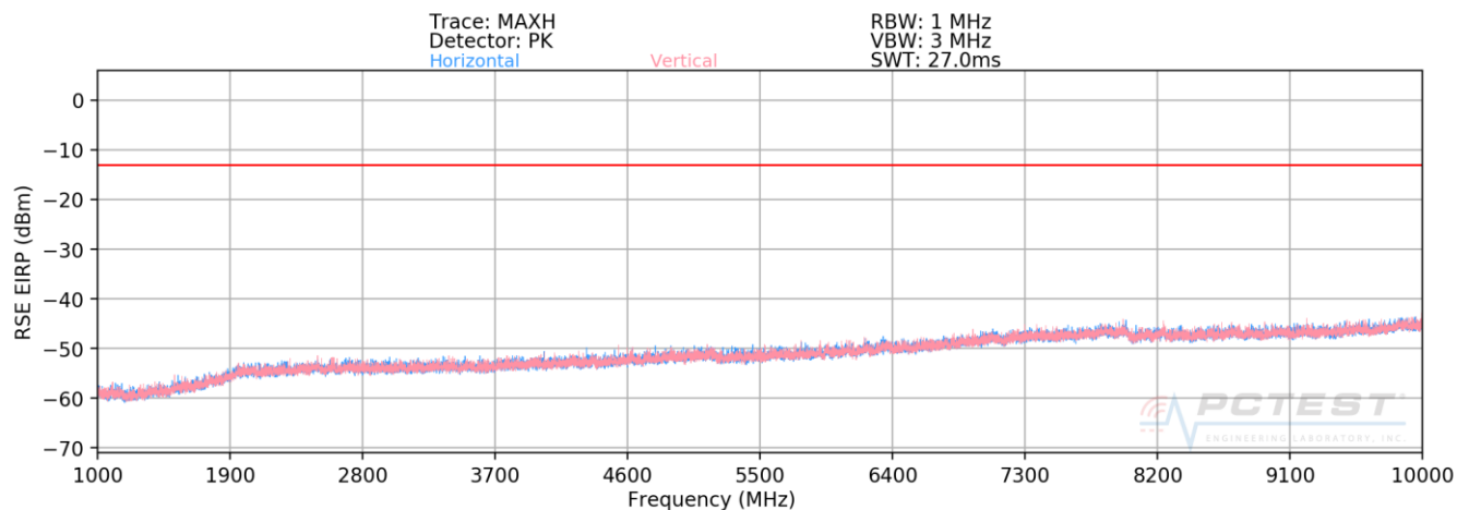
Plot 7-48. Radiated Spurious Plot above 1GHz (Band 26)
