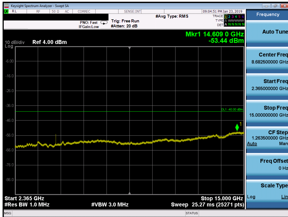
Plot 7-143. Conducted Spurious Plot (Band 30 - 10.0MHz QPSK - RB Size 1, RB Offset 0 - Low Channel)
