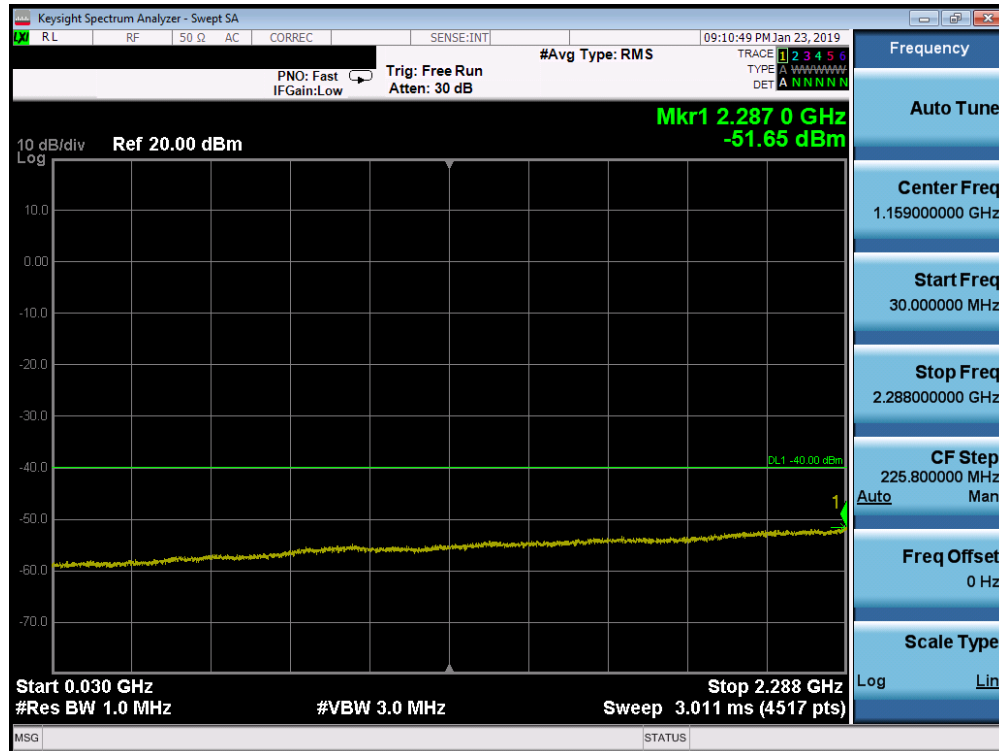
Plot 7-148. Conducted Spurious Plot (Band 30 - 10.0MHz QPSK - RB Size 1, RB Offset 0 - High Channel)
