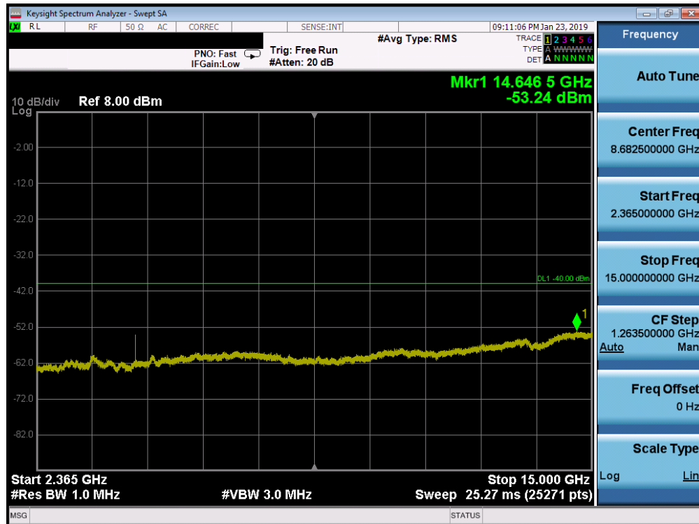
Plot 7-149. Conducted Spurious Plot (Band 30 - 10.0MHz QPSK - RB Size 1, RB Offset 0 - High Channel)
