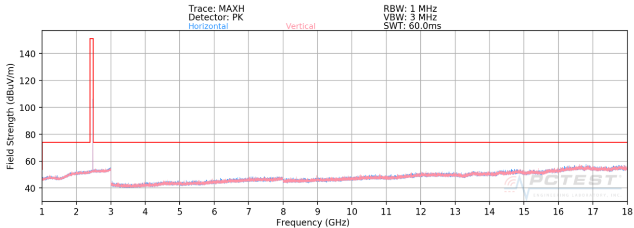
Plot 7-59. Radiated Spurious Plot Above 1GHz Ant-0 (4Mbps, HDR4, ePA – Ch. 75, Ant. Pol. H & V)
