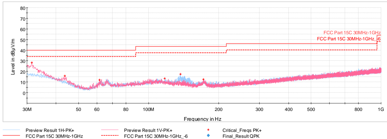
Plot 7-73. Radiated Spurious Plot below 1GHz (4Mbps, HDR4 ePA – Ch.38, Pol. H & V, with Charger)
