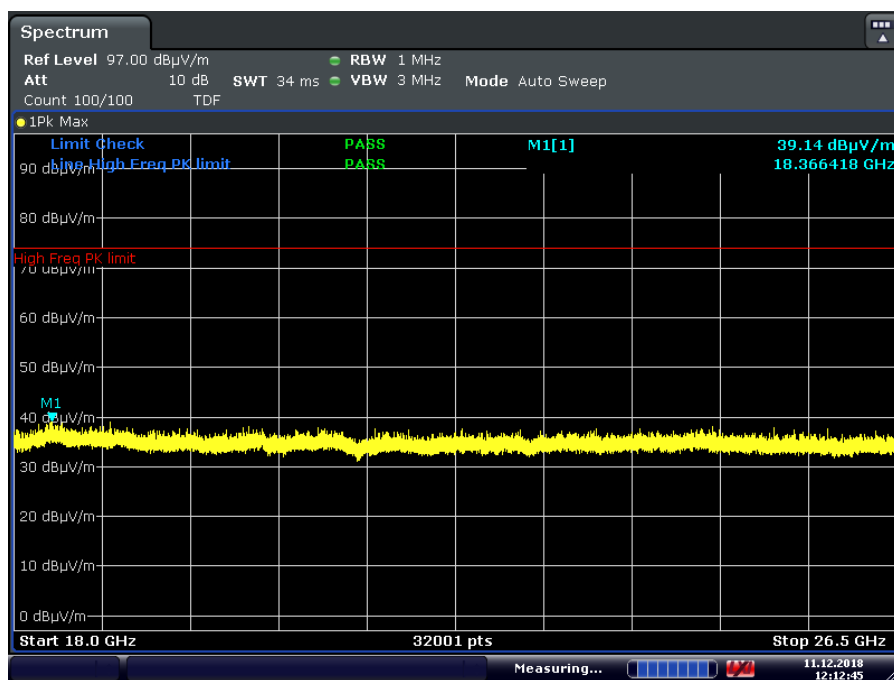
Plot 7-76. Radiated Spurious Plot above 18GHz (GFSK ePA – Ch. 39, Pol. V)
