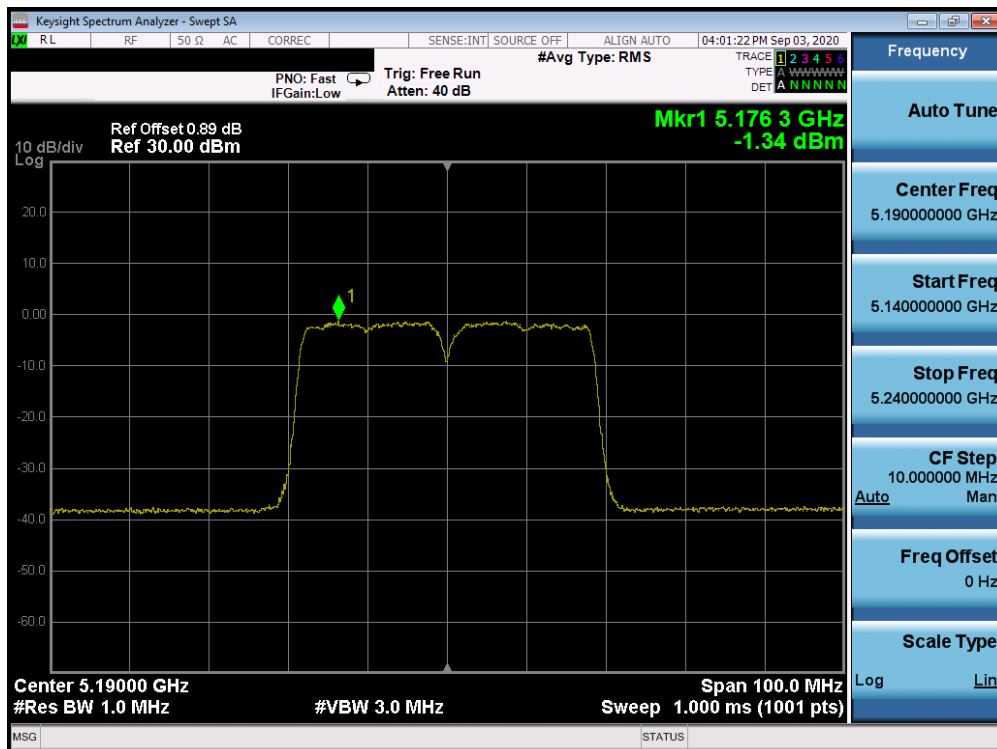
Plot 7-254. ISED Power Spectral Density Plot SDM Diversity Antenna 2b (40MHz BW 802.11n (UNII Band 1) – Ch. 38)
