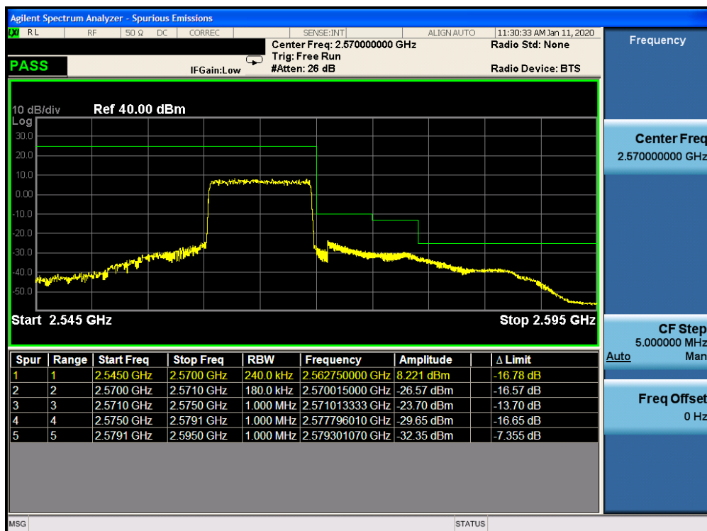
Plot 7-341. Upper ACP Plot (Band 7 – 10.0MHz QPSK – RB Size 50)
