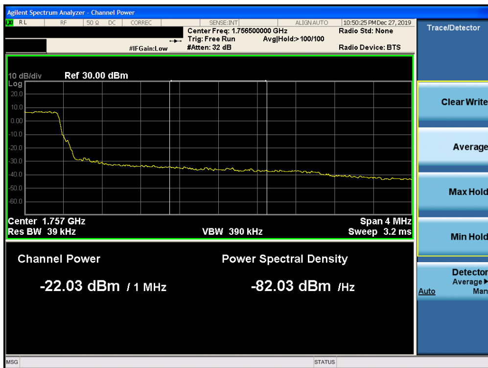
Plot 7-241. Upper Extended Band Edge Plot (Band 4 – 3.0MHz QPSK – RB Size 15)
