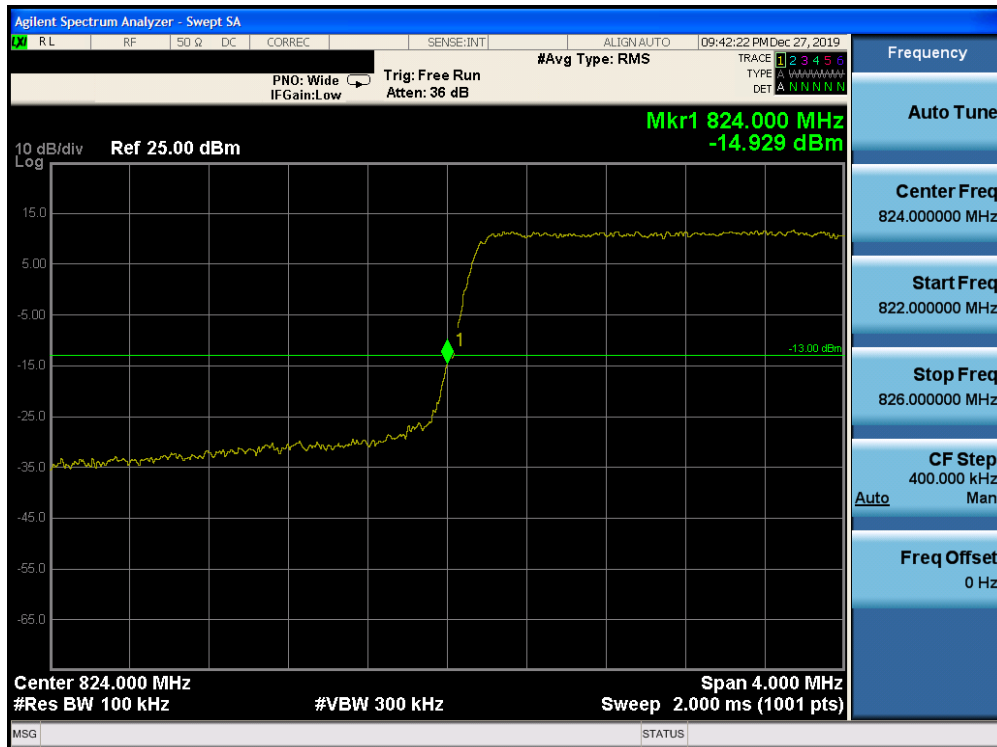
Plot 7-228. Lower Band Edge Plot (Band 5 - 3.0MHz QPSK - RB Size 15)
