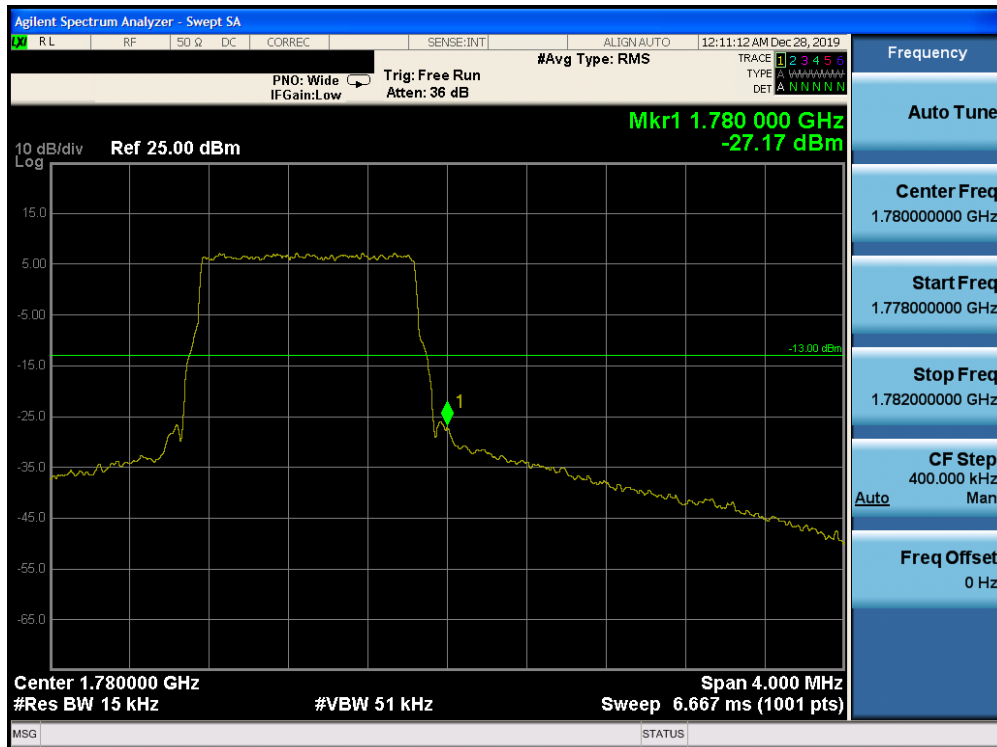
Plot 7-260. Upper Band Edge Plot (Band 66 – 1.4MHz QPSK – RB Size 6)
