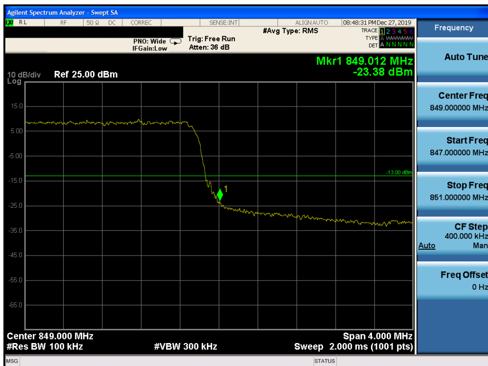
Plot 7-231. Upper Band Edge Plot (Band 5 – 5.0MHz QPSK – RB Size 25)
