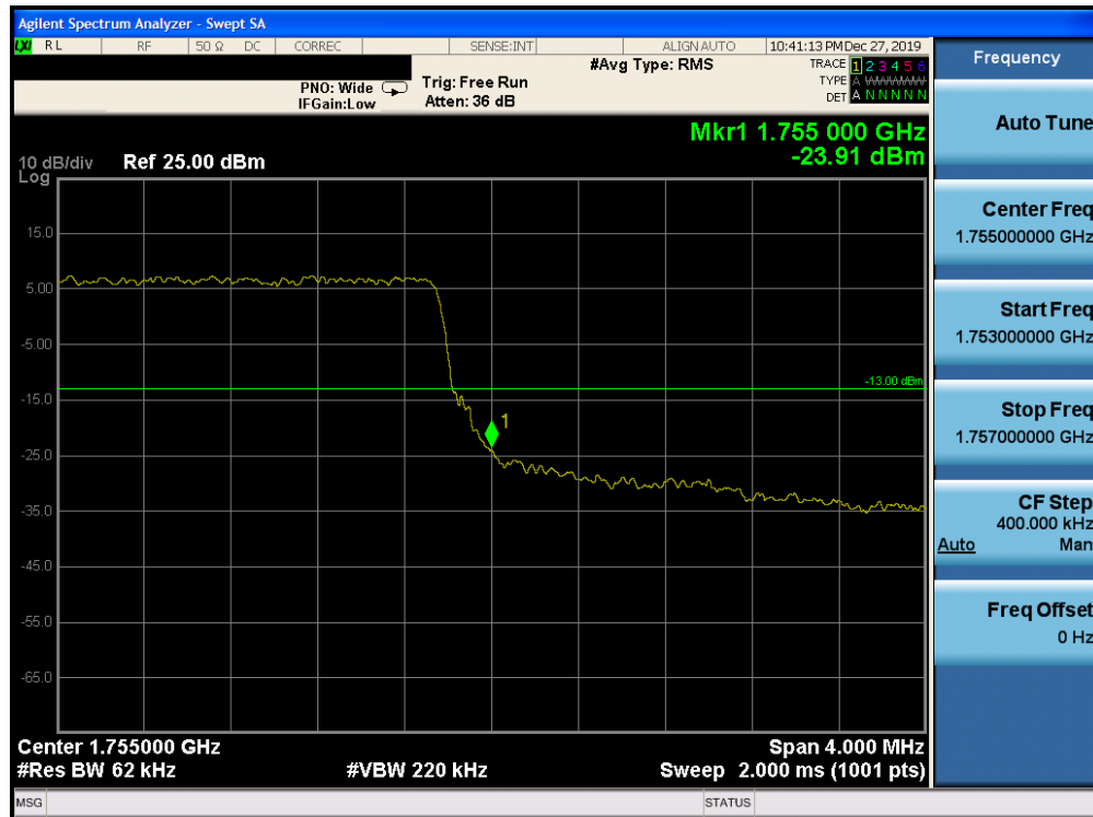
Plot 7-244. Upper Band Edge Plot (Band 4 – 5.0MHz QPSK – RB Size 25)
