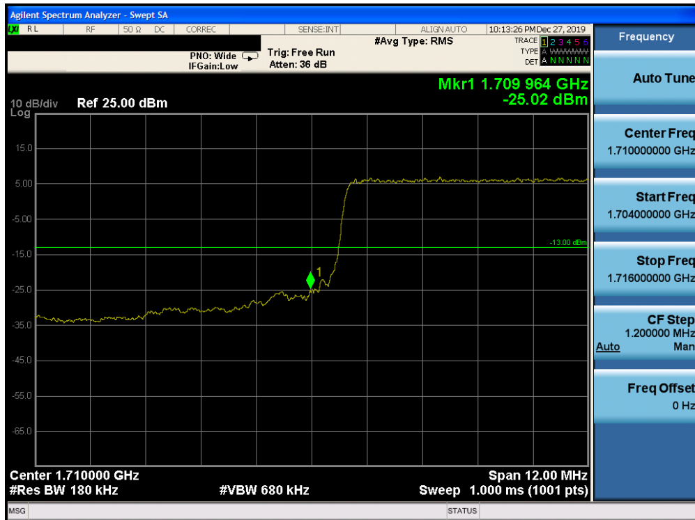
Plot 7-250. Lower Band Edge Plot (Band 4 – 15.0MHz QPSK – RB Size 75)
