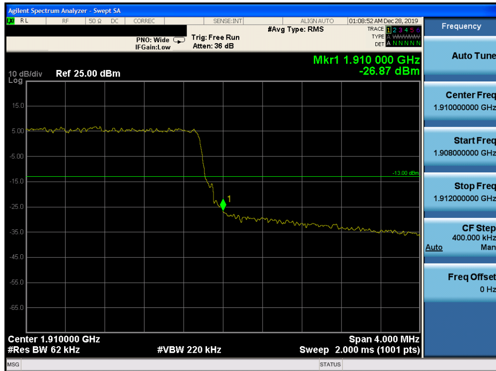
Plot 7-292. Upper Band Edge Plot (Band 2 - 5.0MHz QPSK - RB Size 25)
