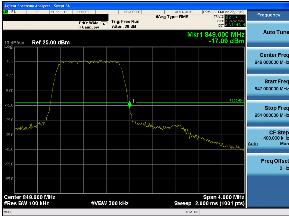
Plot 7-227. Upper Band Edge Plot (Band 5 – 1.4MHz QPSK – RB Size 6)
