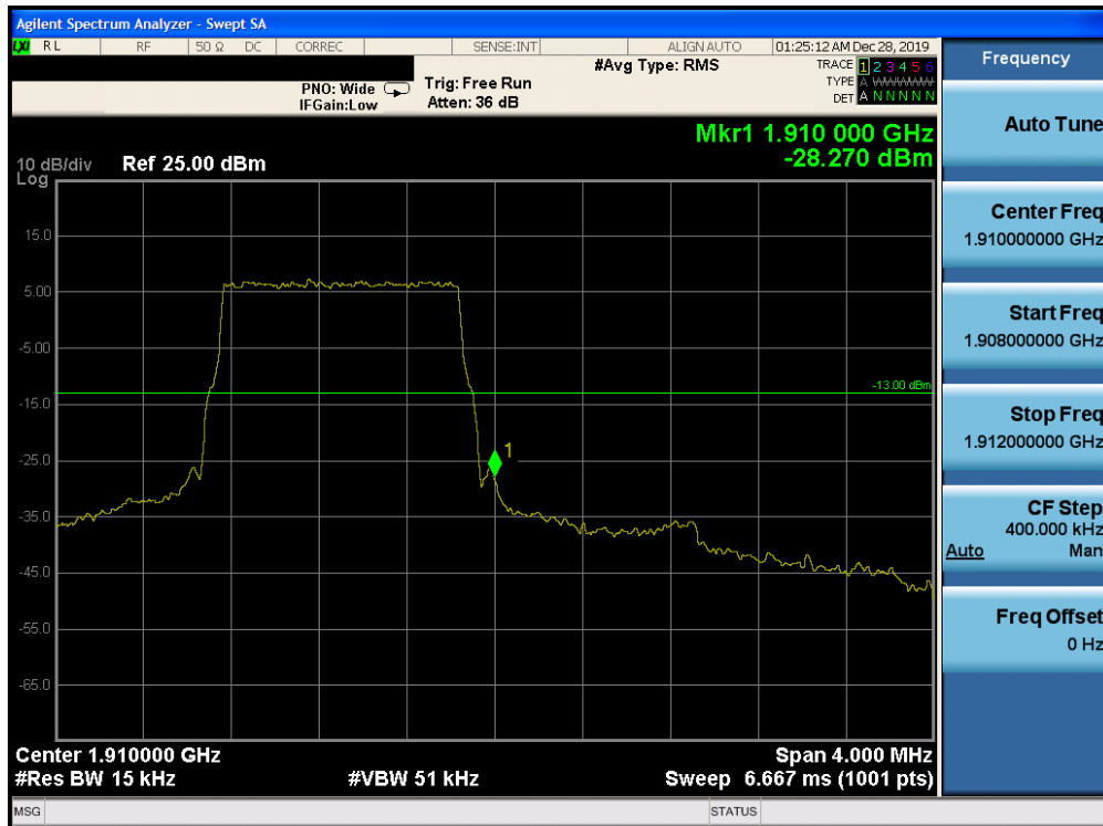
Plot 7-284. Upper Band Edge Plot (Band 2 – 1.4MHz QPSK – RB Size 6)
