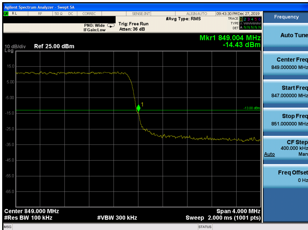
Plot 7-229. Upper Band Edge Plot (Band 5 - 3.0MHz QPSK - RB Size 15)
