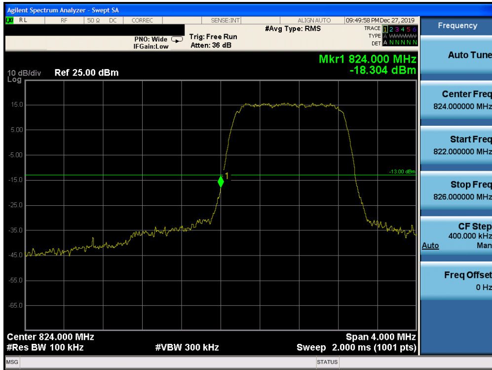
Plot 7-226. Lower Band Edge Plot (Band 5 – 1.4MHz QPSK – RB Size 6)
