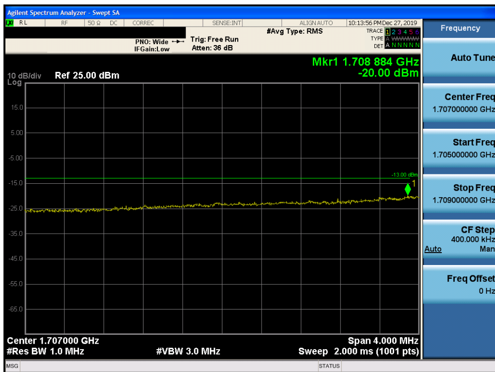
Plot 7-251. Lower Extended Band Edge Plot (Band 4 – 15.0MHz QPSK – RB Size 75)
