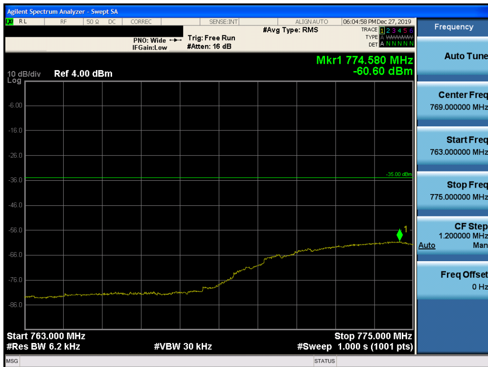
Plot 7-215. Lower Emission Mask Edge Plot (Band 13 – 10.0MHz QPSK – RB Size 50)
