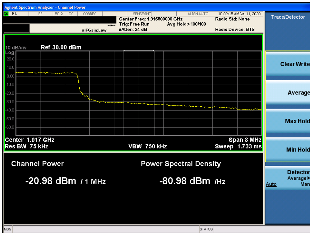
Plot 7-321. Upper Extended Band Edge Plot (Band 25 – 10.0MHz QPSK – RB Size 50)
