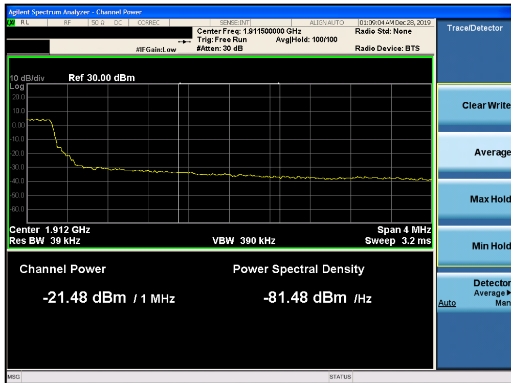
Plot 7-293. Upper Extended Band Edge Plot (Band 2 - 5.0MHz QPSK - RB Size 25)
