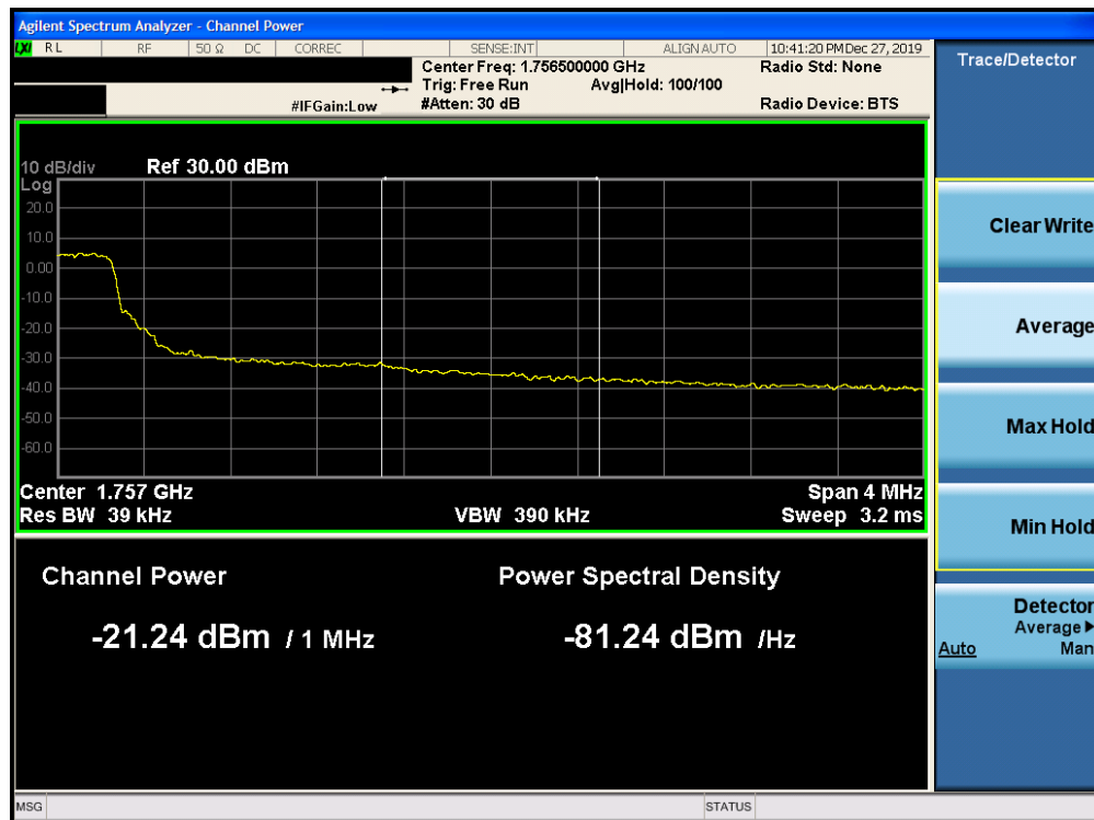
Plot 7-245. Upper Extended Band Edge Plot (Band 4 – 5.0MHz QPSK – RB Size 25)
