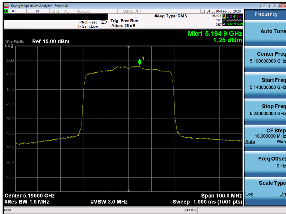
Plot 7-435. Power Spectral Density Plot ISSED SISO CORE 1 (40MHz BW 802.11ax – RU484 (UNII Band 1) – Ch. 38)
