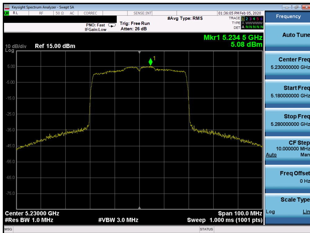
Plot 7-436. Power Spectral Density Plot ISSED SISO CORE 1 (40MHz BW 802.11ax – RU484 (UNII Band 1) – Ch. 46)
