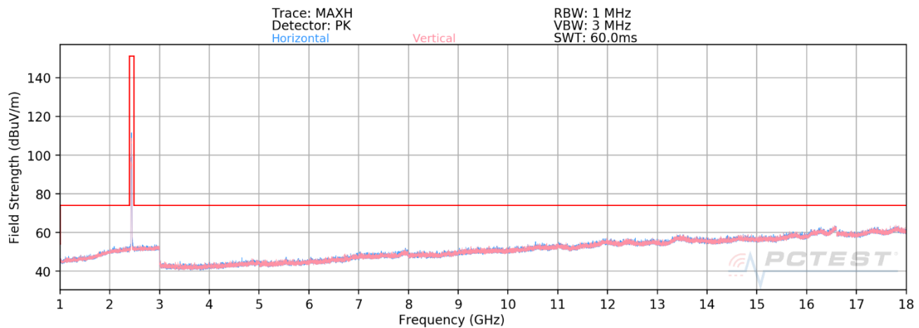
Plot 7-116. Radiated Spurious Plot above 1GHz SISO CORE 1 (802.11ax OFDMA – RU26 – Ch. 6)
