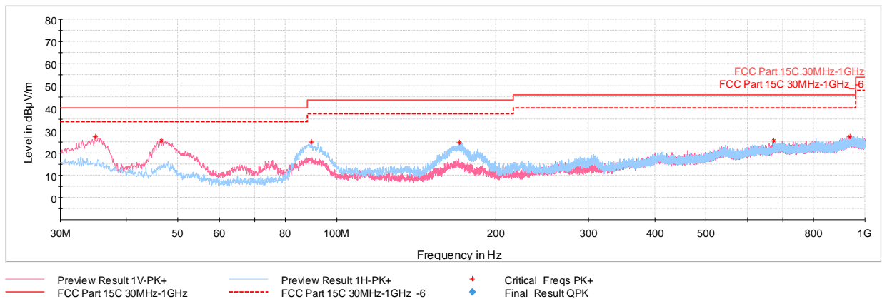
Plot 7-150. Radiated Spurious Plot below 1GHz CDD Ch.6 (RU242), with AC/DC Adapter
