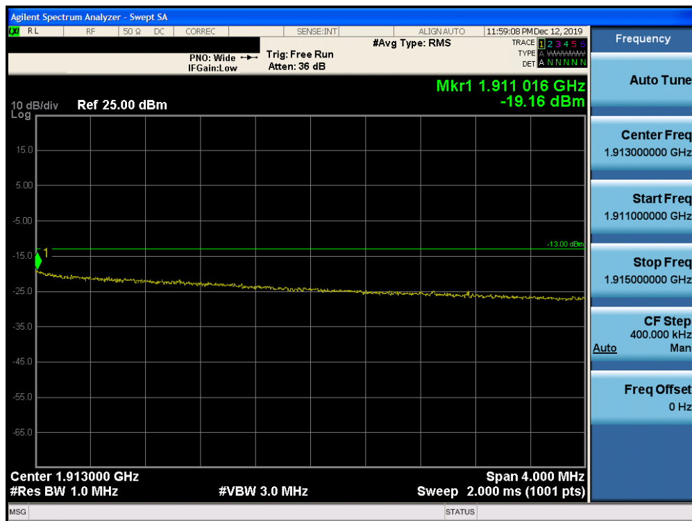
Plot 7-297. Upper Extended Band Edge Plot (Band 2 – 10.0MHz QPSK – RB Size 50)
