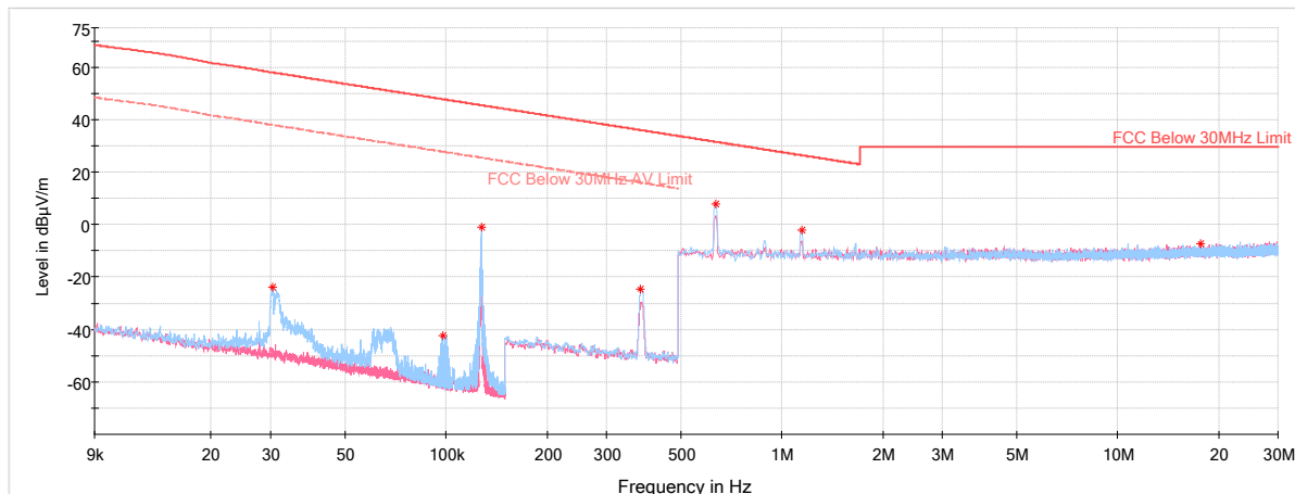
Plot 6-3. Radiated Spurious Plot 9kHz-30MHz with AC/DC Adapter
