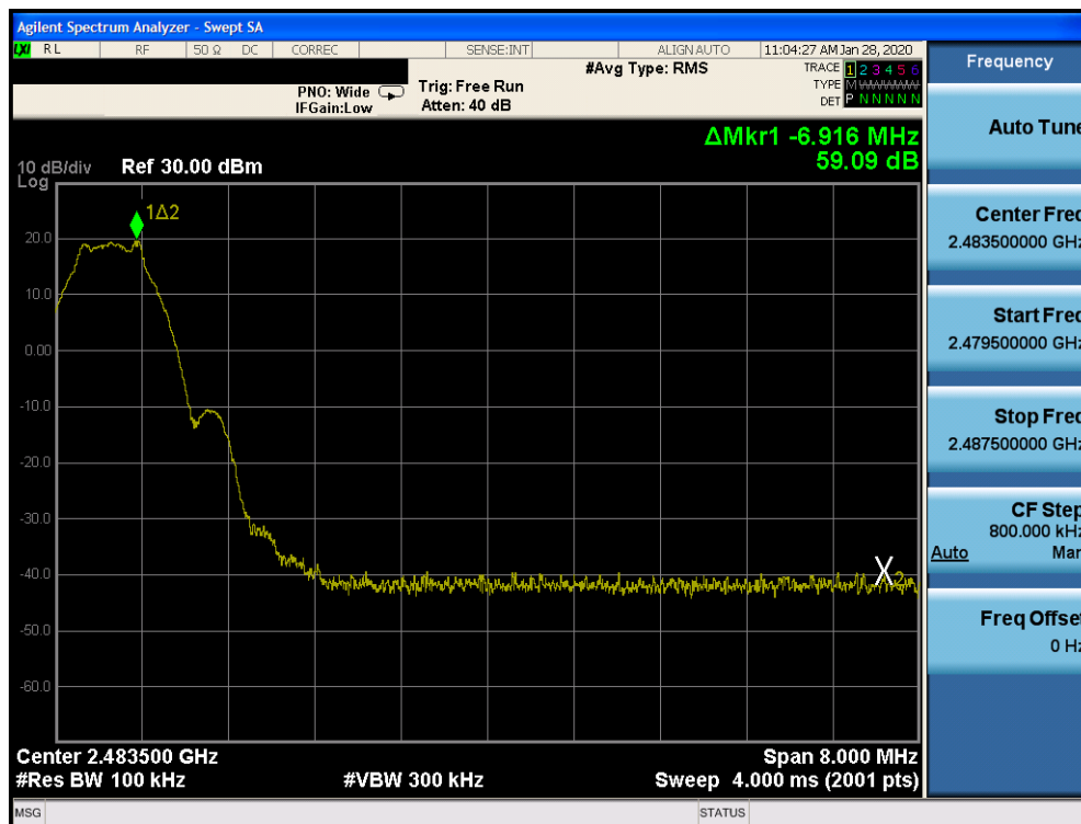
Plot 7-62. Band Edge Plot Ant 4a (Bluetooth (LE), 1Mbps ePA – Ch. 39)
