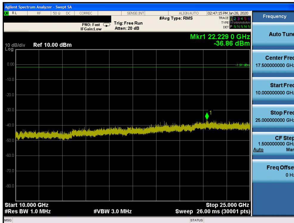
Plot 7-76. Conducted Spurious Plot Ant 2a (Bluetooth (LE), 1Mbps, ePA - Ch. 0)
