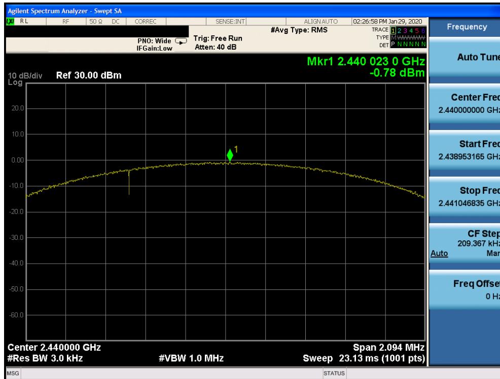
Plot 7-51. Power Spectral Density Plot TxBF Ant 4a (Bluetooth (LE), 2Mbps, ePA – Ch. 19)
