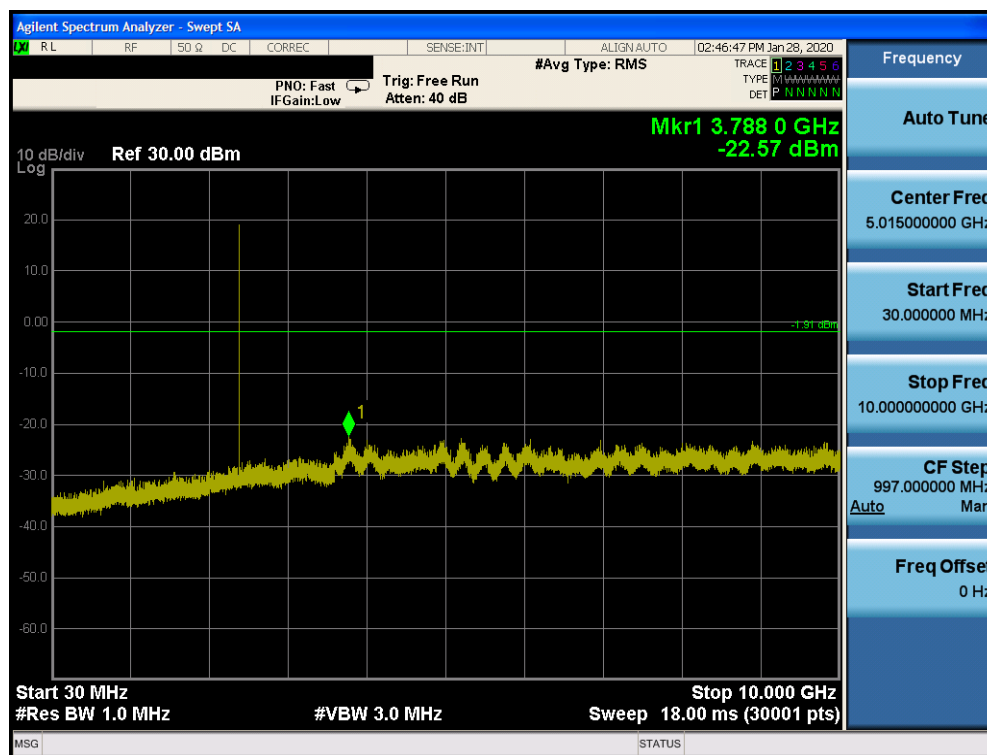
Plot 7-75. Conducted Spurious Plot Ant 2a (Bluetooth (LE), 1Mbps, ePA - Ch. 0)
