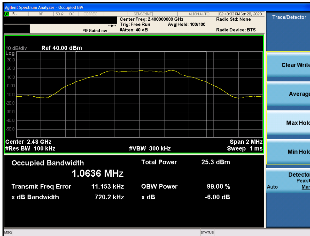
Plot 7-9. 6dB Bandwidth Plot Ant 2a (Bluetooth (LE), 1Mbps, ePA - Ch. 39)
