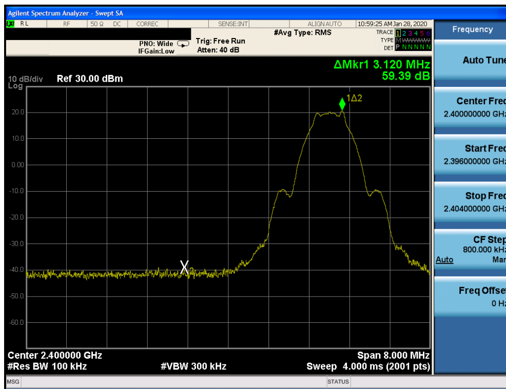
Plot 7-61. Band Edge Plot Ant 4a (Bluetooth (LE), 1Mbps ePA – Ch. 0)
