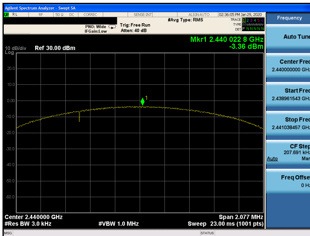
Plot 7-52. Power Spectral Density Plot TxBF Ant 2a (Bluetooth (LE), 2Mbps, ePA – Ch. 19)
