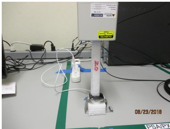
CENTER, RF EXPOSURE SETUP PHOTO (HORIZONTAL) 20cm
