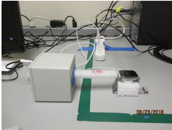
S4, RF EXPOSURE SETUP PHOTO (HORIZONTAL) 15cm
