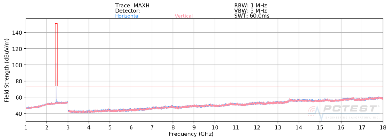
Plot 7-33. Radiated Spurious Plot Above 1GHz (Bluetooth (LE), 2Mbps – Ch. 19, Ant. Pol. H & V)
