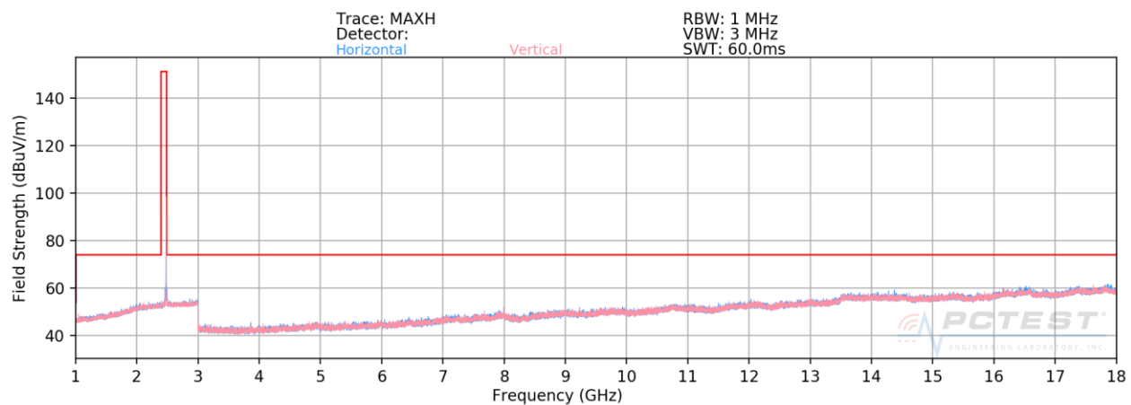
Plot 7-34. Radiated Spurious Plot Above 1GHz (Bluetooth (LE), 2Mbps – Ch. 39, Ant. Pol. H & V)
