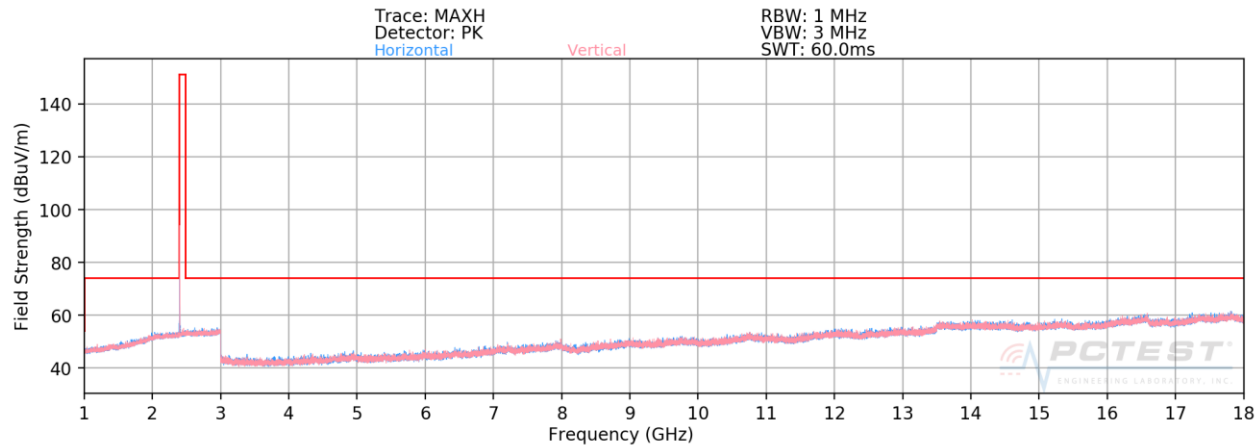
Plot 7-29. Radiated Spurious Plot Above 1GHz (Bluetooth (LE), 1Mbps – Ch. 0, Ant. Pol. H & V)
