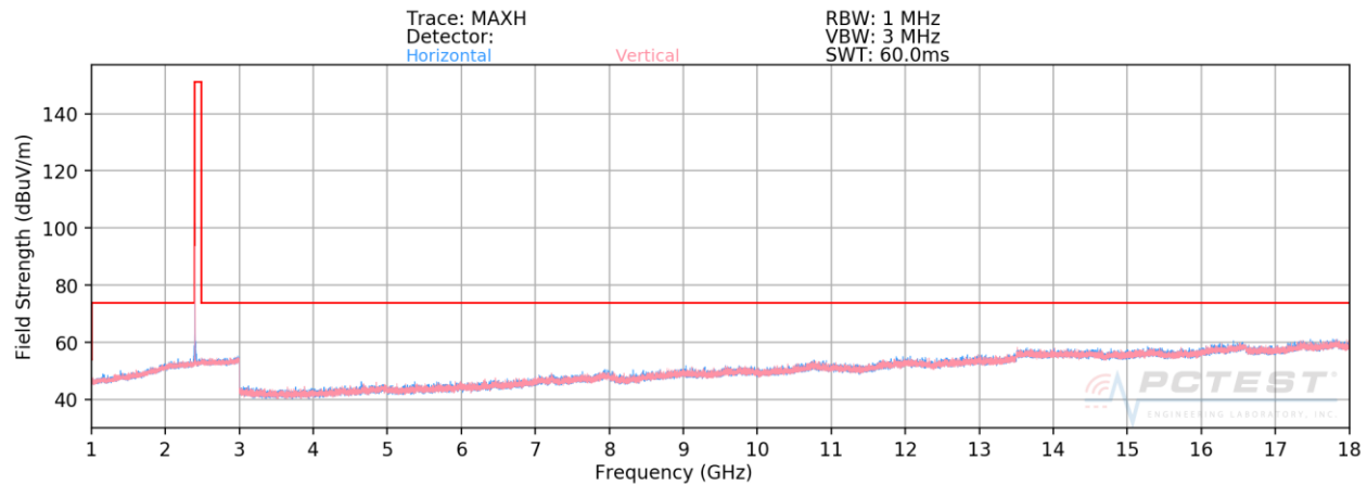
Plot 7-32. Radiated Spurious Plot Above 1GHz (Bluetooth (LE), 2Mbps – Ch. 0, Ant. Pol. H & V)
