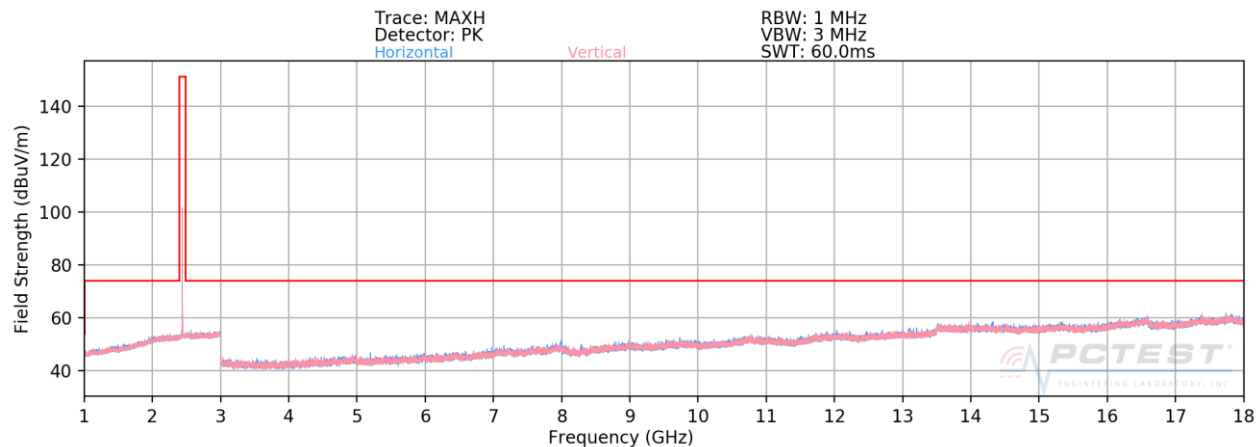
Plot 7-30. Radiated Spurious Plot Above 1GHz (Bluetooth (LE), 1Mbps – Ch. 19, Ant. Pol. H & V)
