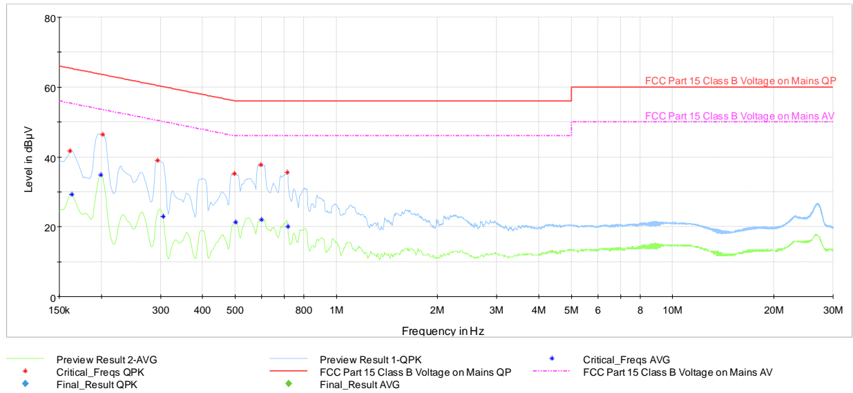
Plot 7-48. Line Conducted Plot with Bluetooth LE 1Mbps, Ch. 19 (L1, with AC/DC Adapter)
