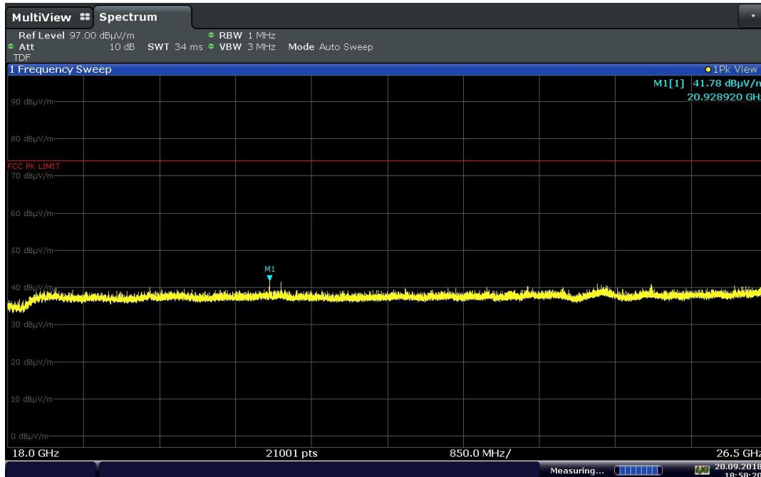
Plot 7-36. Radiated Spurious Plot Above 18GHz (Bluetooth (LE), 1Mbps, Ch. 19, Ant. Pol. V)
