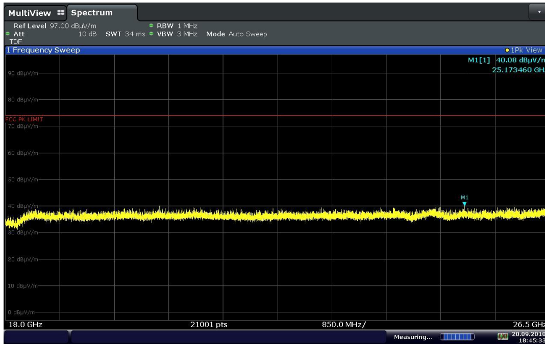
Plot 7-35. Radiated Spurious Plot Above 18GHz (Bluetooth (LE), 1Mbps, Ch. 19, Ant. Pol. H)
