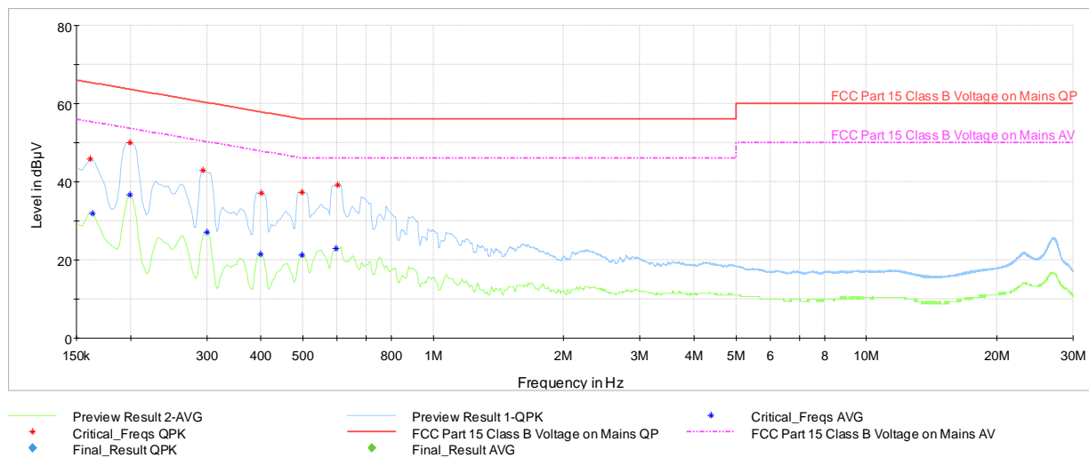
Plot 7-49. Line Conducted Plot with Bluetooth LE 1Mbps, Ch. 19 (N, with AC/DC Adapter)
