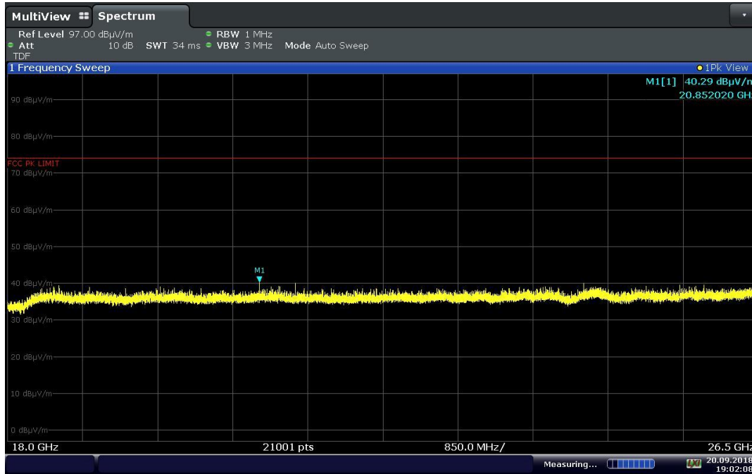
Plot 7-37. Radiated Spurious Plot Above 18GHz (Bluetooth (LE), 2Mbps, Ch. 19, Ant. Pol. H)
