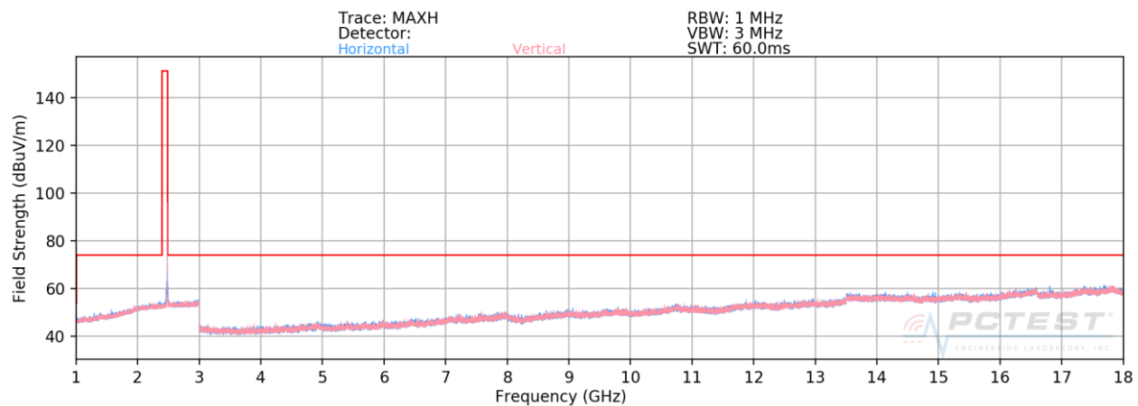
Plot 7-31. Radiated Spurious Plot Above 1GHz (Bluetooth (LE), 1Mbps – Ch. 39, Ant. Pol. H & V)
