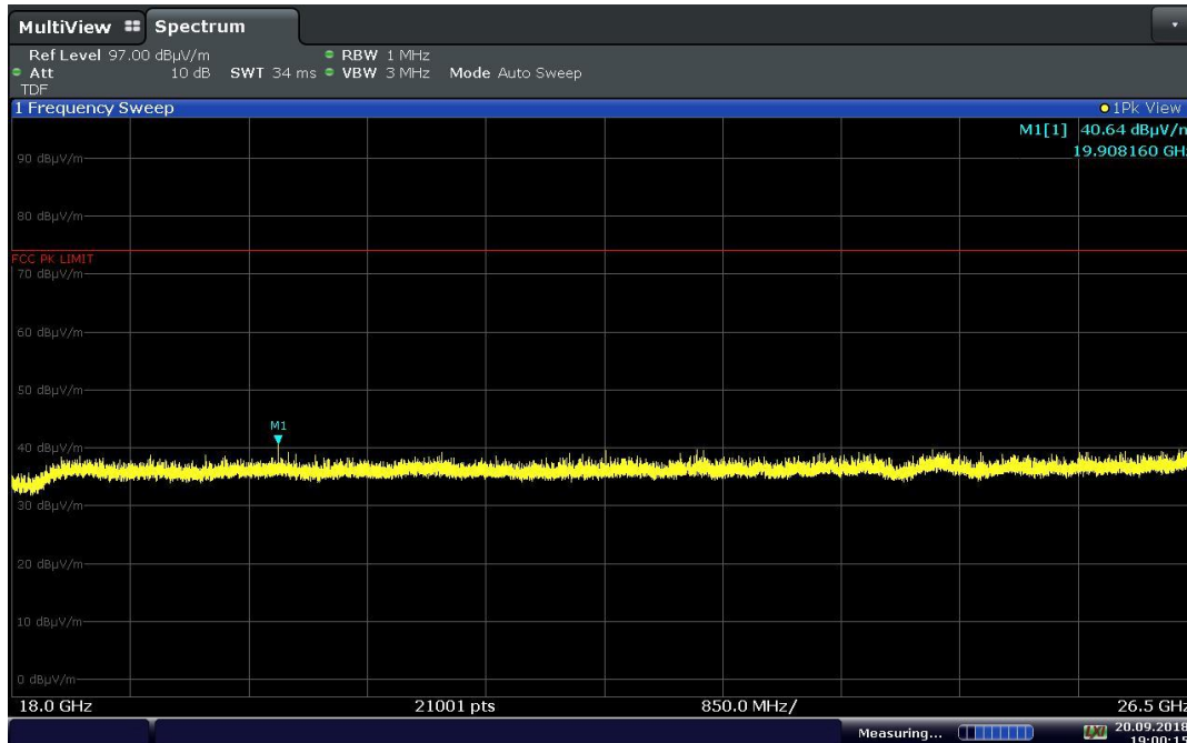
Plot 7-38. Radiated Spurious Plot Above 18GHz (Bluetooth (LE), 2Mbps, Ch. 19, Ant. Pol. V)
