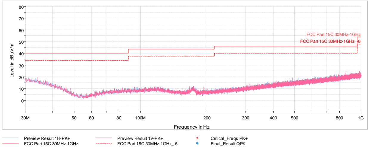
Plot 7-47. Radiated Spurious Plot Below 1GHz (1Mbps, Ch. 19, Ant. Pol. H & V, with AC/DC Adapter)
