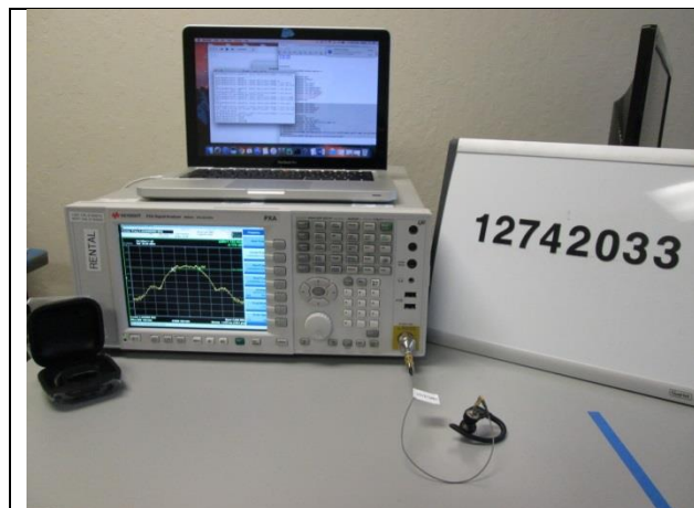
RF CONDUCTED
