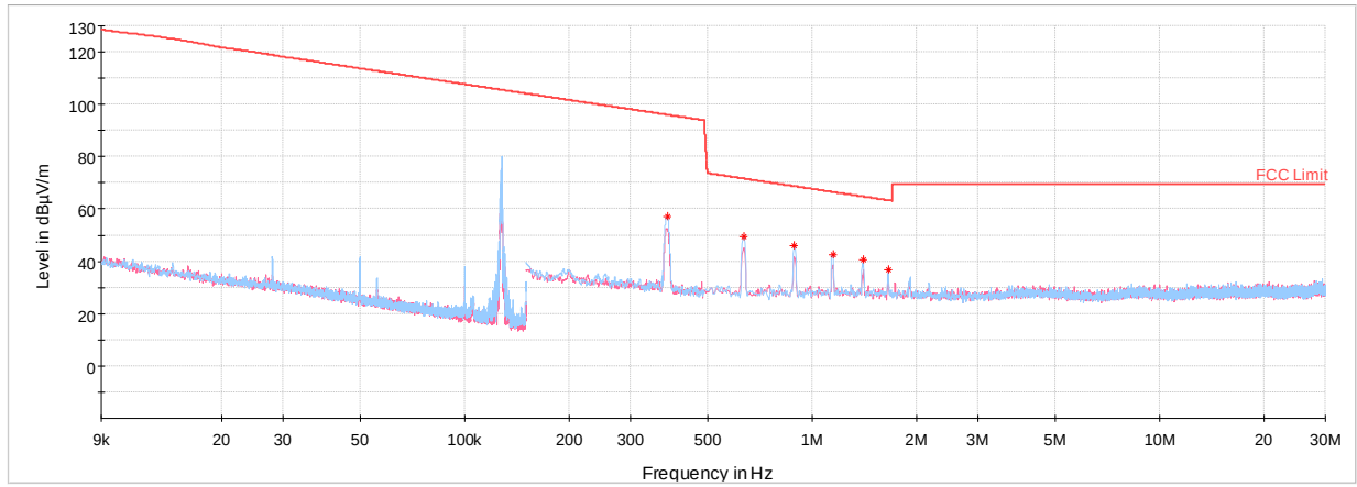
Plot 7-3. Radiated Spurious Plot from 9kHz – 30MHz (Loop Antenna X & Y)
