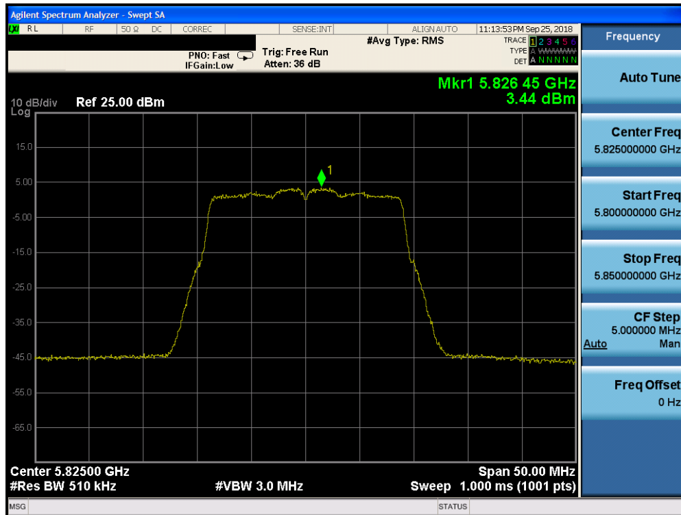
Plot 7-159. Power Spectral Density Plot CDD CORE 0 (20MHz BW 802.11n (UNII Band 3) – Ch. 165)
