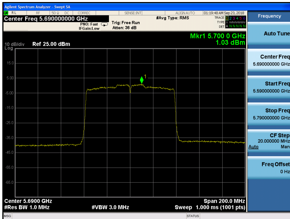
Plot 7-154. Power Spectral Density Plot CDD CORE 1 (80MHz BW 802.11ac (UNII Band 2C) – Ch. 138)
