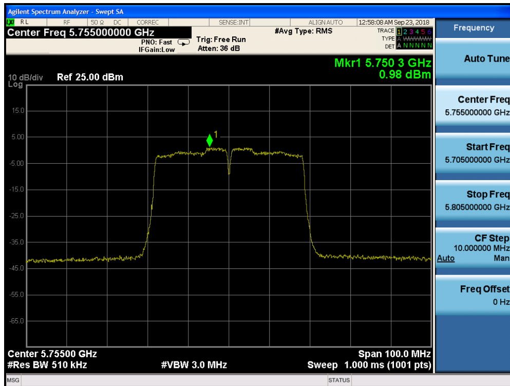
Plot 7-162. Power Spectral Density Plot CDD CORE 1 (40MHz BW 802.11n (UNII Band 3) – Ch. 151)
