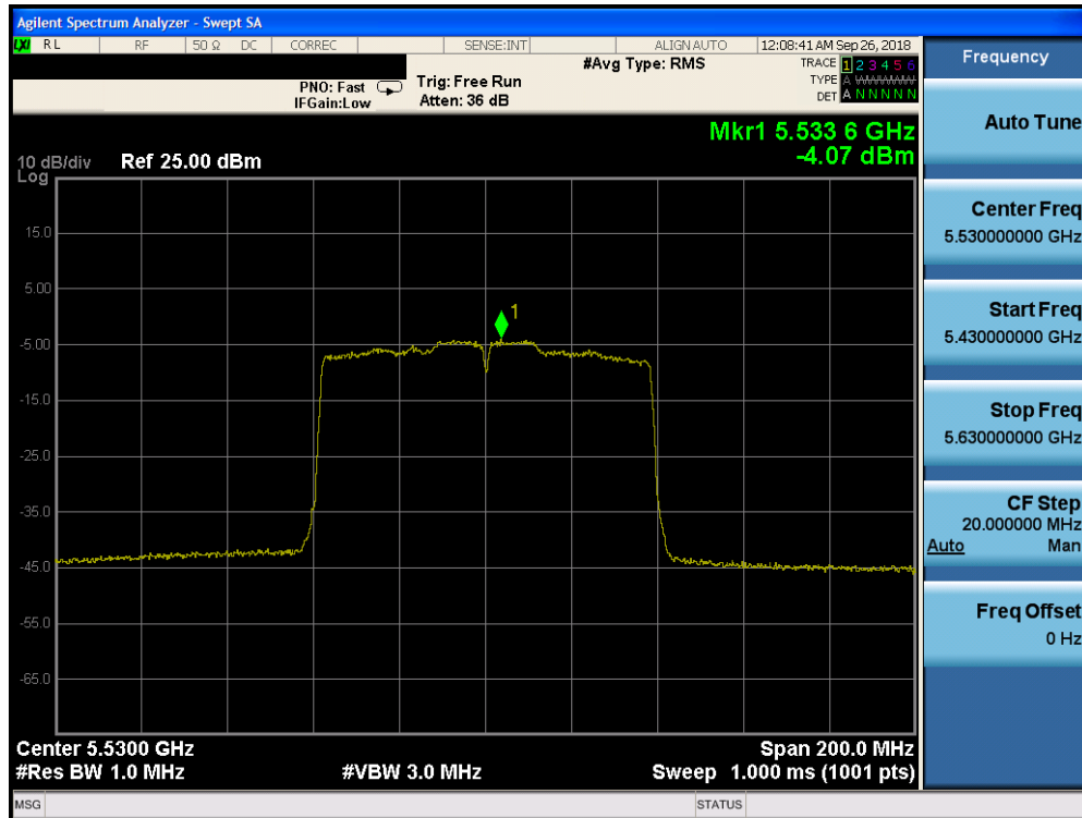
Plot 7-151. Power Spectral Density Plot CDD CORE 0 (80MHz BW 802.11ac (UNII Band 2C) – Ch. 106)
