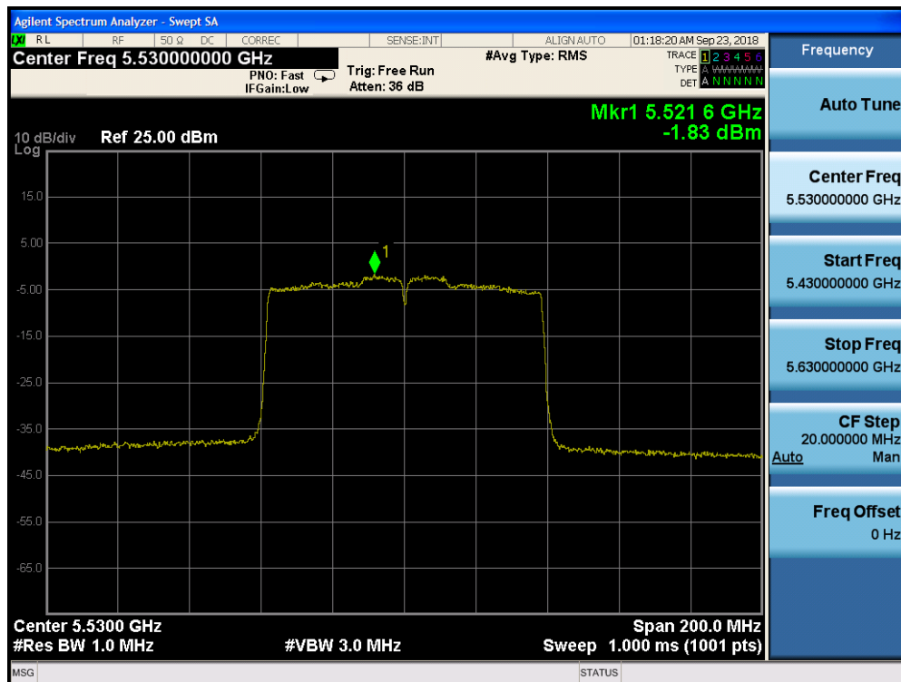
Plot 7-152. Power Spectral Density Plot CDD CORE 1 (80MHz BW 802.11ac (UNII Band 2C) – Ch. 106)
