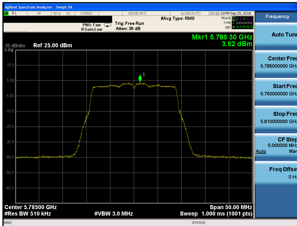
Plot 7-74. Power Spectral Density Plot SISO CORE0 (20MHz BW 802.11n (UNII Band 3) – Ch. 157)
