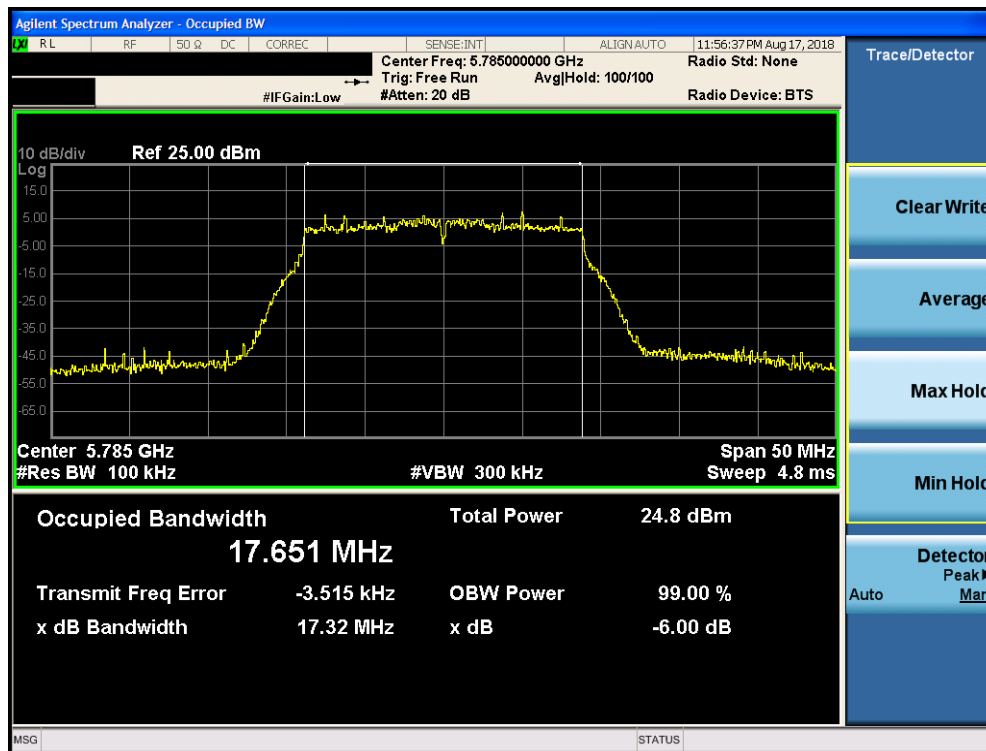
Plot 7-48. 6dB Bandwidth Plot SISO CORE1 (20MHz BW 802.11n (UNII Band 3) – Ch. 157)
