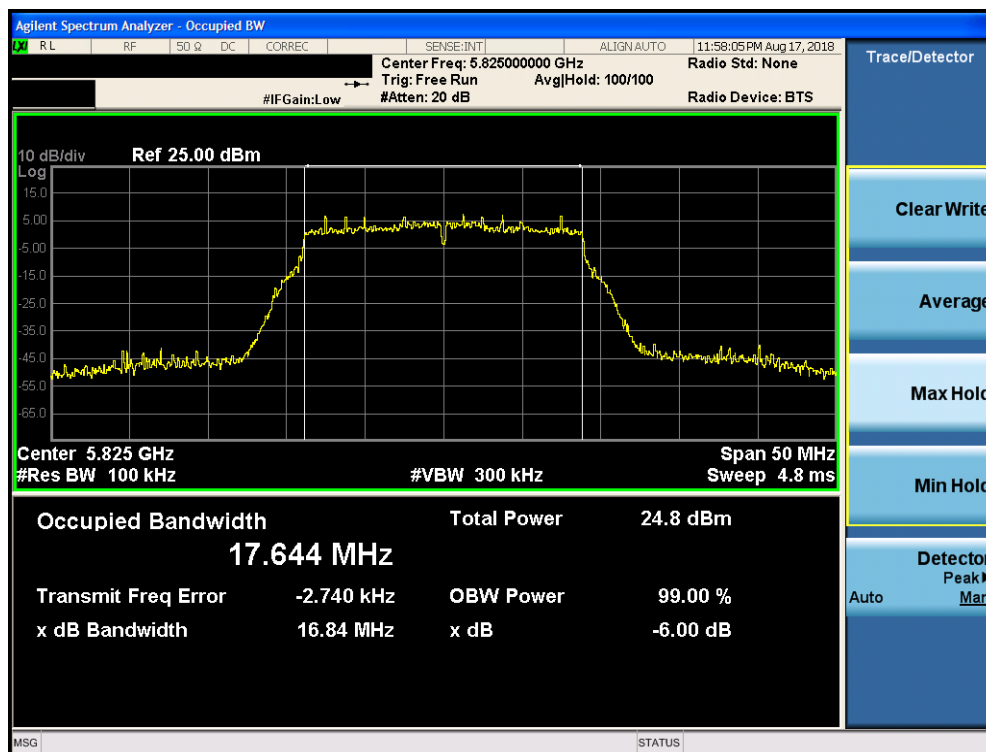
Plot 7-49. 6dB Bandwidth Plot SISO CORE1 (20MHz BW 802.11n (UNII Band 3) – Ch. 165)
