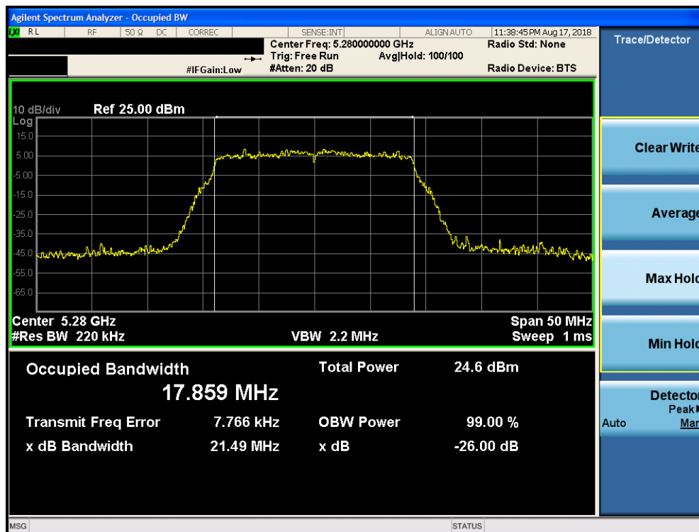
Plot 7-28. 26dB Bandwidth Plot SISO CORE1 (20MHz BW 802.11n (UNII Band 2A) – Ch. 56)
