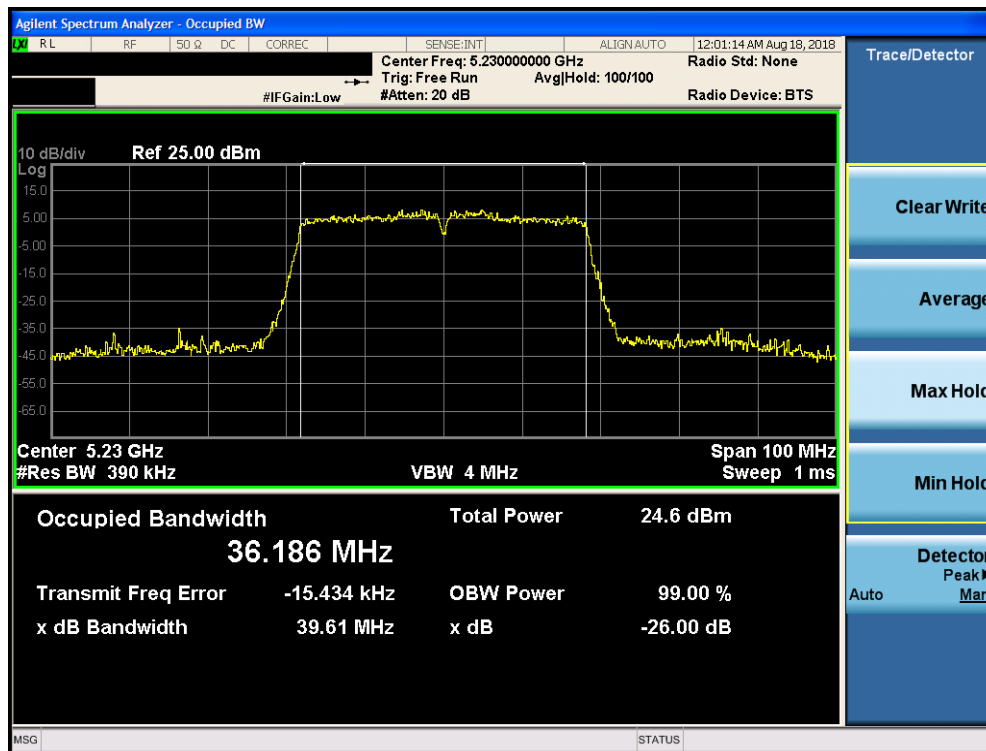
Plot 7-25. 26dB Bandwidth Plot SISO CORE1 (40MHz BW 802.11n (UNII Band 1) – Ch. 46)
