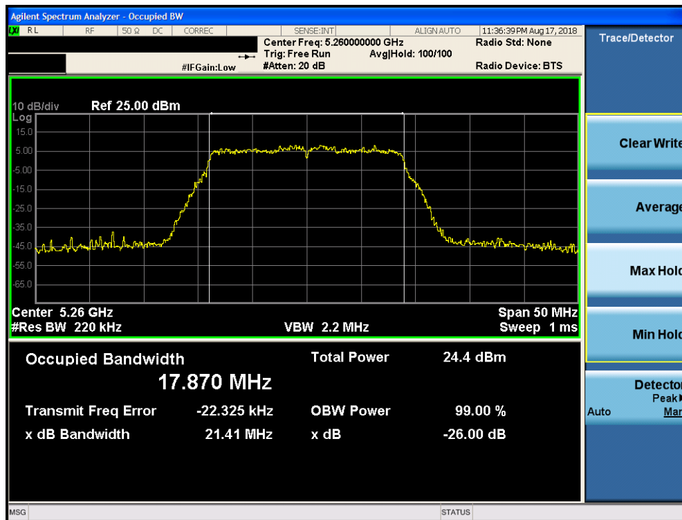
Plot 7-27. 26dB Bandwidth Plot SISO CORE1 (20MHz BW 802.11n (UNII Band 2A) – Ch. 52)
