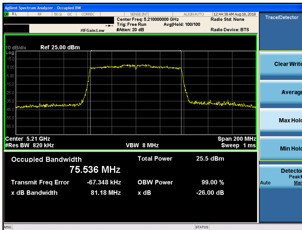
Plot 7-26. 26dB Bandwidth Plot SISO CORE1 (80MHz BW 802.11ac (UNII Band 1) – Ch. 42)
