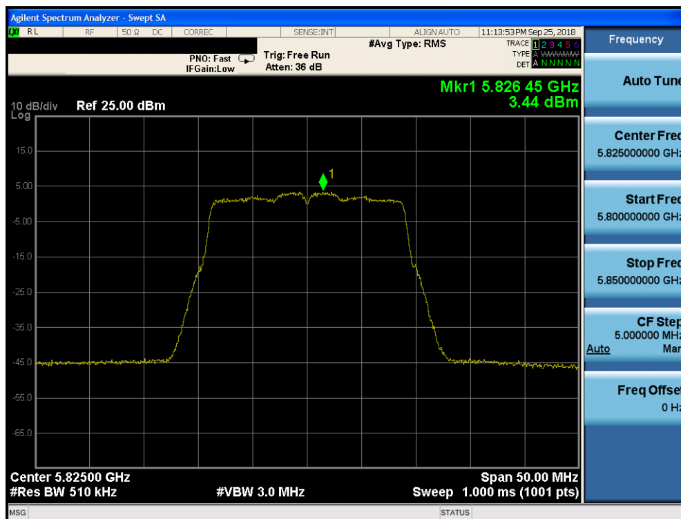
Plot 7-75. Power Spectral Density Plot SISO CORE0 (20MHz BW 802.11n (UNII Band 3) – Ch. 165)
