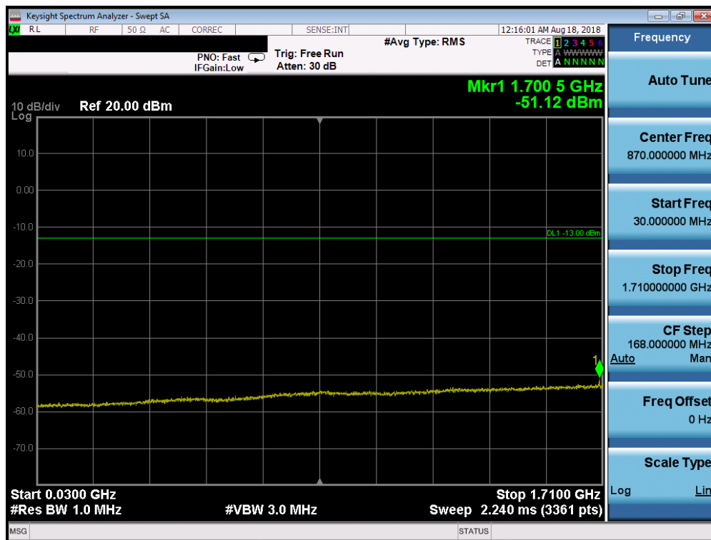
Plot 7-41. Conducted Spurious Plot (AWS WCDMA Mode - High Channel)
