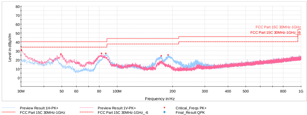
Plot 7-4. Radiated Spurious Plot above 30MHz (Pol. H & V)
