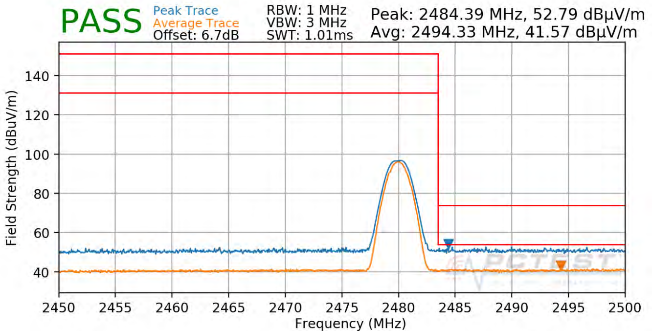
Plot 7-100. Radiated Restricted Upper Band Edge Measurement ANT2 (Average & Peak)
