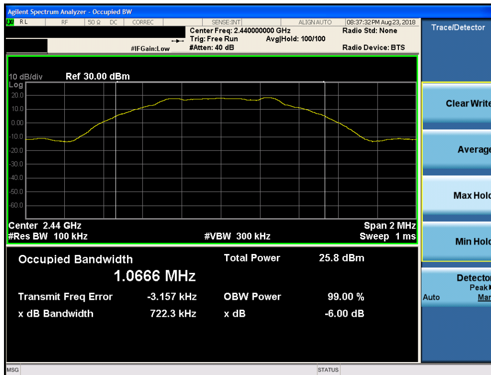
Plot 7-8. 6dB Bandwidth Plot ANT1 (Bluetooth (LE), 1Mbps, ePA – Ch. 19)
