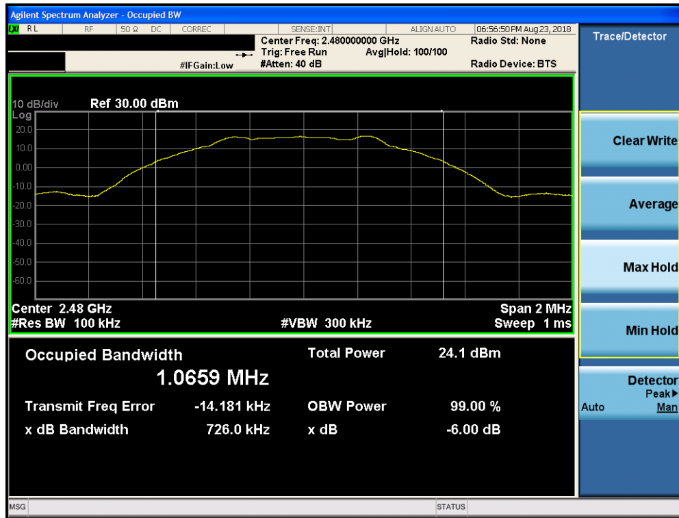
Plot 7-3. 6dB Bandwidth Plot ANT0 (Bluetooth (LE), 1Mbps, ePA – Ch. 39)
