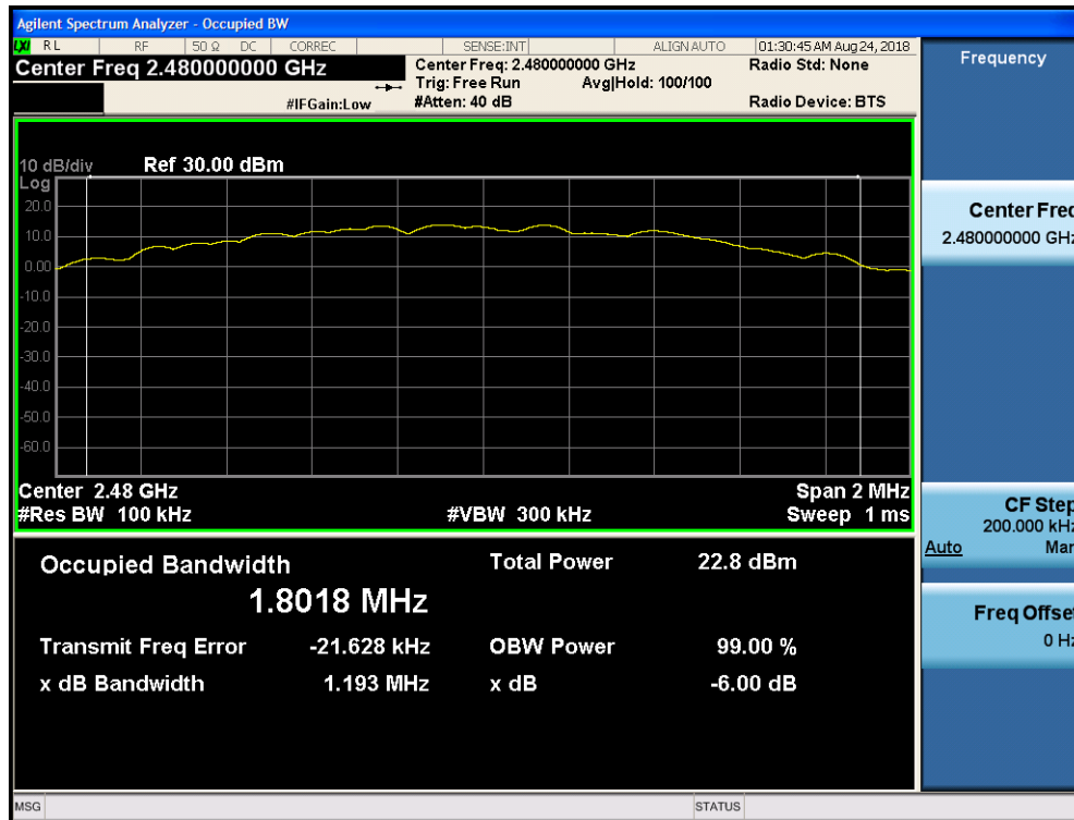
Plot 7-18. 6dB Bandwidth Plot ANT2 (Bluetooth (LE), 2Mbps, ePA – Ch. 39)
