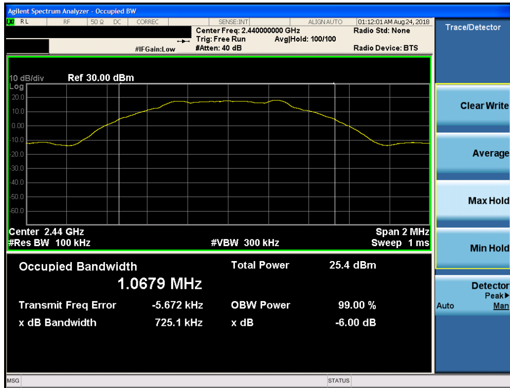
Plot 7-14. 6dB Bandwidth Plot ANT2 (Bluetooth (LE), 1Mbps, ePA – Ch. 19)
