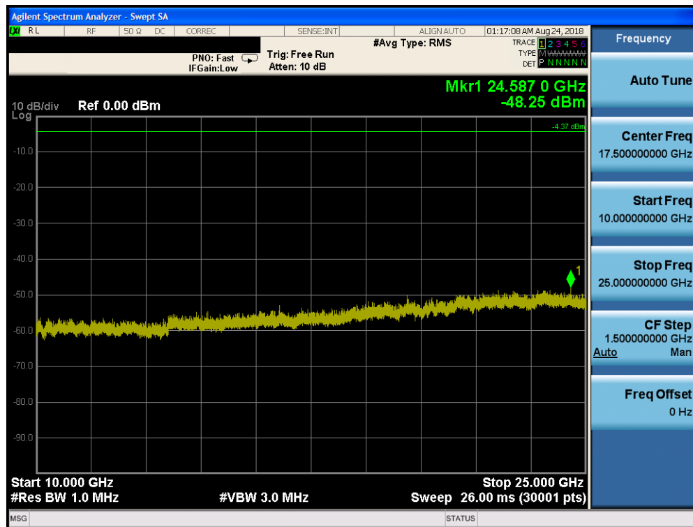
Plot 7-78. Conducted Spurious Plot ANT2 (Bluetooth (LE), 1Mbps, ePA – Ch. 39)
