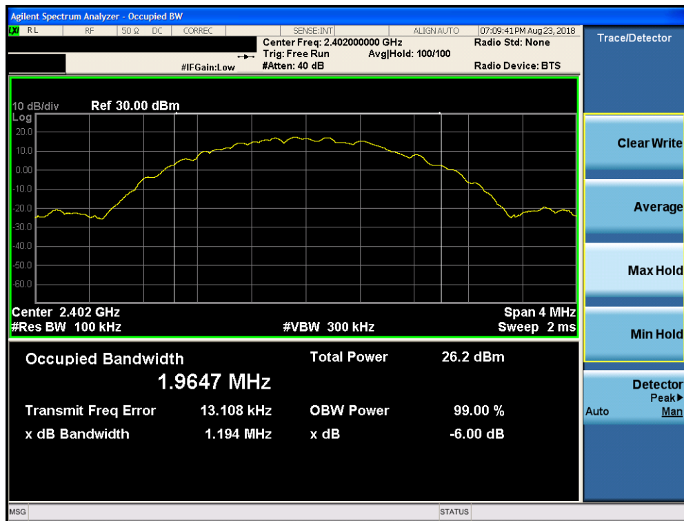
Plot 7-4. 6dB Bandwidth Plot ANT0 (Bluetooth (LE), 2Mbps, ePA – Ch. 0)
