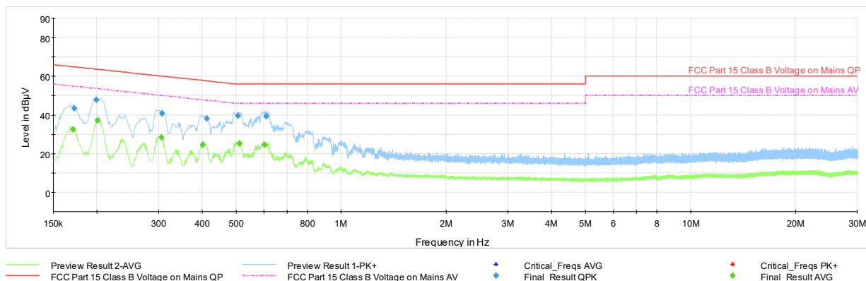
Plot 7-104. Line Conducted Plot with Bluetooth LE (N, with AC/DC Adapter)
