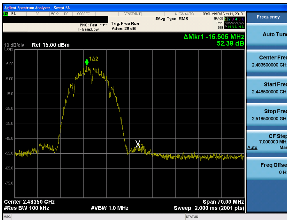
Plot 7-82. Band Edge Plot SISO Core 0 (802.11b – Ch. 13)
