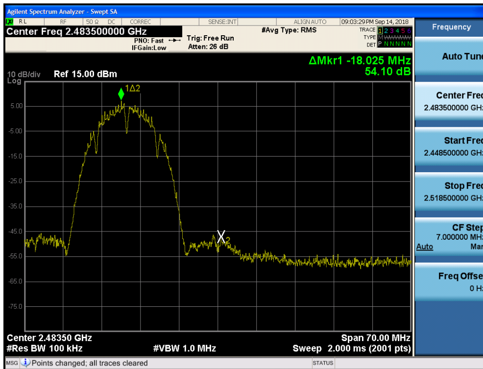
Plot 7-81. Band Edge Plot SISO Core 0 (802.11b – Ch. 12)
