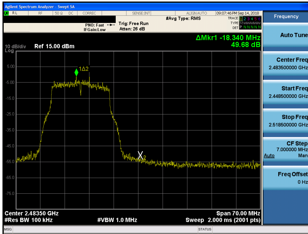
Plot 7-85. Band Edge Plot SISO Core 0 (802.11g – Ch. 12)
