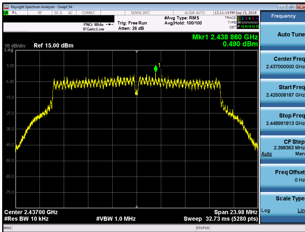
Plot 7-69. Power Spectral Density Plot CDD Core 0 (802.11g – Ch. 6)
