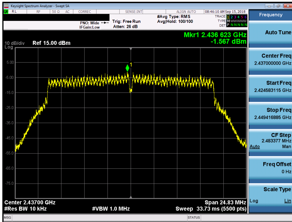
Plot 7-75. Power Spectral Density Plot CDD Core 0 (802.11n – Ch. 6)
