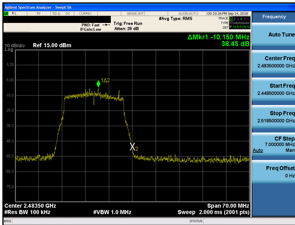
Plot 7-90. Band Edge Plot SISO Core 0 (11n) (2.4GHz) – Ch. 13)
