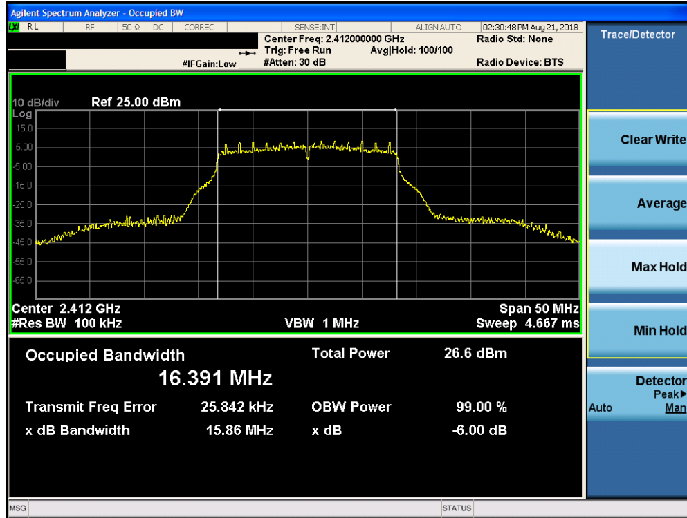
Plot 7-13. 6dB Bandwidth Plot Core 1 Primary (802.11g – Ch. 1)
