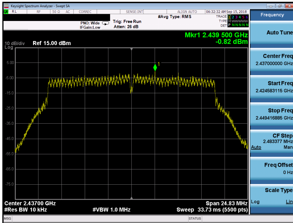
Plot 7-63. Power Spectral Density Plot CDD Core 0 (802.11n – Ch. 6)
