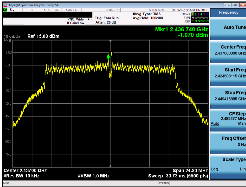
Plot 7-57. Power Spectral Density Plot CDD Core 0 (802.11g – Ch. 6)
