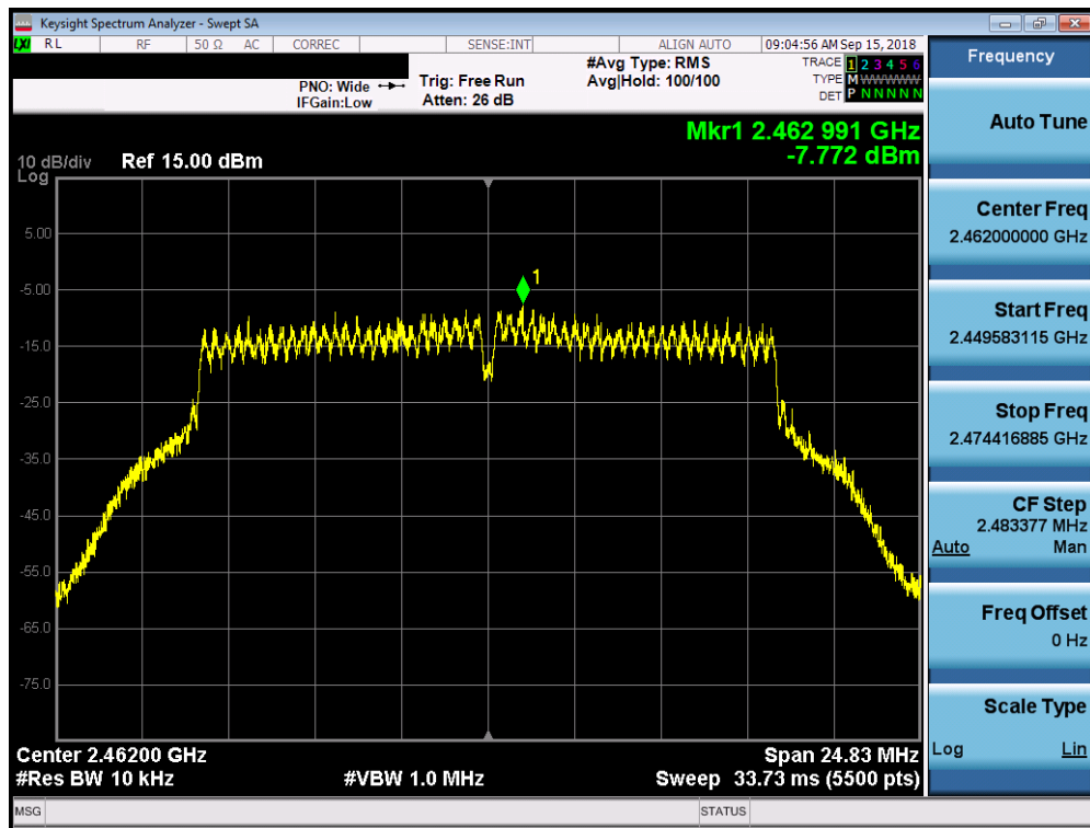
Plot 7-59. Power Spectral Density Plot CDD Core 0 (802.11g – Ch. 11)
