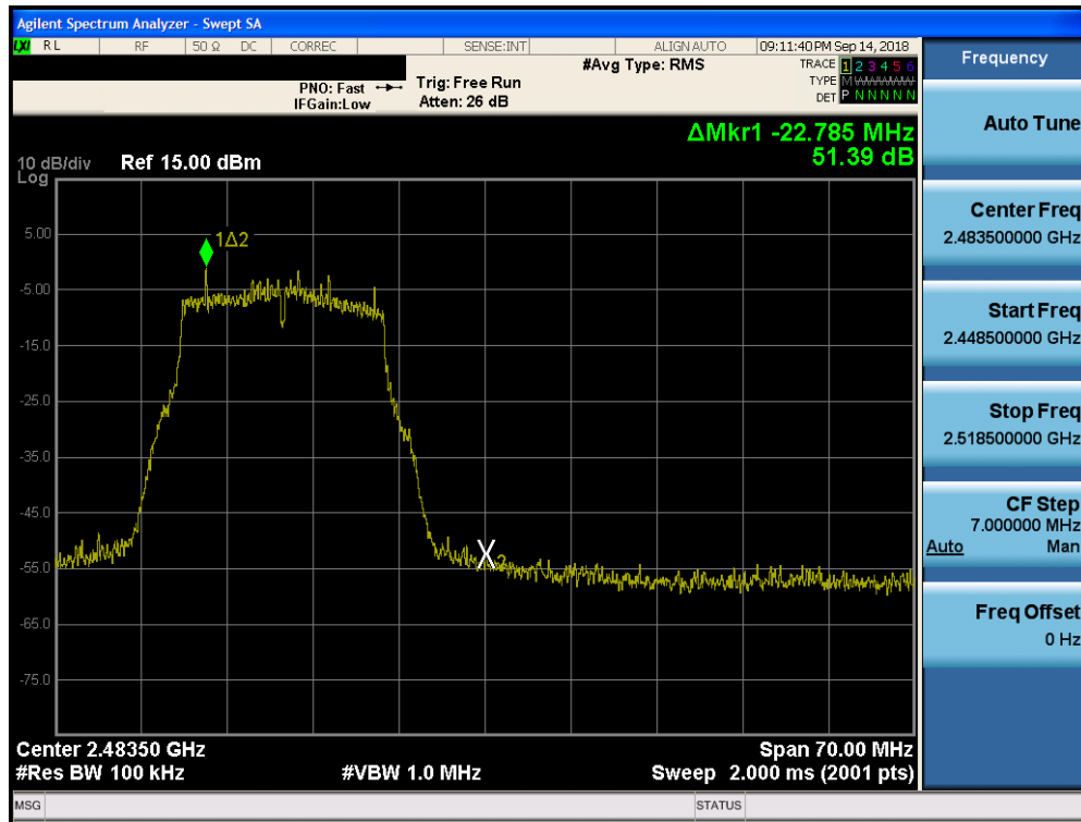
Plot 7-89. Band Edge Plot SISO Core 0 (11n) (2.4GHz) – Ch. 12)
