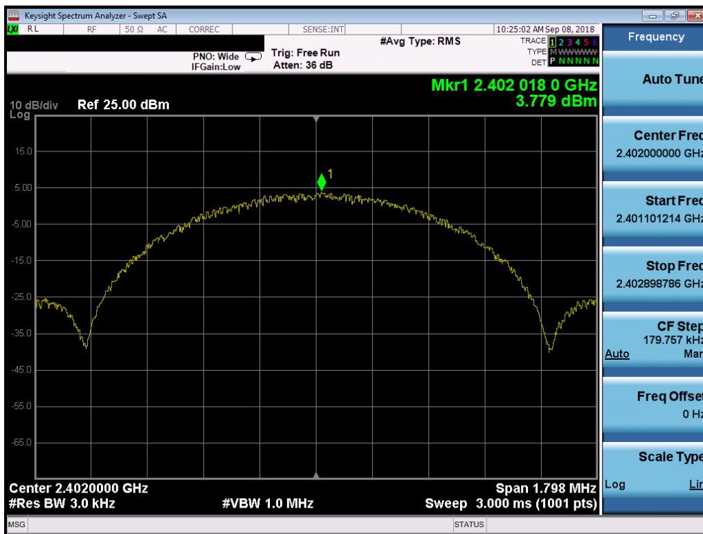
Plot 7-19. Power Spectral Density Plot (Bluetooth (LE), 1Mbps, ePA – Ch. 0, Antenna 0)
