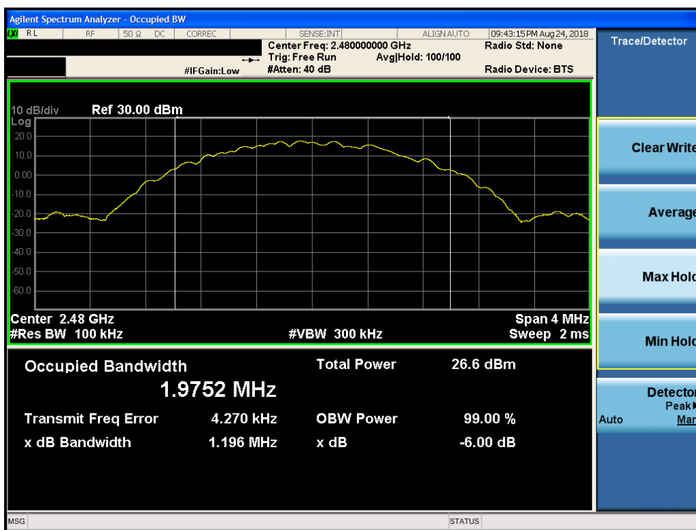
Plot 7-6. 6dB Bandwidth Plot (Bluetooth (LE), 2Mbps, ePA – Ch. 39, Antenna 0)
