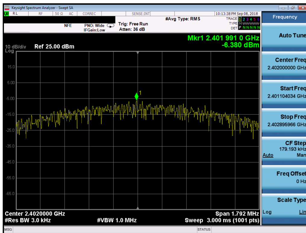
Plot 7-52. Power Spectral Density Plot (Bluetooth (LE), 2Mbps, iPA – Ch. 0, Antenna 2)
