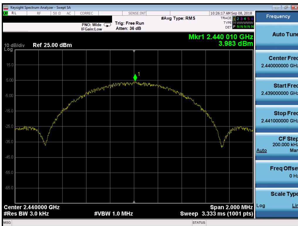
Plot 7-20. Power Spectral Density Plot (Bluetooth (LE), 1Mbps, ePA – Ch. 19, Antenna 0)
