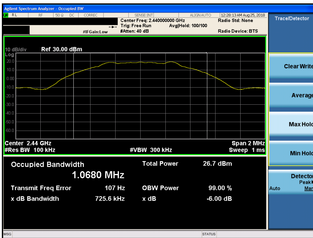
Plot 7-8. 6dB Bandwidth Plot (Bluetooth (LE), 1Mbps, ePA – Ch. 19, Antenna 1)
