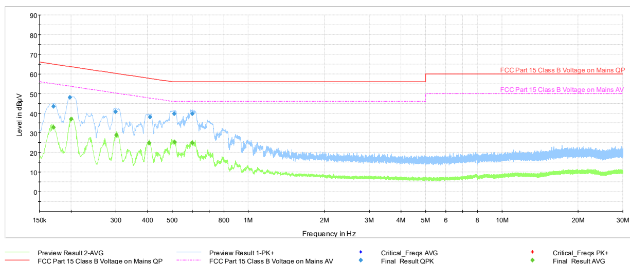
Plot 7-102. Line Conducted Plot with Bluetooth LE (GFSK ePA, N, with AC/DC Adapter)
