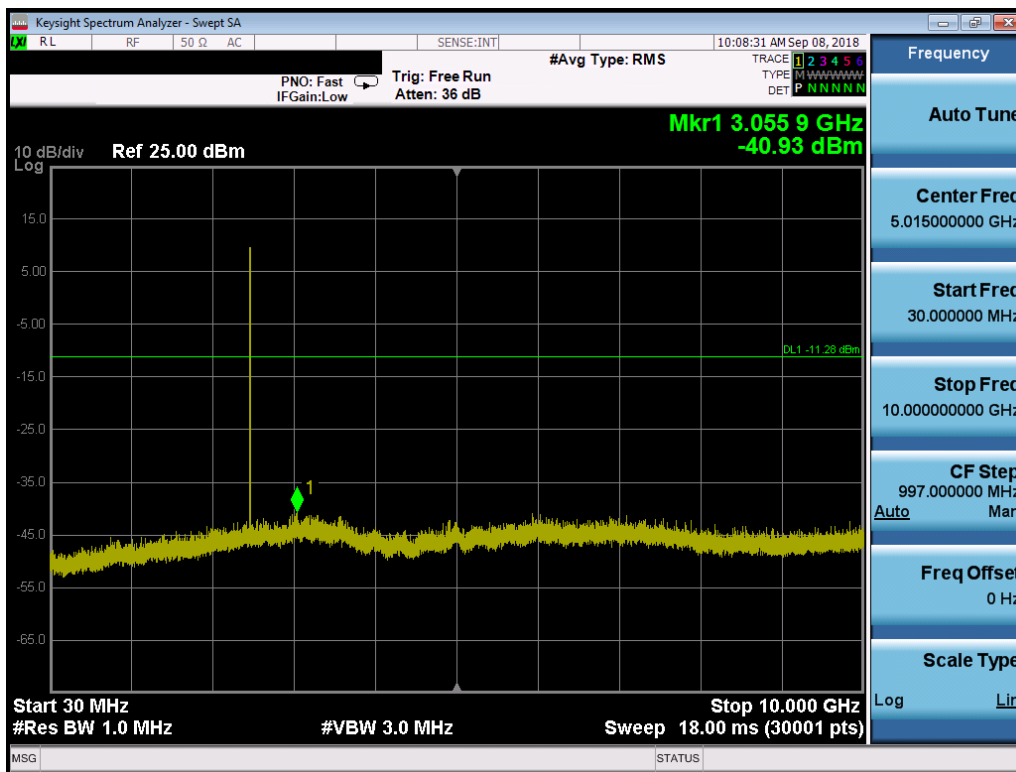
Plot 7-65. Conducted Spurious Plot (Bluetooth (LE), 1Mbps, ePA – Ch. 39, Antenna 0)
