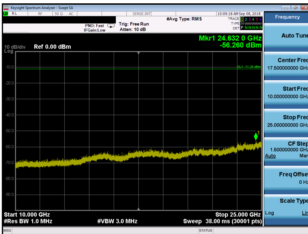
Plot 7-66. Conducted Spurious Plot (Bluetooth (LE), 1Mbps, ePA – Ch. 39, Antenna 0)
