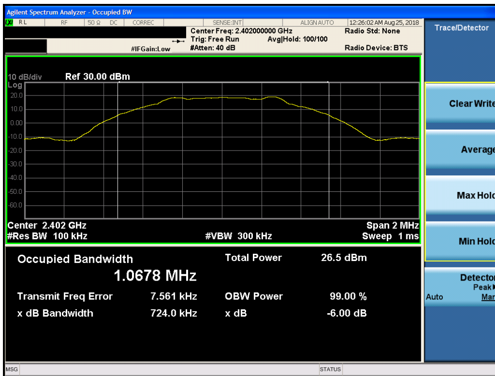
Plot 7-7. 6dB Bandwidth Plot (Bluetooth (LE), 1Mbps, ePA – Ch. 0, Antenna 1)
