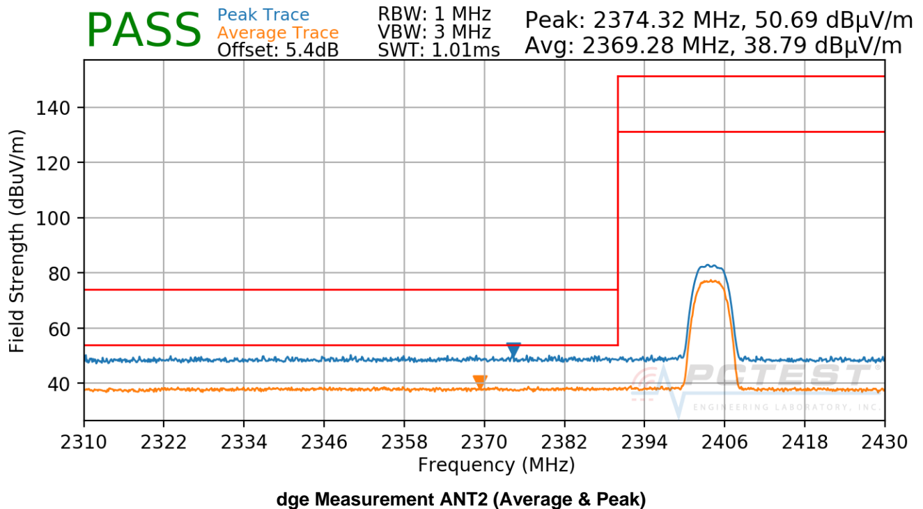
Plot 7-114. Radiated Restricted Lower Band E
