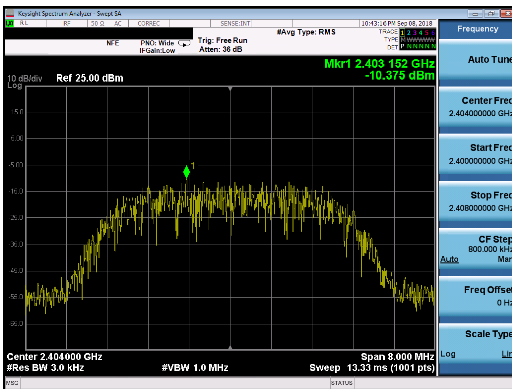
Plot 7-52. Power Spectral Density Plot ANT2 (Bluetooth (HDR8), 8Mbps, iPA – Ch. 1)
