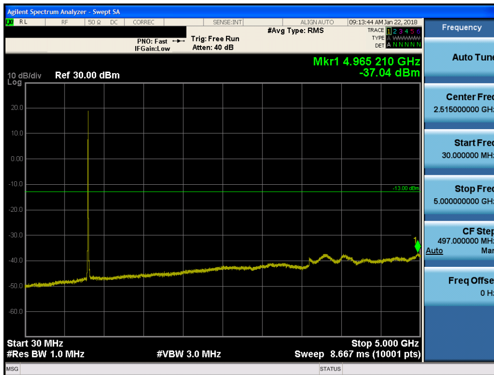
Plot 7-17. Conducted Spurious Plot (3MHz QPSK – RB Size 1, RB Offset 0 – High Channel)
