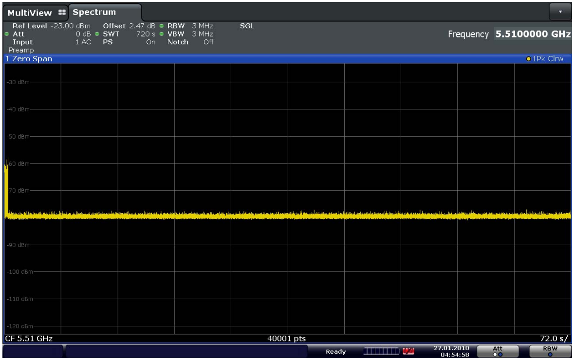
Figure 9-5. 5510MHz - Monitoring 10 minutes (40MHz)
