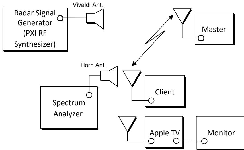
Figure 5-2. Mode-2 Test Setup
