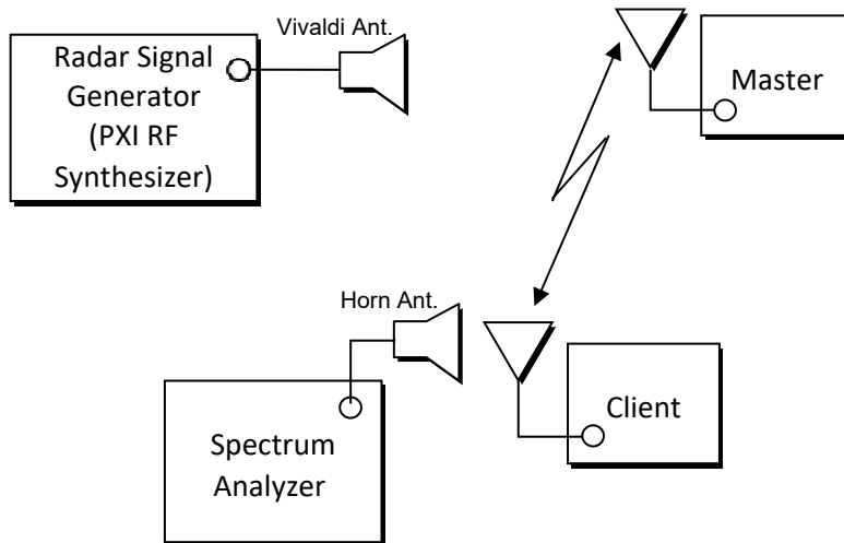
Figure 5-1. Mode-1 Test Setup
