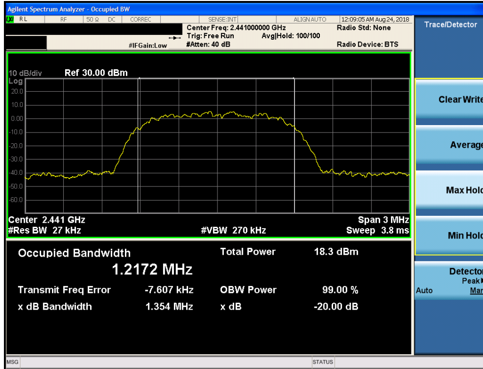
Plot 7-17. 20dB Bandwidth Plot ANT 2 (Bluetooth, 8DPSK, ePA – Ch. 39)
