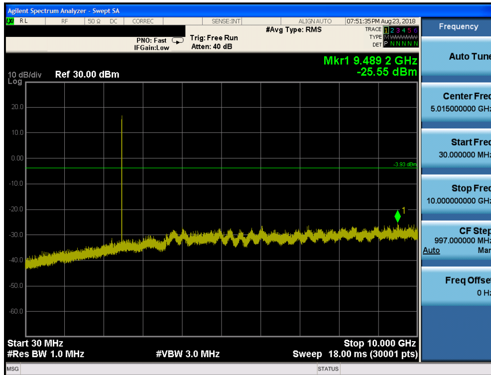
Plot 7-77. Conducted Spurious Plot ANT 1 (Bluetooth, GFSK, ePA – Ch. 78)
