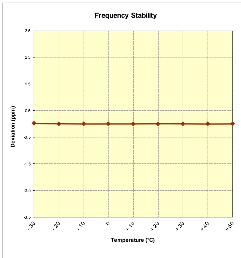
Figure 7-8. Frequency Stability Graph (Cellular WCDMA Mode – Ch. 4183)
