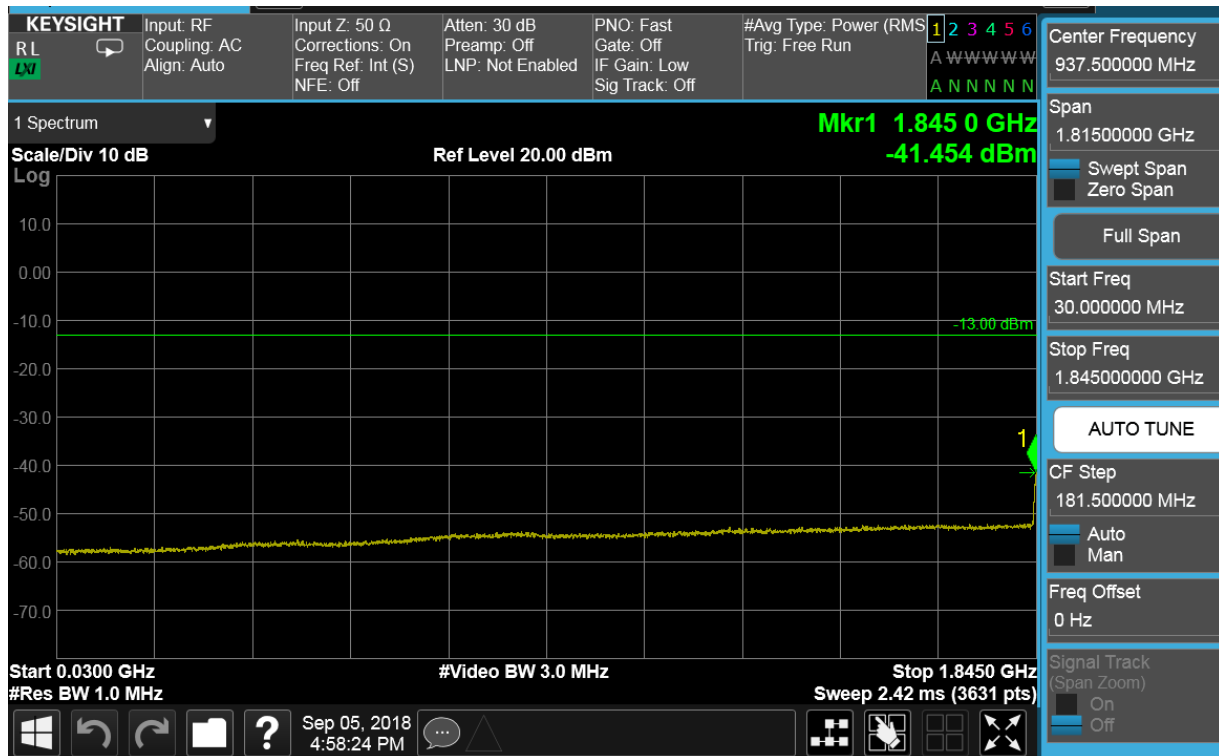
Plot 7-44. Conducted Spurious Plot (PCS WCDMA Mode - Low Channel)
