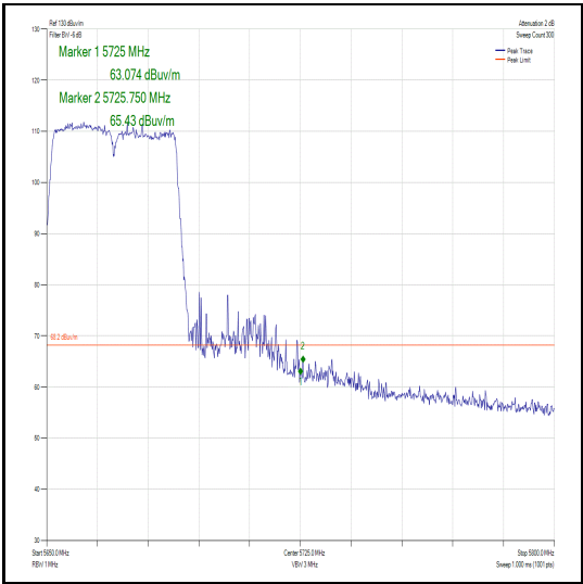
Figure 400 – Channel 134 - Authorised Band Edge
