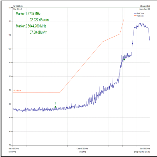
Figure 387 – Channel 149 - Authorized Band Edge
