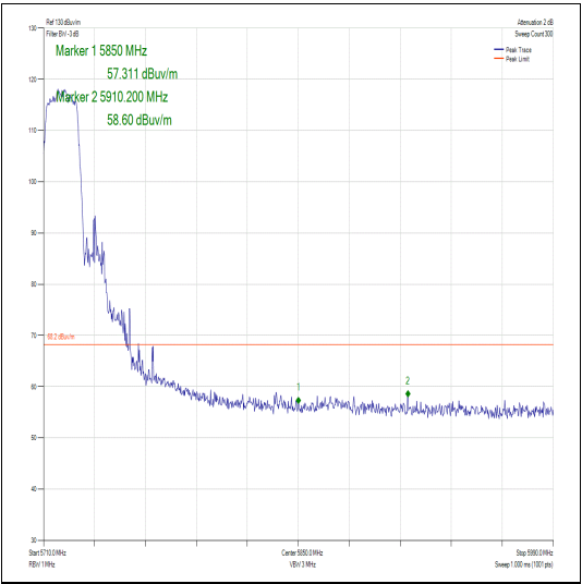
Figure 386 – Channel 144 - Authorized Band Edge
