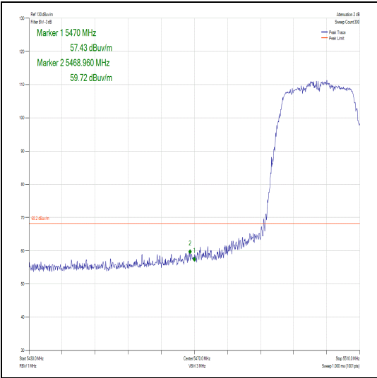
Figure 384 – Channel 100 - Authorized Band Edge
