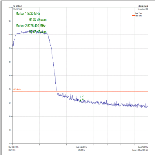
Figure 385 – Channel 140 - Authorized Band Edge
