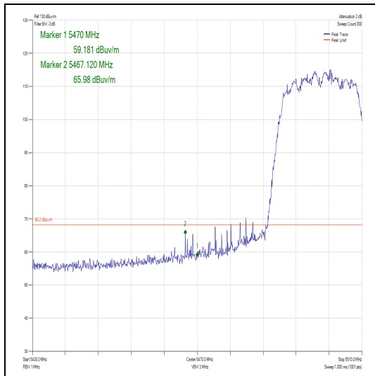
Figure 389 – Channel 100 - Authorised Band Edge
