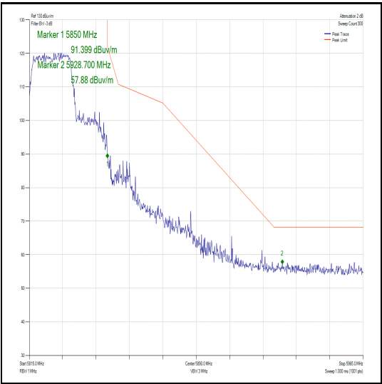
Figure 393 – Channel 165 - Authorised Band Edge
