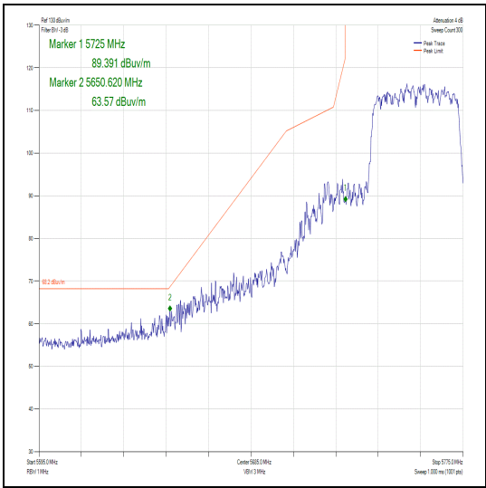
Figure 402 – Channel 151 - Authorised Band Edge
