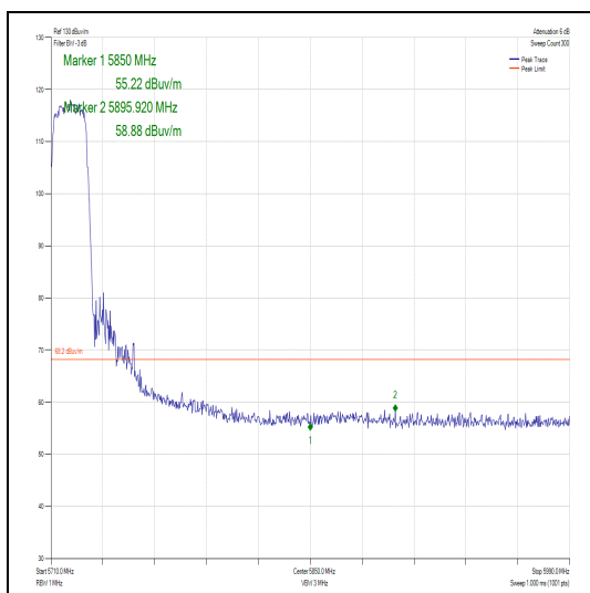
Figure 391 – Channel 144 - Authorised Band Edge
