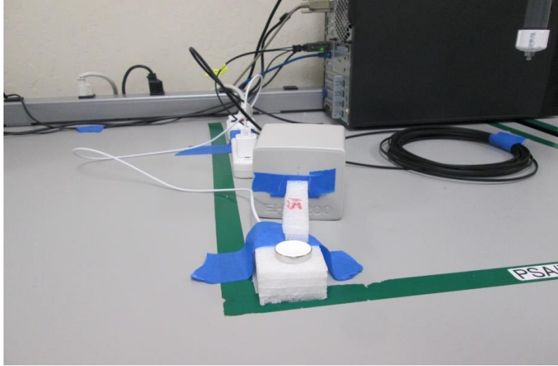
S1, RF EXPOSURE SETUP PHOTO 15cm
