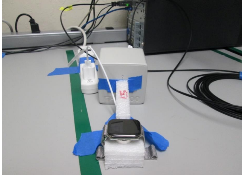
S1, RF EXPOSURE SETUP PHOTO 15 cm
