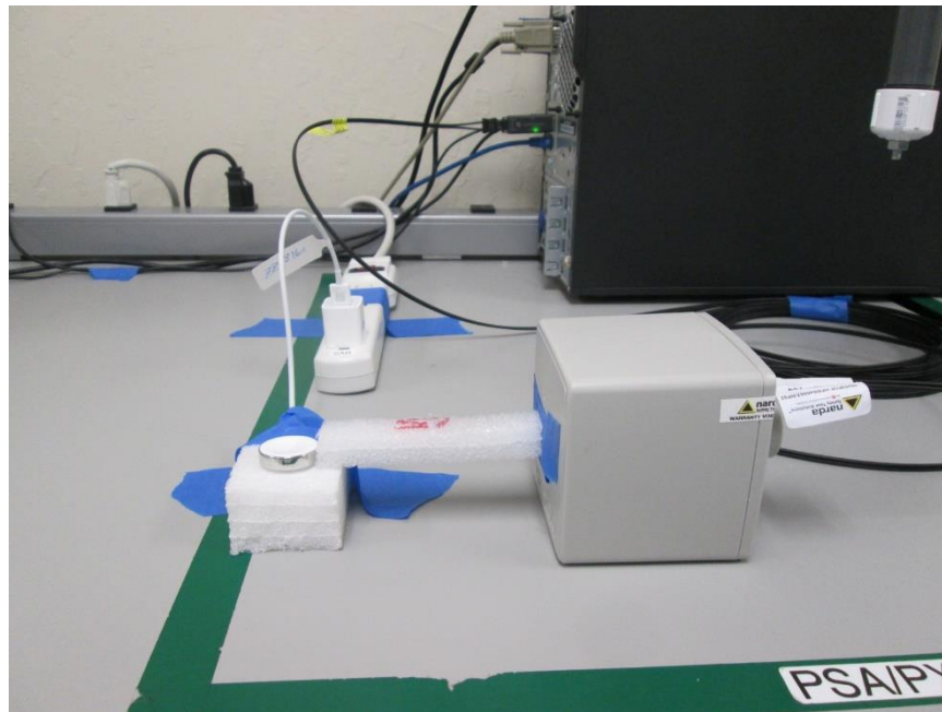
S2, RF EXPOSURE SETUP PHOTO 15cm
