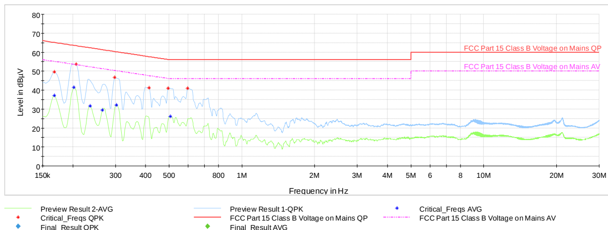
Plot 7-6. Line Conducted Plot (N, with AC/DC Adapter)
