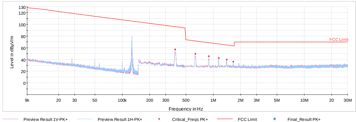
Plot 7-3. Radiated Spurious Plot from 9kHz – 30MHz (Loop Antenna X & Y)
