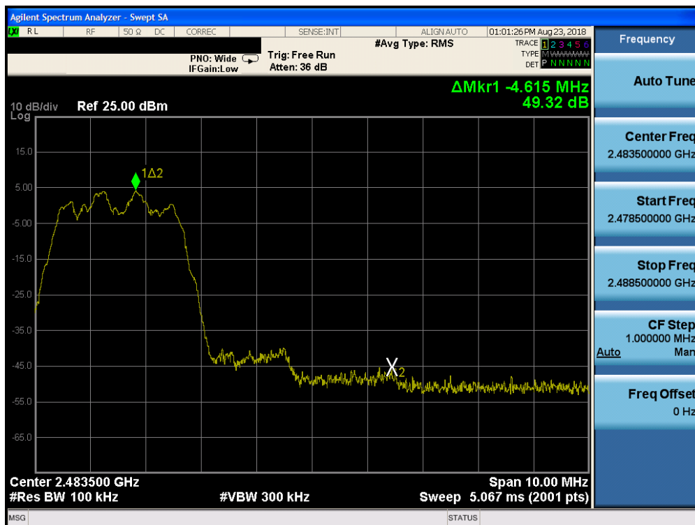
Plot 7-56. Band Edge Plot ANT0 (Bluetooth (HDR4, ePA), 4Mbps – Ch. 75)
