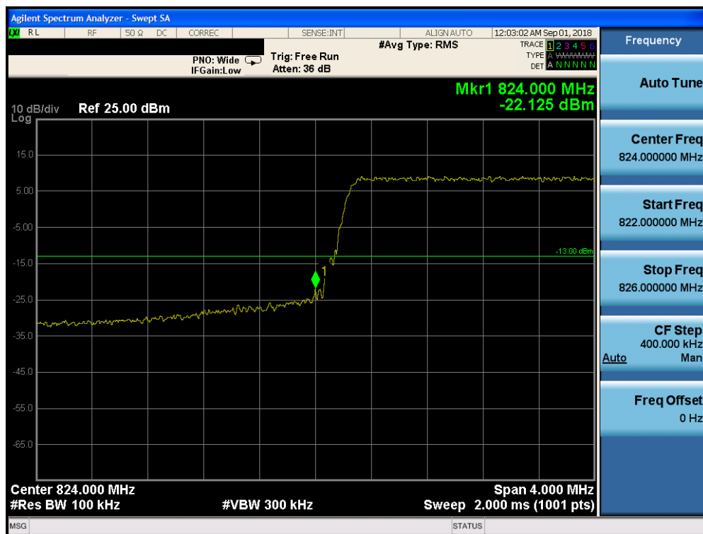
Plot 7-192. Lower Band Edge Plot (Band 26 - 5.0MHz QPSK - RB Size 25)
