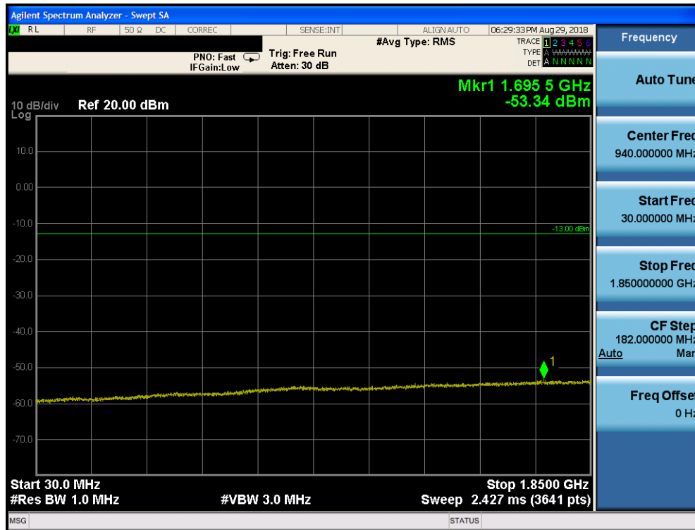
Plot 7-133. Conducted Spurious Plot (Band 25/2 – 20.0MHz QPSK – RB Size 1, RB Offset 0 – High Channel)
