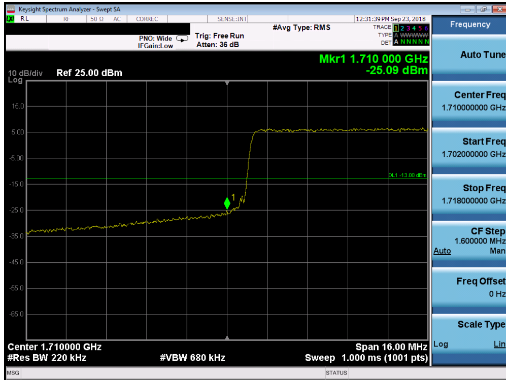
Plot 7-216. Lower Band Edge Plot (Band 4 – 20.0MHz QPSK – RB Size 100)
