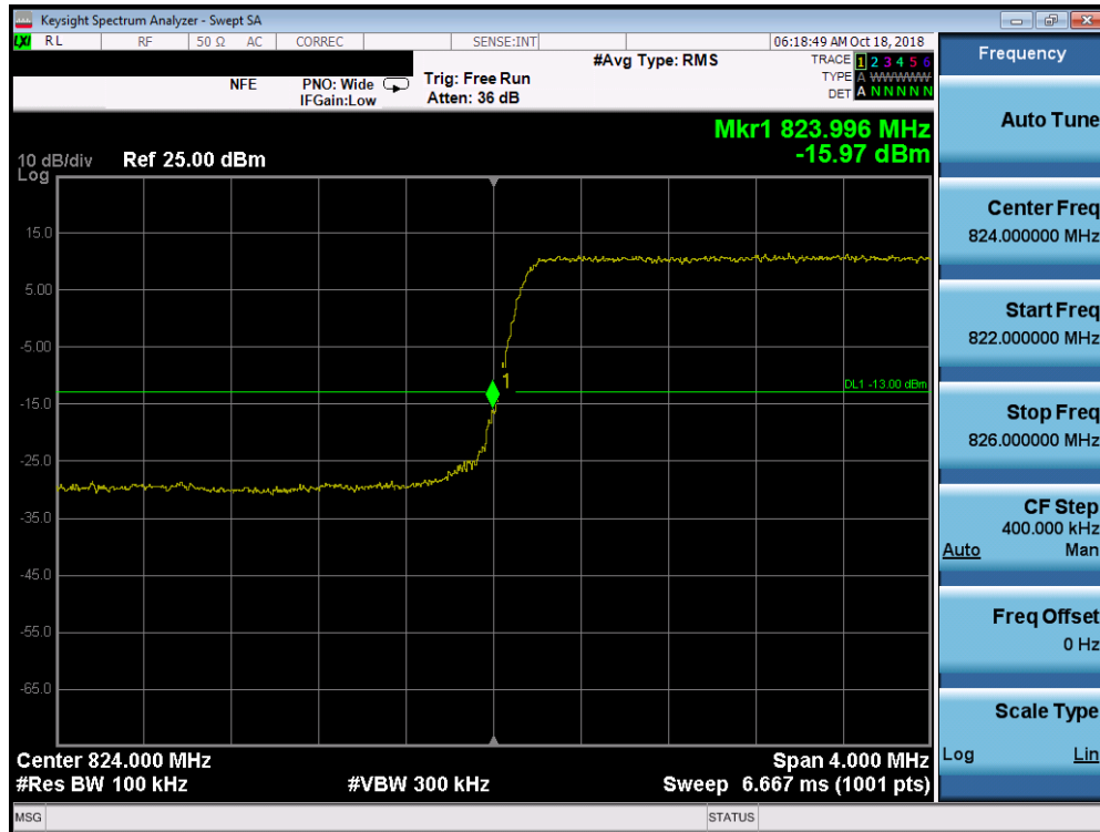
Plot 7-179. Lower Band Edge Plot (Band 5 – 3.0MHz QPSK – RB Size 15)
