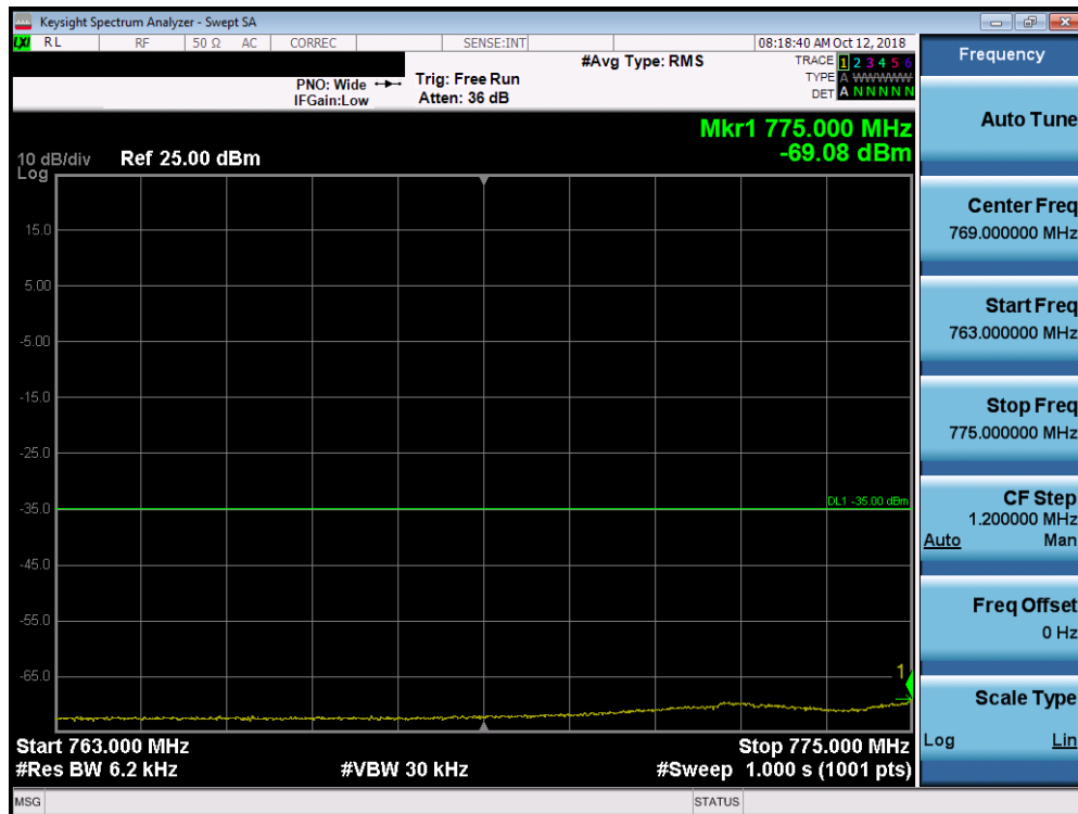
Plot 7-174. Lower Emission Mask Edge Plot (Band 13 – 10.0MHz QPSK – RB Size 50)
