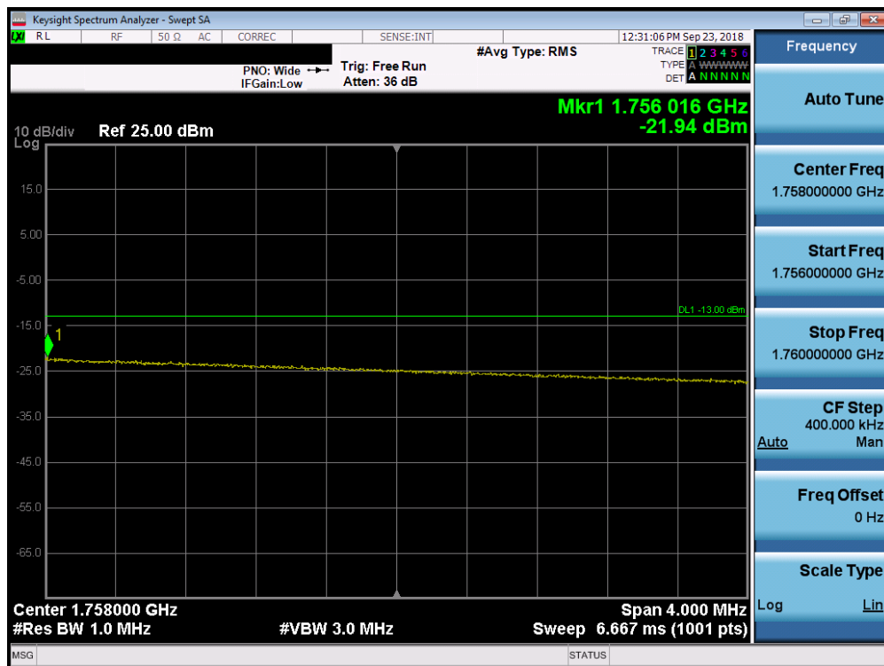
Plot 7-219. Upper Extended Band Edge Plot (Band 4 – 20.0MHz QPSK – RB Size 100)
