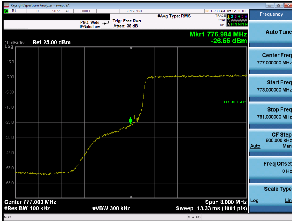
Plot 7-173. Lower Band Edge Plot (Band 13 – 10.0MHz QPSK – RB Size 50)
