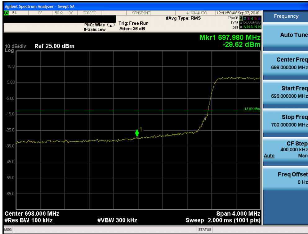
Plot 7-161. Lower Band Edge Plot (Band 12 – 5.0MHz QPSK – RB Size 25)
