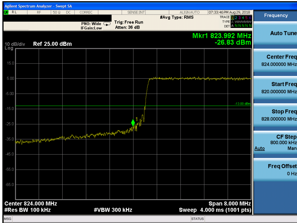
Plot 7-183. Lower Band Edge Plot (Band 5 – 10.0MHz QPSK – RB Size 50)
