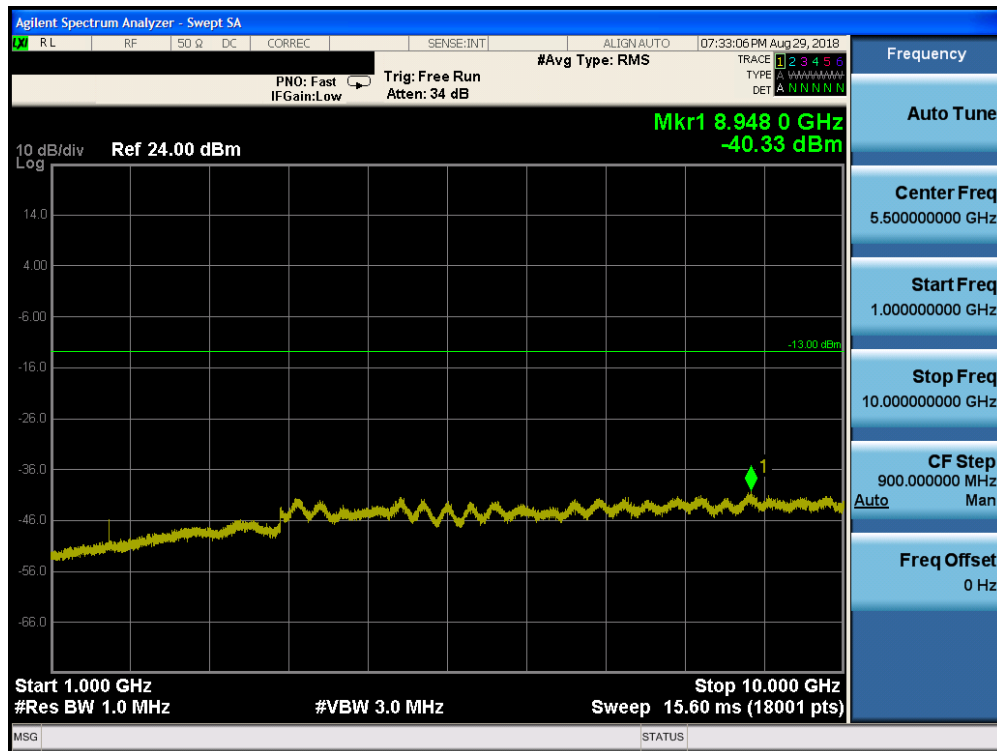
Plot 7-111. Conducted Spurious Plot (Band 26/5 – 10.0MHz QPSK – RB Size 1, RB Offset 0 – Low Channel)
