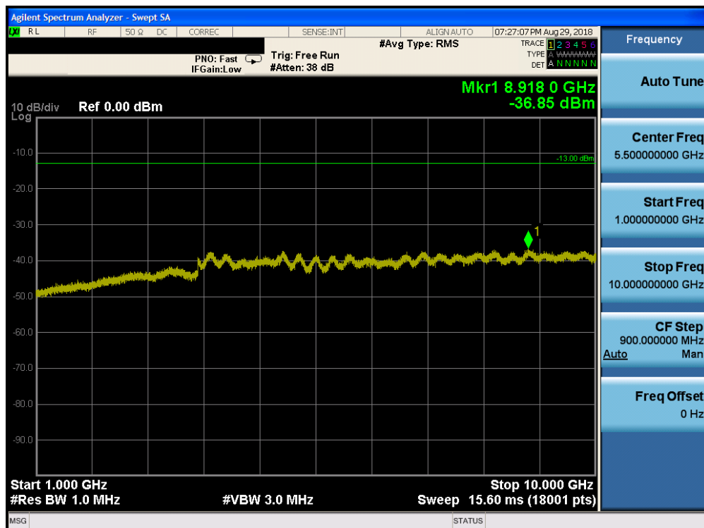
Plot 7-114. Conducted Spurious Plot (Band 26/5 – 10.0MHz QPSK – RB Size 1, RB Offset 0 – Mid Channel)
