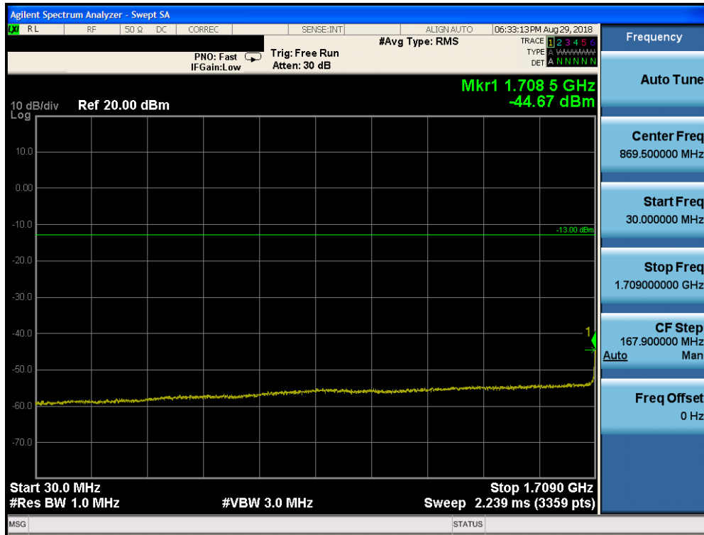
Plot 7-118. Conducted Spurious Plot (Band 66/4 – 20.0MHz QPSK – RB Size 1, RB Offset 0– Low Channel)
