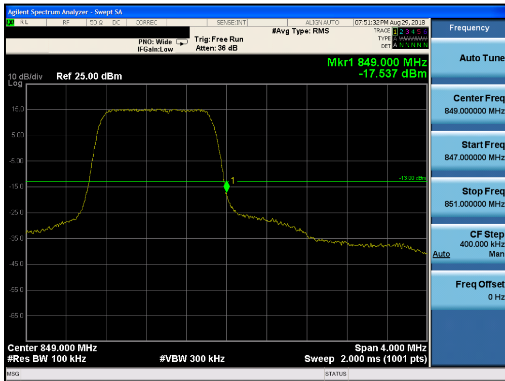
Plot 7-178. Upper Band Edge Plot (Band 5 – 1.4MHz QPSK – RB Size 6)
