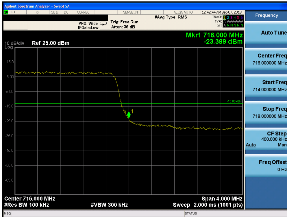
Plot 7-162. Upper Band Edge Plot (Band 12 – 5.0MHz QPSK – RB Size 25)
