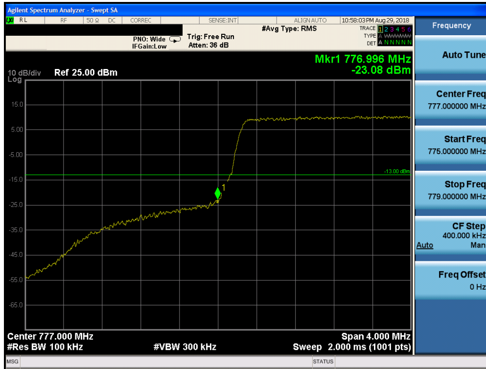
Plot 7-169. Lower Band Edge Plot (Band 13 – 5.0MHz QPSK – RB Size 25)
