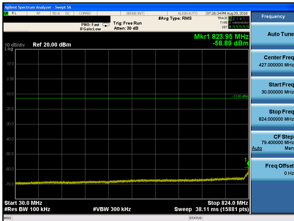
Plot 7-112. Conducted Spurious Plot (Band 26/5 – 10.0MHz QPSK – RB Size 1, RB Offset 0 – Mid Channel)
