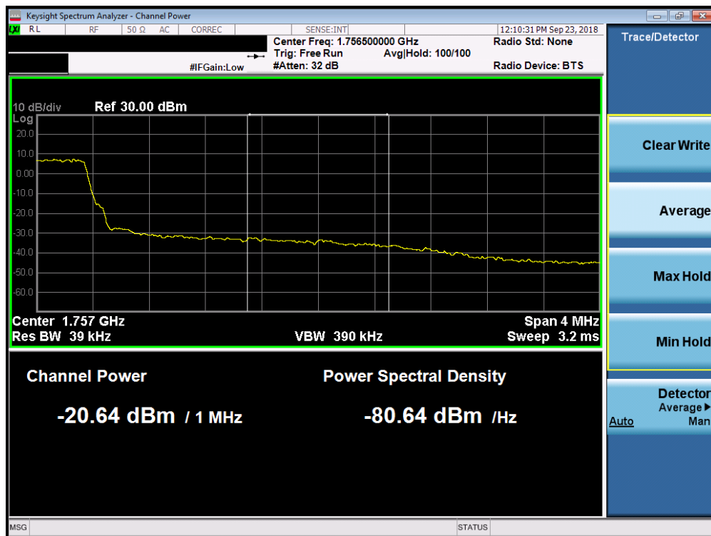
Plot 7-203. Upper Extended Band Edge Plot (Band 4 – 3.0MHz QPSK – RB Size 15)
