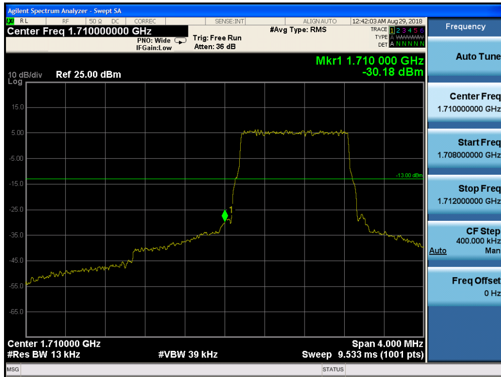
Plot 7-220. Lower Band Edge Plot (Band 66 – 1.4MHz QPSK – RB Size 6)
