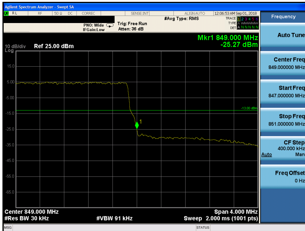
Plot 7-190. Upper Band Edge Plot (Band 26 – 3.0MHz QPSK – RB Size 15)
