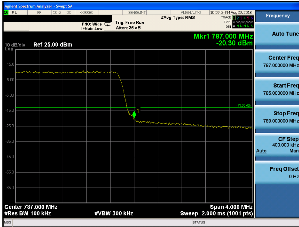
Plot 7-171. Upper Band Edge Plot (Band 13 – 5.0MHz QPSK – RB Size 25)
