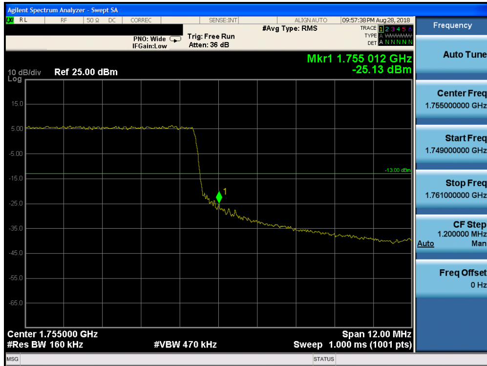
Plot 7-214. Upper Band Edge Plot (Band 4 – 15.0MHz QPSK – RB Size 75)
