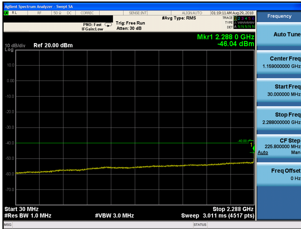
Plot 7-136. Conducted Spurious Plot (Band 30 – 10.0MHz QPSK – RB Size 1, RB Offset 0)
