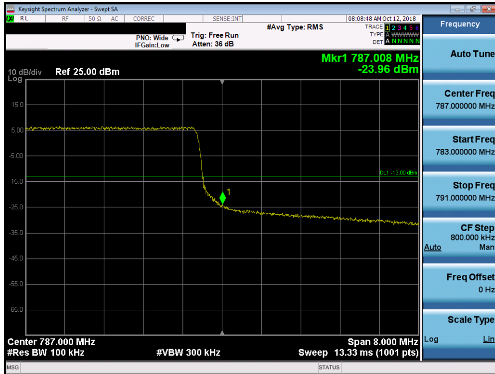
Plot 7-175. Upper Band Edge Plot (Band 13 – 10.0MHz QPSK – RB Size 50)
