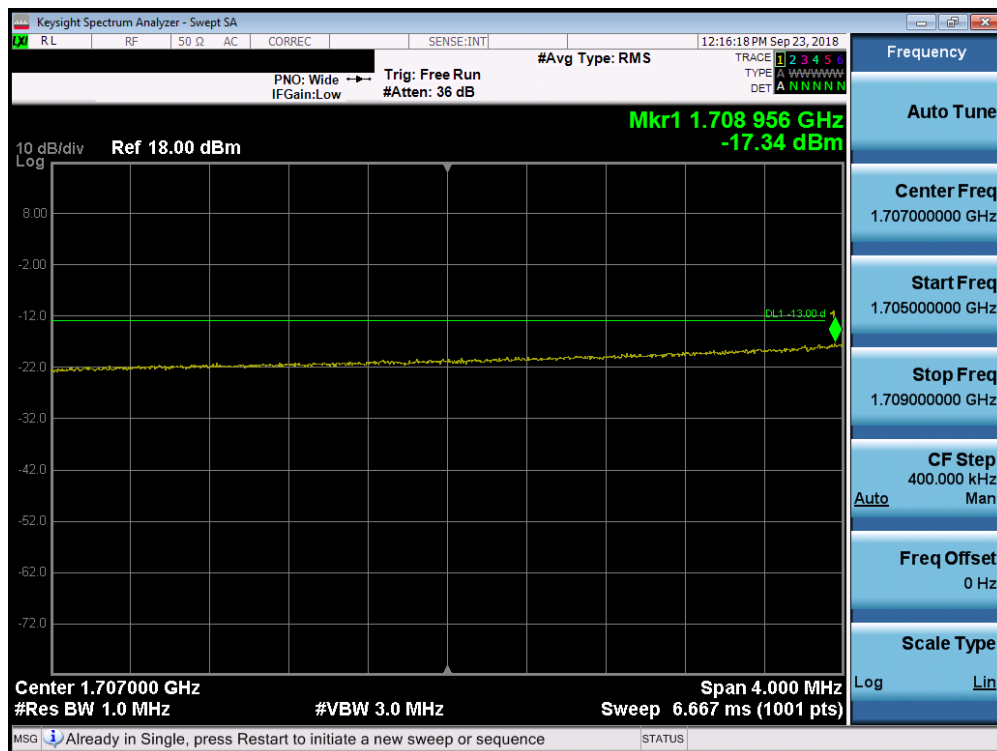
Plot 7-209. Lower Extended Band Edge Plot (Band 4 – 10.0MHz QPSK – RB Size 50)
