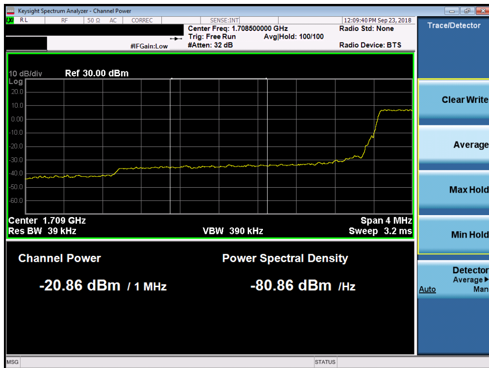
Plot 7-201. Lower Extended Band Edge Plot (Band 4 – 3.0MHz QPSK – RB Size 15)
