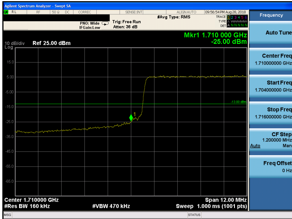
Plot 7-212. Lower Band Edge Plot (Band 4 – 15.0MHz QPSK – RB Size 75)
