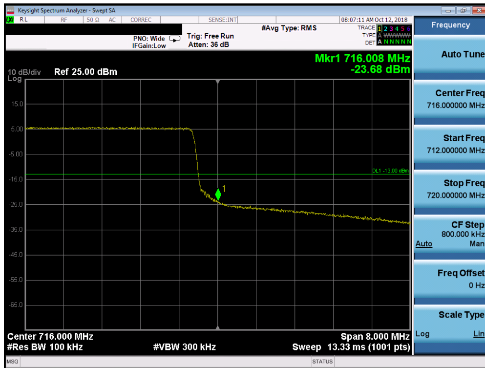
Plot 7-168. Upper Band Edge Plot (Band 17 – 10.0MHz QPSK – RB Size 50)
