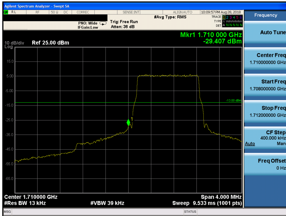
Plot 7-196. Lower Band Edge Plot (Band 4 – 1.4MHz QPSK – RB Size 6)
