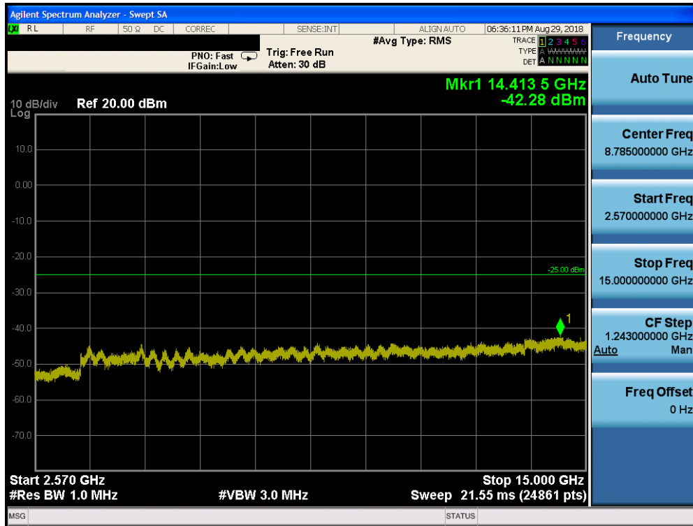
Plot 7-143. Conducted Spurious Plot (Band 7 - 20.0MHz QPSK - RB Size 1, RB Offset 0 - Mid Channel)
