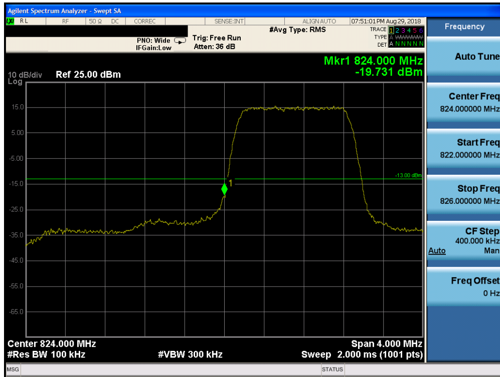
Plot 7-177. Lower Band Edge Plot (Band 5 – 1.4MHz QPSK – RB Size 6)
