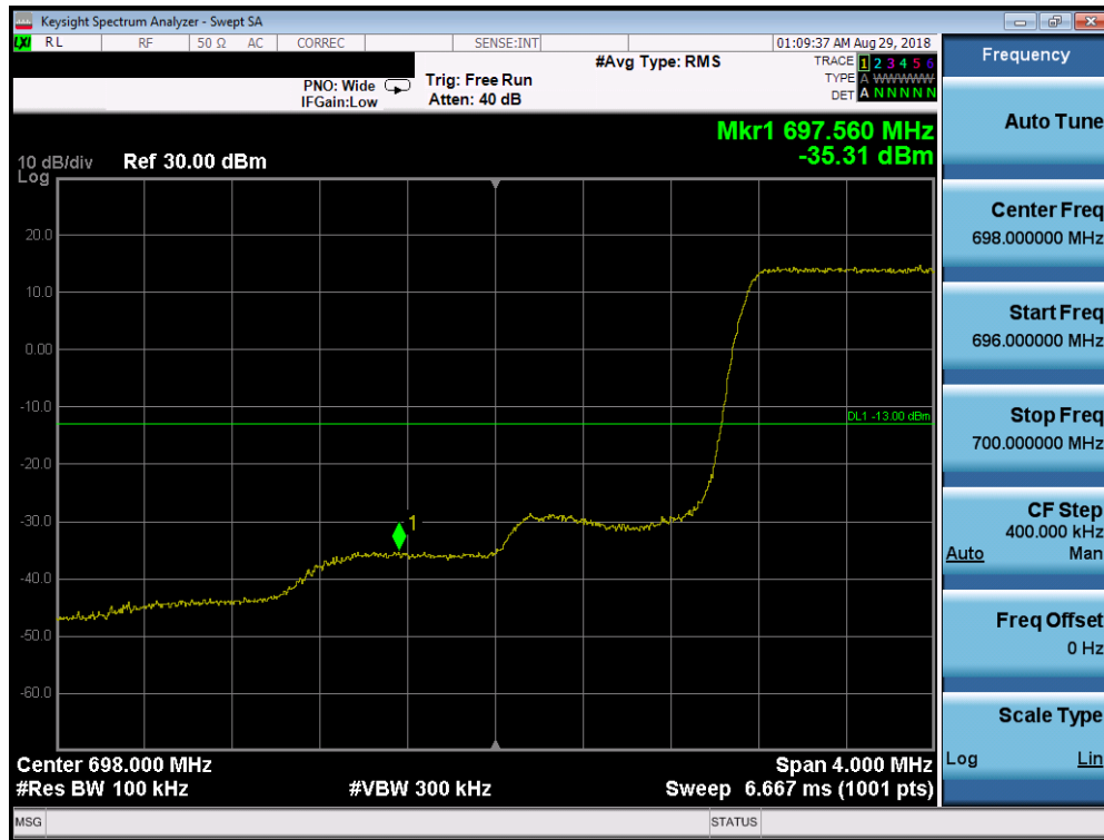
Plot 7-157. Lower Band Edge Plot (Band 12 – 1.4MHz QPSK – RB Size 6)
