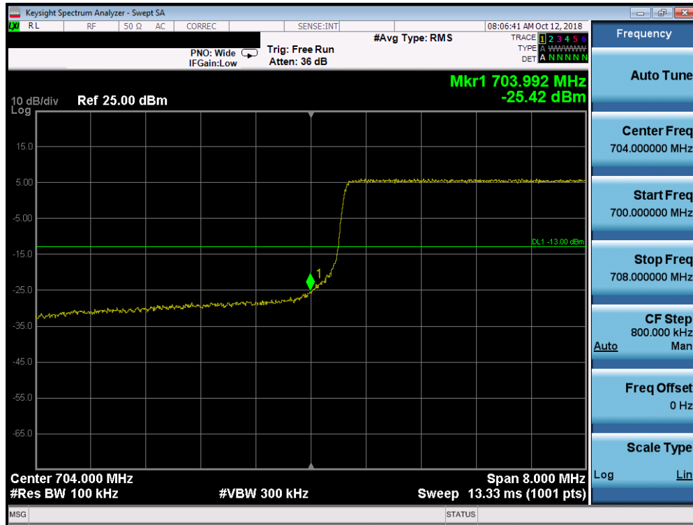
Plot 7-167. Lower Band Edge Plot (Band 17 – 10.0MHz QPSK – RB Size 50)
