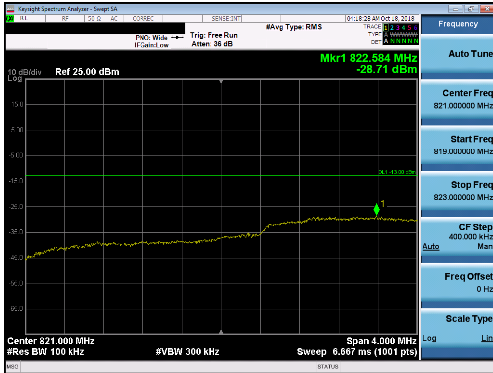
Plot 7-189. Upper Extended Band Edge Plot (Band 26 – 3MHz QPSK – RB Size 6)
