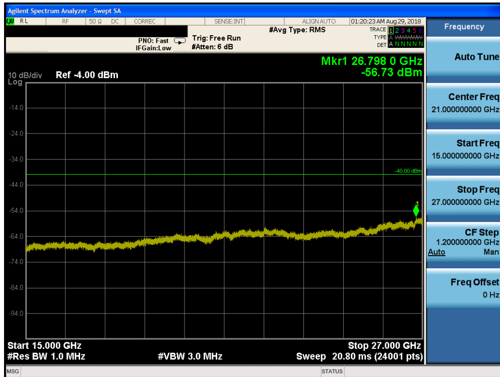
Plot 7-138. Conducted Spurious Plot (Band 30 – 10.0MHz QPSK – RB Size 1, RB Offset 0)
