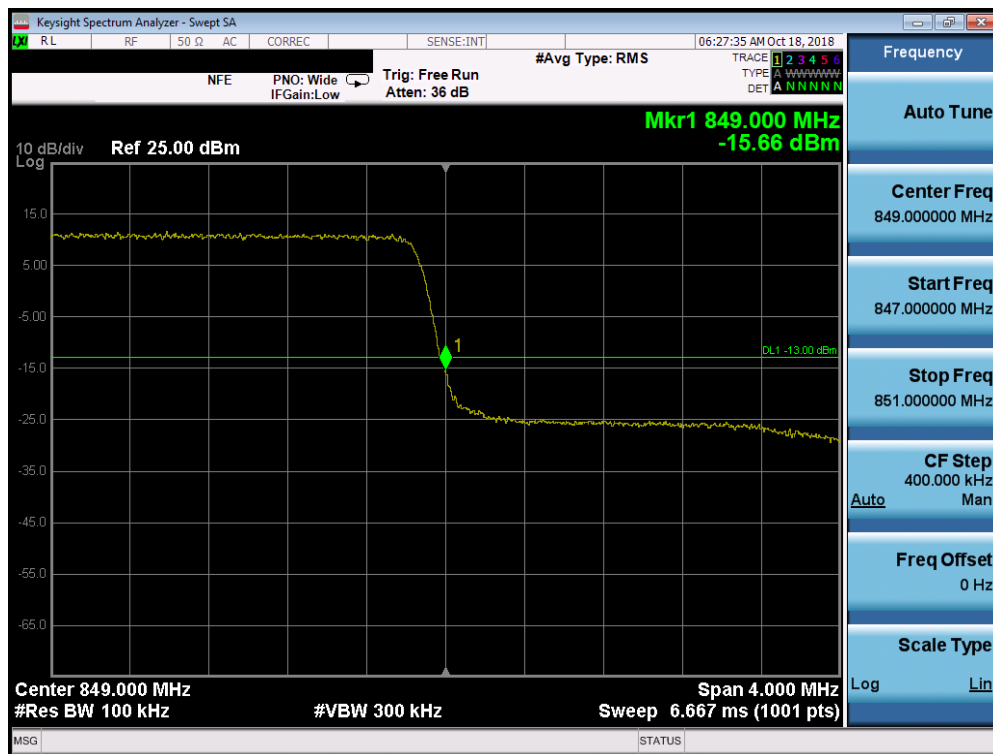
Plot 7-180. Upper Band Edge Plot (Band 5 – 3.0MHz QPSK – RB Size 15)
