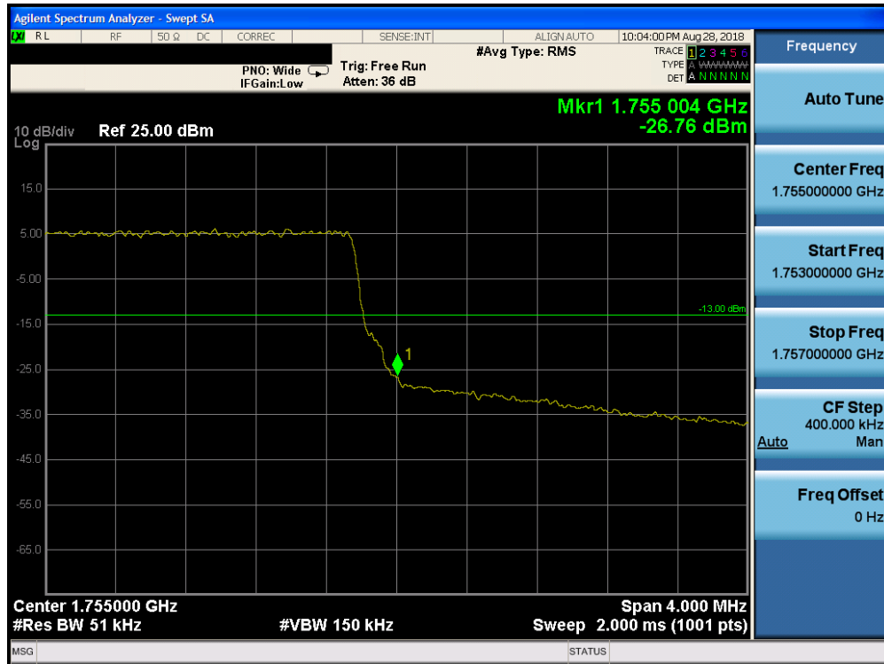
Plot 7-206. Upper Band Edge Plot (Band 4 – 5.0MHz QPSK – RB Size 25)
