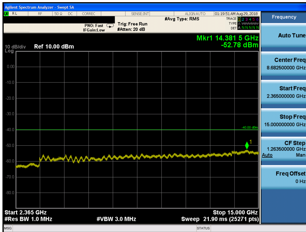
Plot 7-137. Conducted Spurious Plot (Band 30 – 10.0MHz QPSK – RB Size 1, RB Offset 0)
