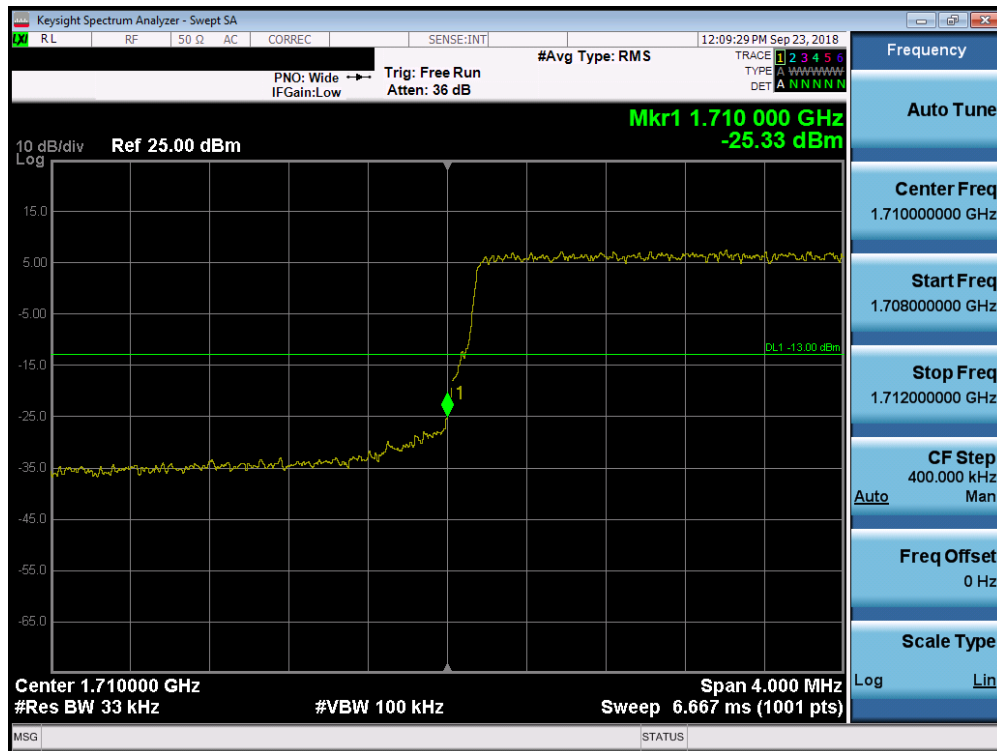
Plot 7-200. Lower Band Edge Plot (Band 4 – 3.0MHz QPSK – RB Size 15)
