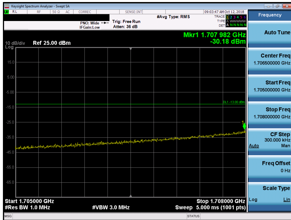
Plot 7-221. Lower Extended Band Edge Plot (Band 66 – 1.4MHz QPSK – RB Size 6)
