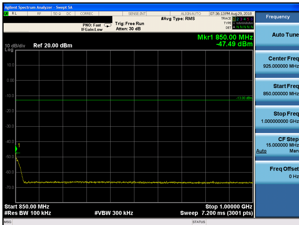
Plot 7-116. Conducted Spurious Plot (Band 26/5 – 10.0MHz QPSK – RB Size 1, RB Offset 0 – High Channel)
