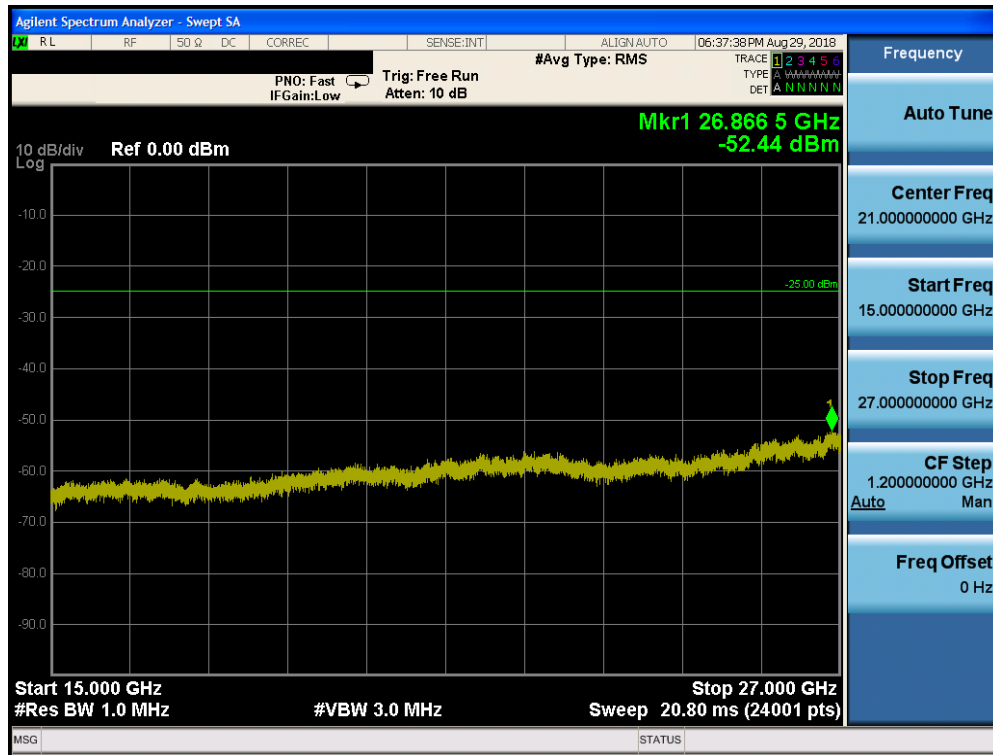
Plot 7-141. Conducted Spurious Plot (Band 7 - 20.0MHz QPSK - RB Size 1, RB Offset 0 - Low Channel)
