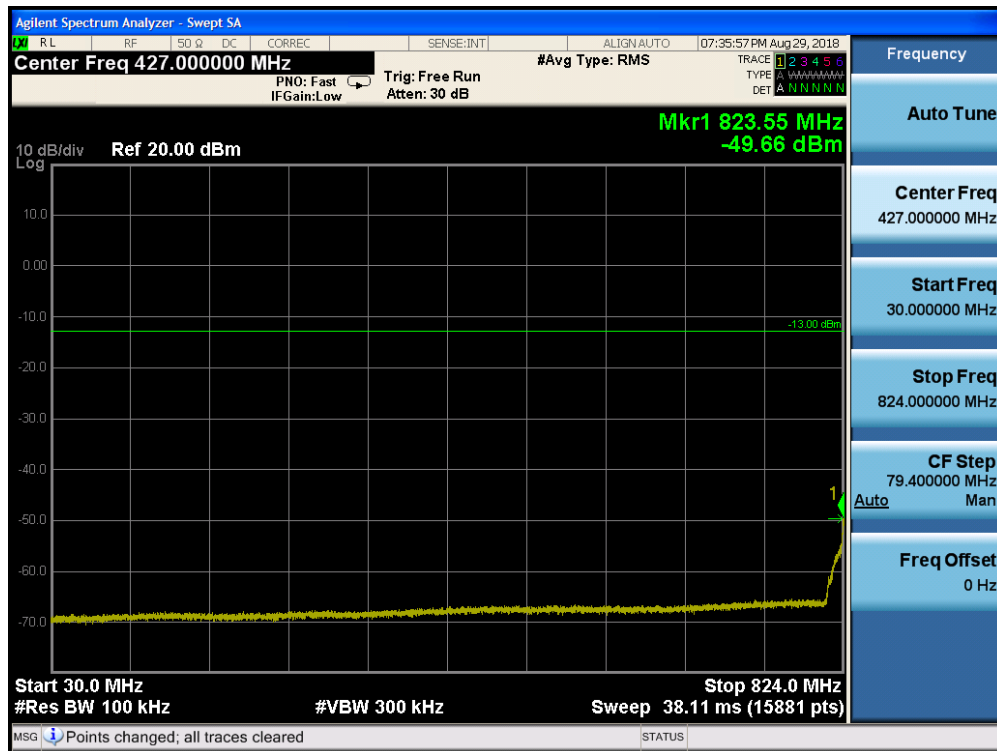
Plot 7-115. Conducted Spurious Plot (Band 26/5 – 10.0MHz QPSK – RB Size 1, RB Offset 0 – High Channel)
