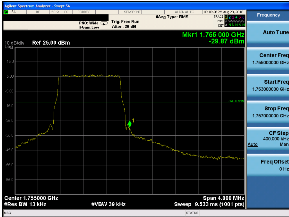
Plot 7-198. Upper Band Edge Plot (Band 4 – 1.4MHz QPSK – RB Size 6)
