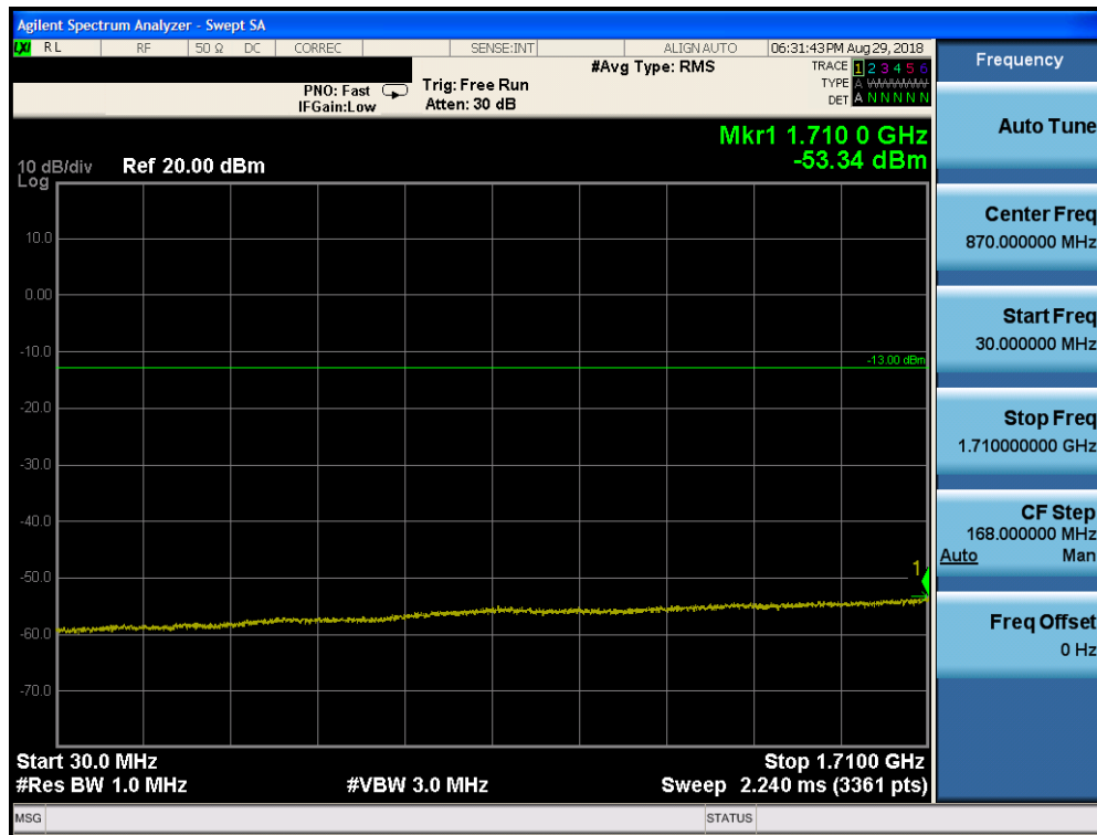
Plot 7-121. Conducted Spurious Plot (Band 66/4 – 20.0MHz QPSK – RB Size 1, RB Offset 0 – Mid Channel)
