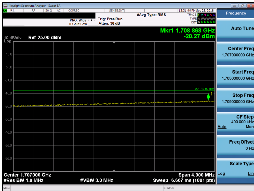
Plot 7-217. Lower Extended Band Edge Plot (Band 4 – 20.0MHz QPSK – RB Size 100)
