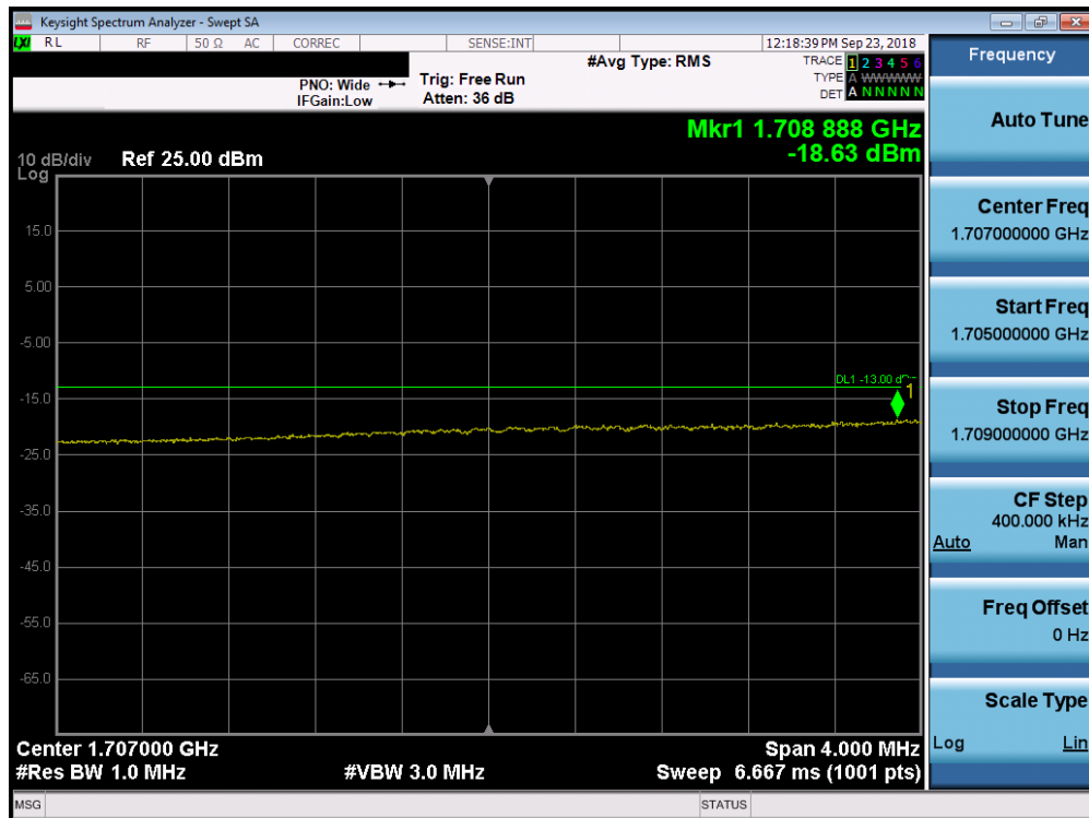
Plot 7-213. Lower Extended Band Edge Plot (Band 4 – 15.0MHz QPSK – RB Size 75)
