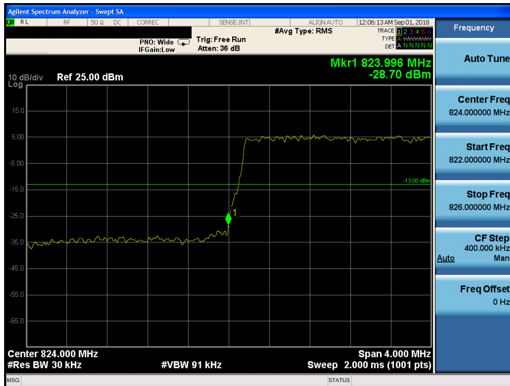
Plot 7-188. Lower Band Edge Plot (Band 26 – 3.0MHz QPSK – RB Size 15)
