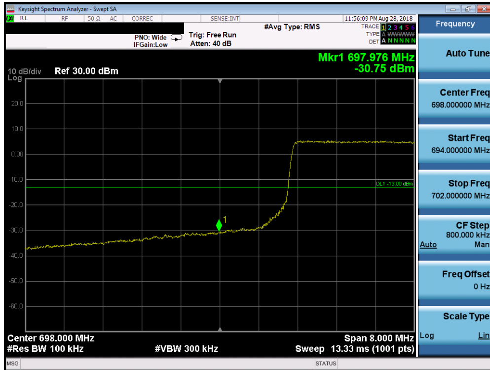
Plot 7-163. Lower Band Edge Plot (Band 12 – 10.0MHz QPSK – RB Size 50)
