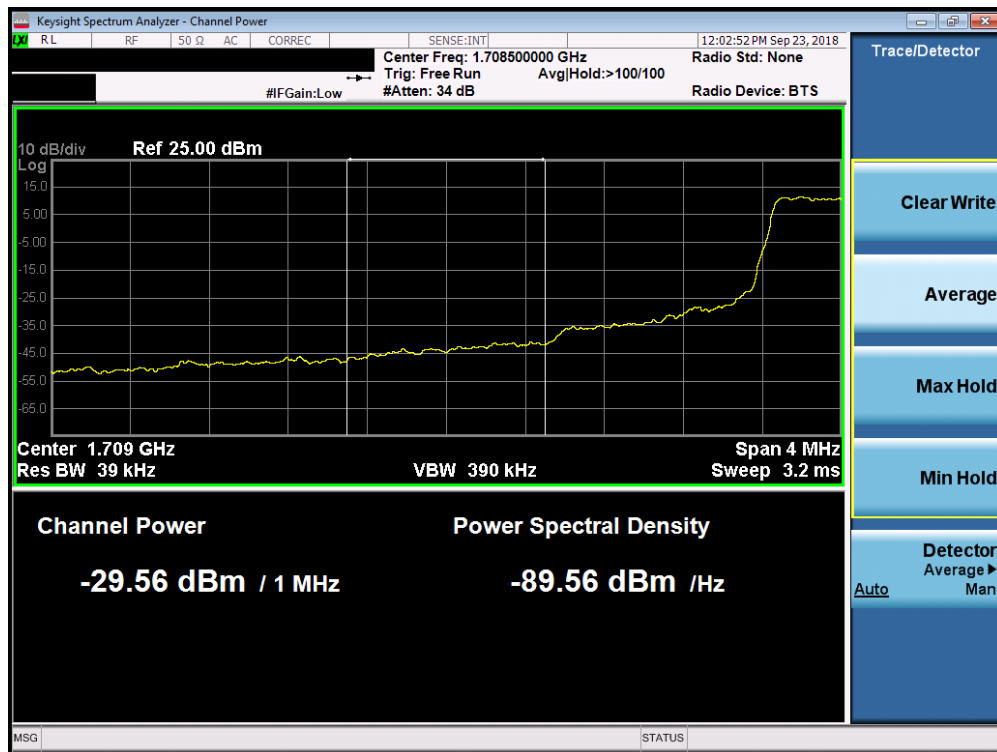
Plot 7-197. Lower Extended Band Edge Plot (Band 4 – 1.4MHz QPSK – RB Size 6)
