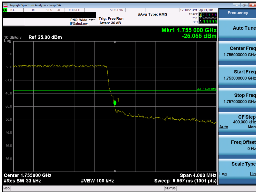
Plot 7-202. Upper Band Edge Plot (Band 4 – 3.0MHz QPSK – RB Size 15)
