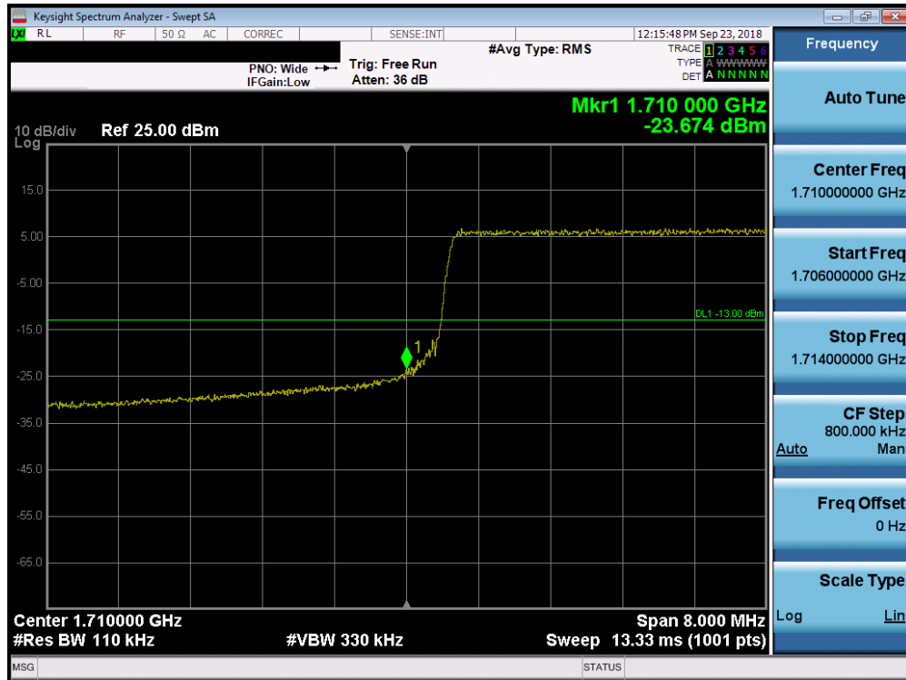
Plot 7-208. Lower Band Edge Plot (Band 4 – 10.0MHz QPSK – RB Size 50)
