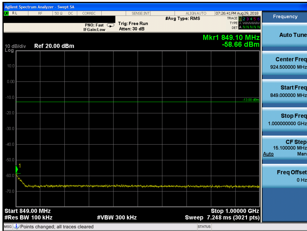
Plot 7-113. Conducted Spurious Plot (Band 26/5 – 10.0MHz QPSK – RB Size 1, RB Offset 0 – Mid Channel)
