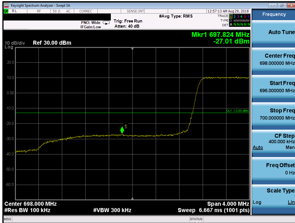
Plot 7-159. Lower Band Edge Plot (Band 12 – 3.0MHz QPSK – RB Size 15)
