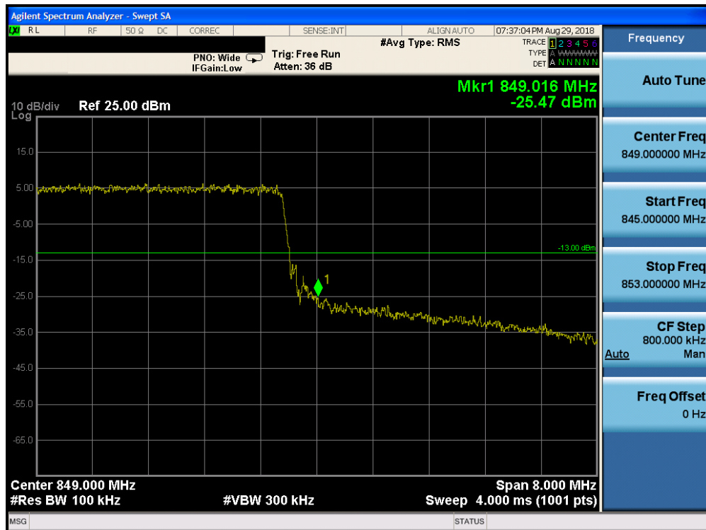
Plot 7-184. Upper Band Edge Plot (Band 5 – 10.0MHz QPSK – RB Size 50)
