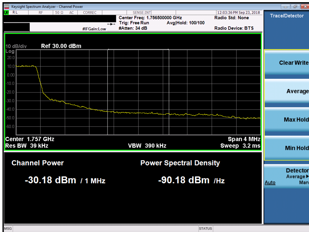
Plot 7-199. Upper Extended Band Edge Plot (Band 4 – 1.4MHz QPSK – RB Size 6)
