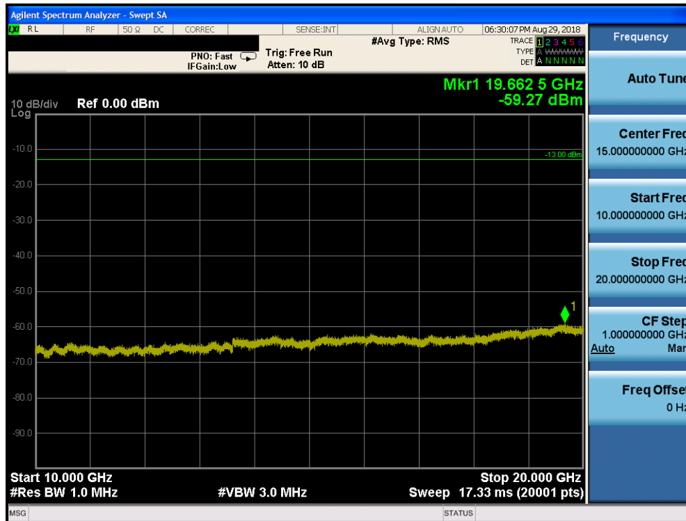
Plot 7-135. Conducted Spurious Plot (Band 25/2 – 20.0MHz QPSK – RB Size 1, RB Offset 0 – High Channel)
