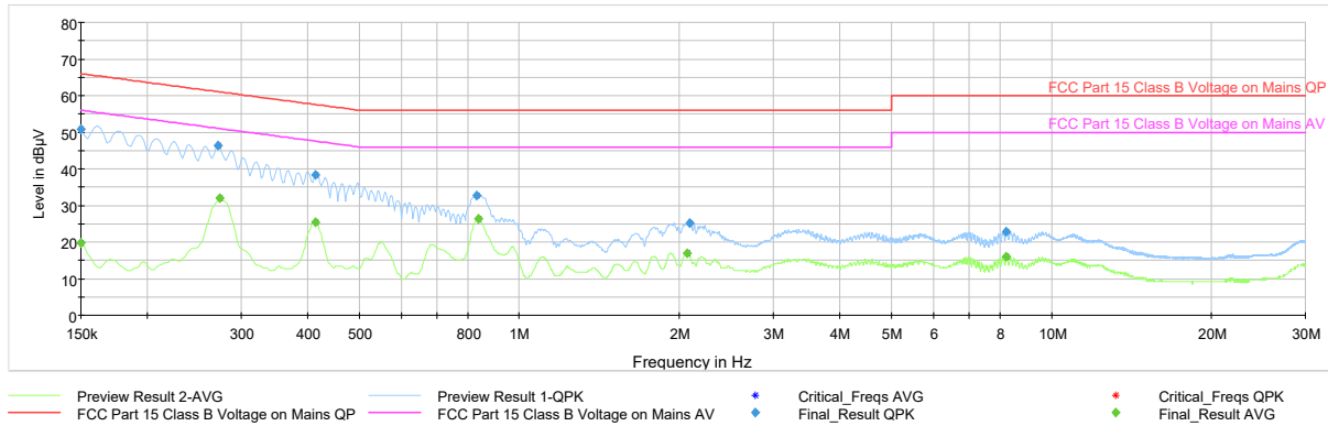
Plot 7-33. Line Conducted Plot with Bluetooth LE (GFSK ePA, L1)
