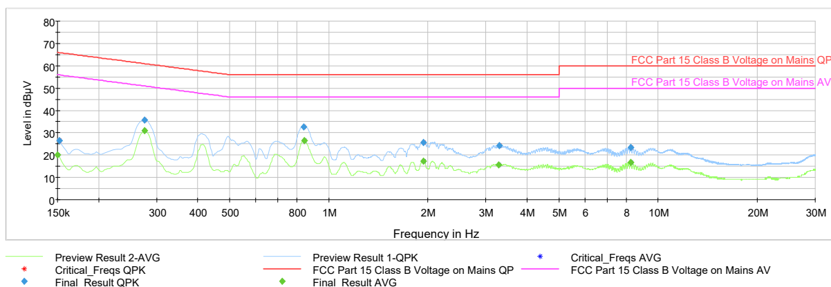
Plot 7-80. Line-Conducted Test Plot (L1)
