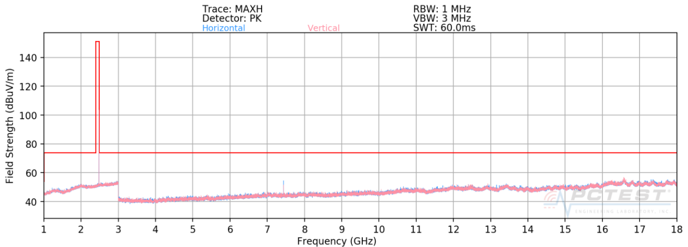
Plot 7-37. Radiated Spurious Plot above 1GHz (BT GFSK – Ch. 78)
