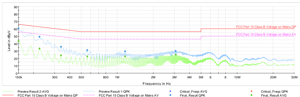
Plot 7-33. AC Line Conducted Plot with Bluetooth LE (L1 – 1Mbps, with Laptop)
