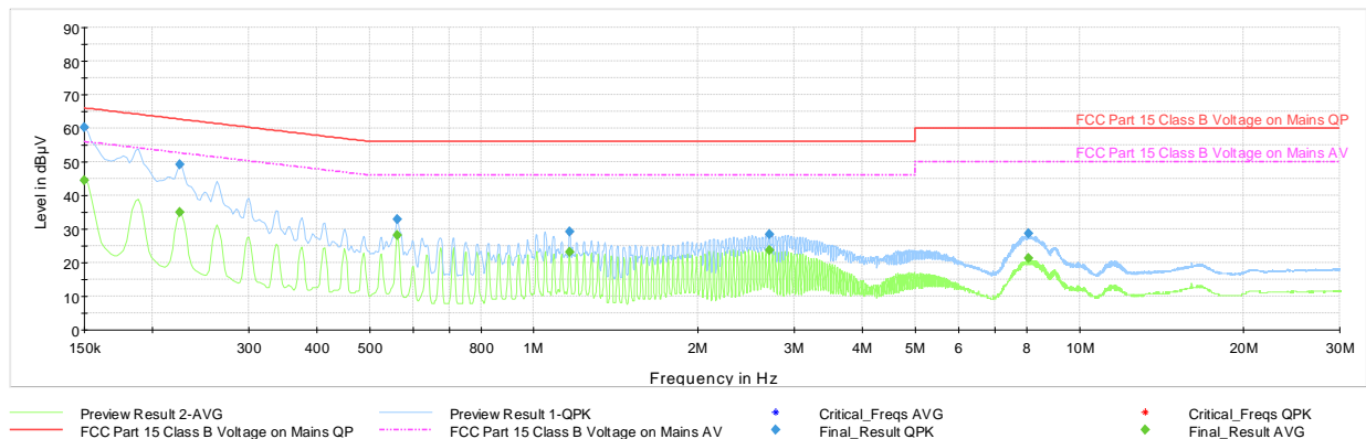
Plot 7-34. AC Line Conducted Plot with Bluetooth LE (N – 1Mbps, with Laptop)
