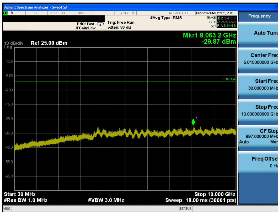
Plot 7-73. Conducted Spurious Plot ANT 1 (Bluetooth, GFSK, ePA – Ch. 0)
