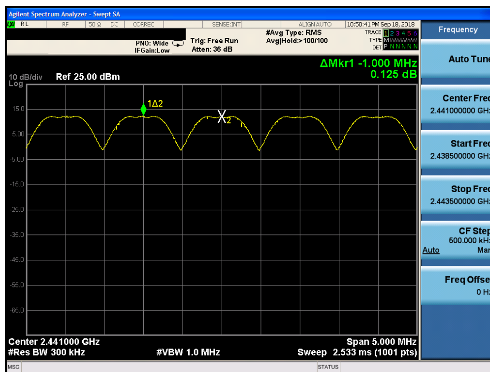
Plot 7-47. Channel Spacing Plot ANT2 (Bluetooth, GFSK, ePA)
