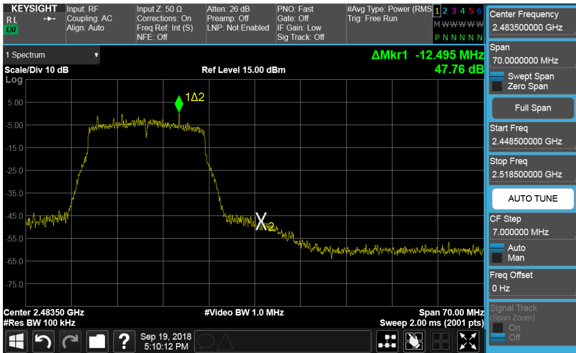
Plot 7-101. Band Edge Plot SISO Core 1 Primary (802.11n (2.4GHz) – Ch. 12)
