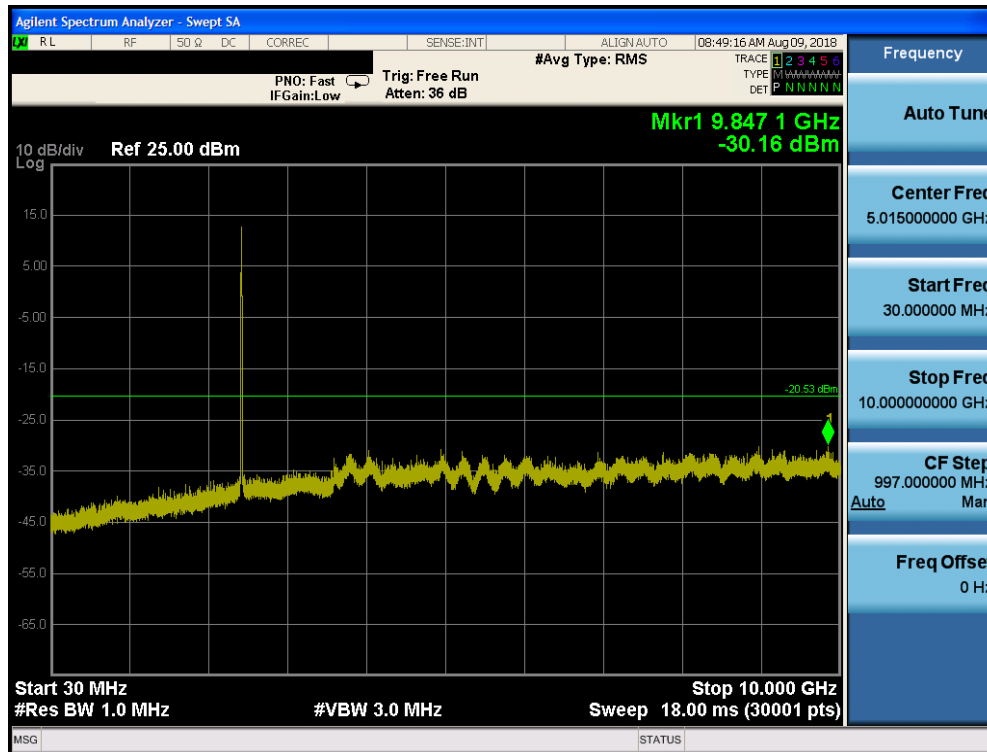
Plot 7-117. Conducted Spurious Plot SISO Core 0 (802.11b – Ch. 6)
