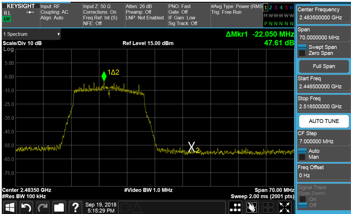
Plot 7-102. Band Edge Plot SISO Core 1 Primary (802.11n (2.4GHz) – Ch. 13)
