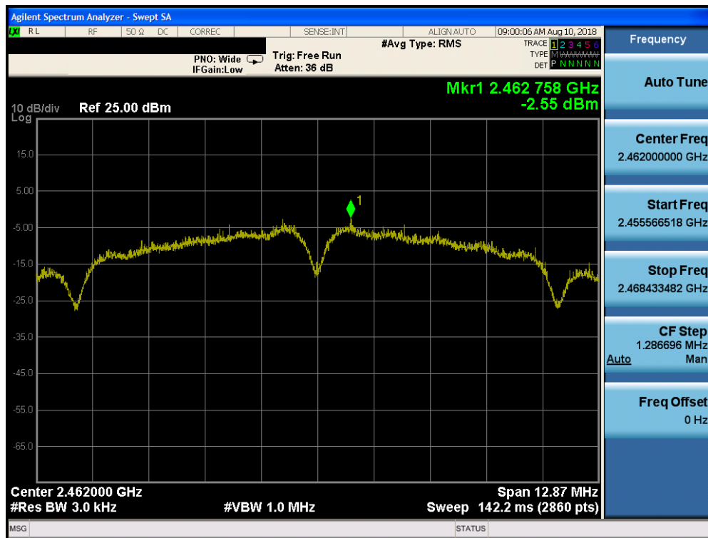
Plot 7-30. Power Spectral Density Plot SISO Core 0 (802.11b – Ch. 11)
