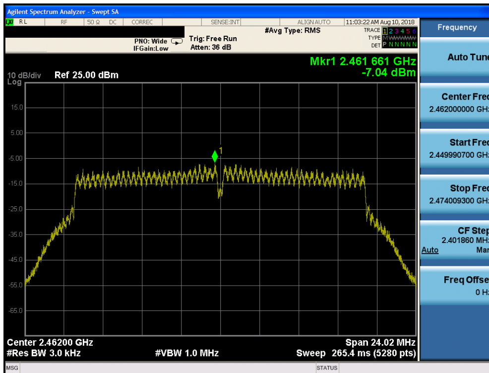
Plot 7-36. Power Spectral Density Plot SISO Core 0 (802.11n (2.4GHz) – Ch. 11)
