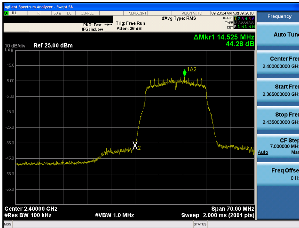
Plot 7-87. Band Edge Plot SISO Core 0 (802.11n (2.4GHz) – Ch. 1)
