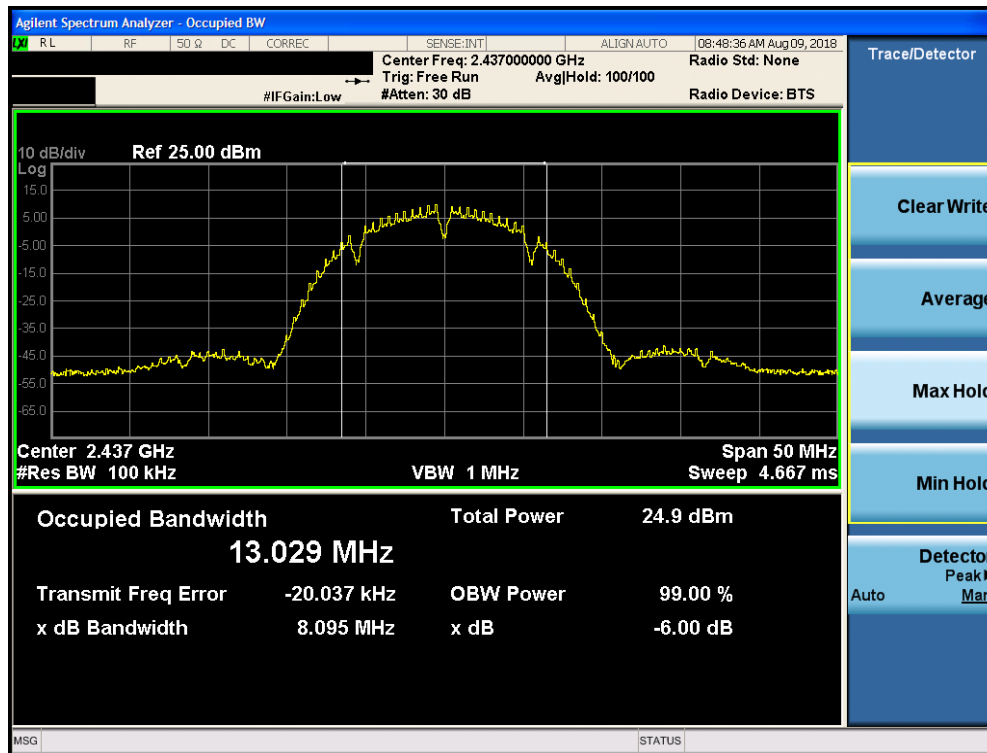
Plot 7-2. 6dB Bandwidth Plot SISO Core 0 (802.11b – Ch. 6)
