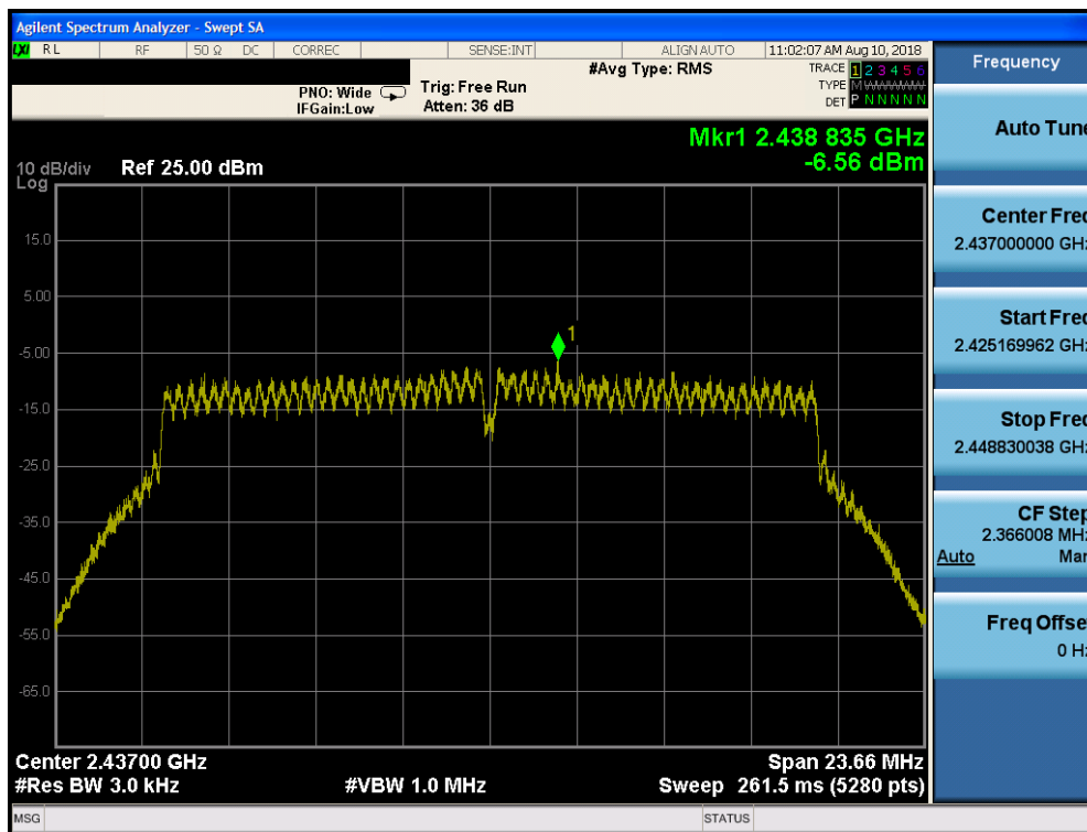
Plot 7-35. Power Spectral Density Plot SISO Core 0 (802.11n (2.4GHz) – Ch. 6)
