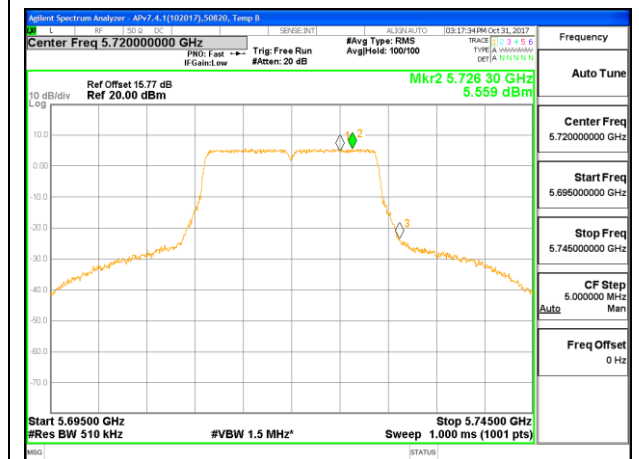
CHANNEL 144 PSD
