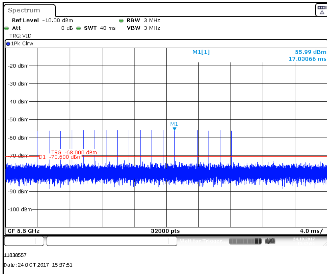
Radar Type 0 – full 18 pulse waveform
