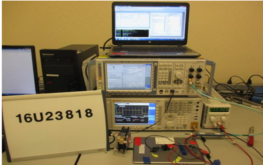
ANTENNA PORT CONDUCTED PHOTO
