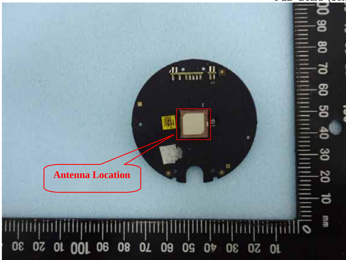
FIGURE 4 PCB Board (Solder Side)
