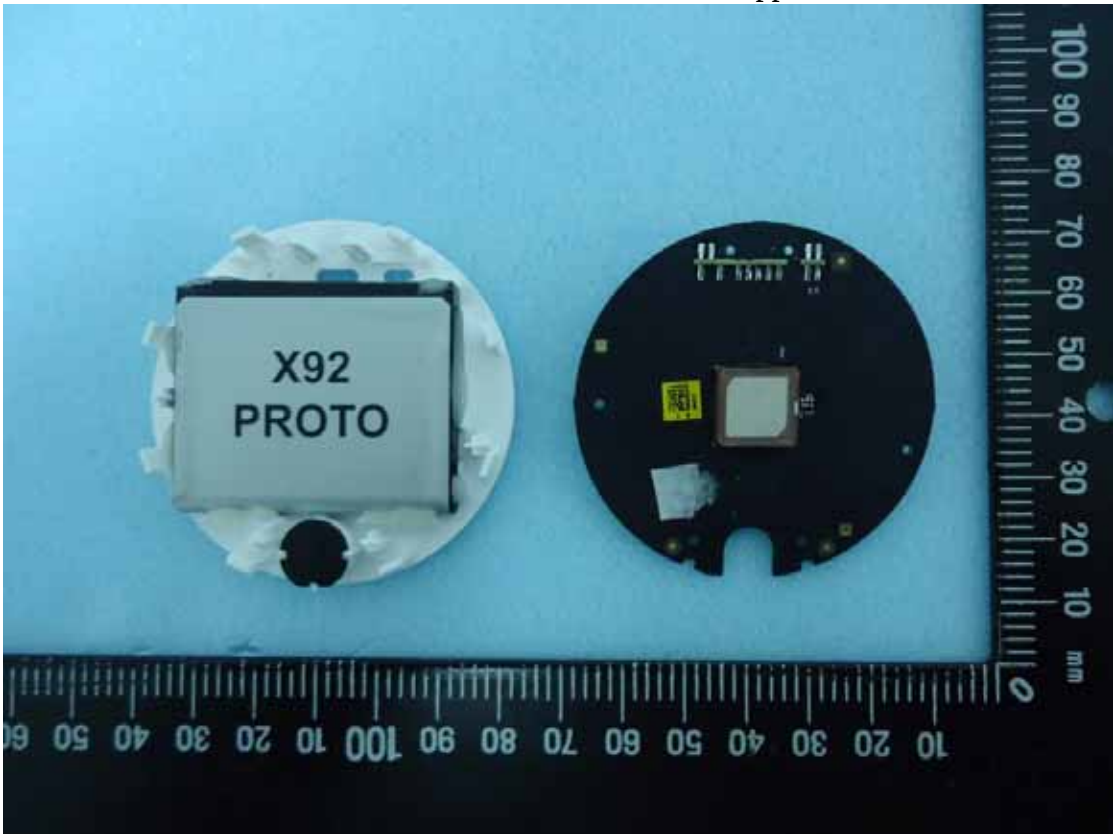
FIGURE 2 Internal Appearance (PCB Board Remove)
