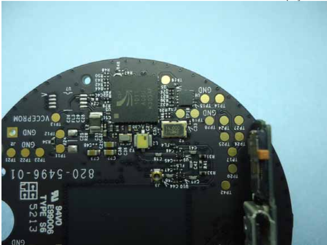
FIGURE 6 PCB Board (Crystal Oscillator)
