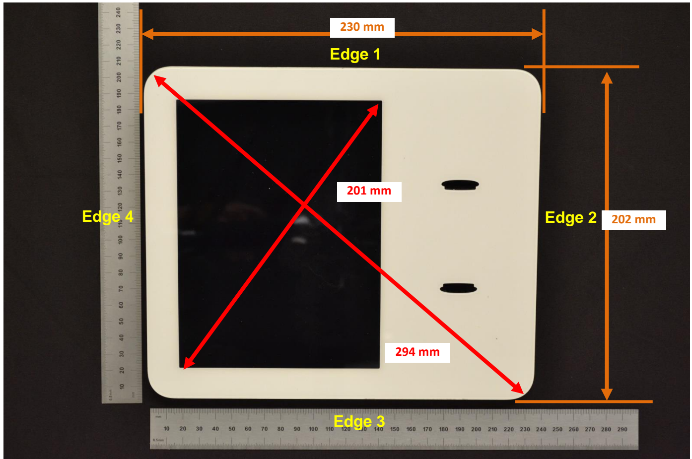
Overall Dimensions
