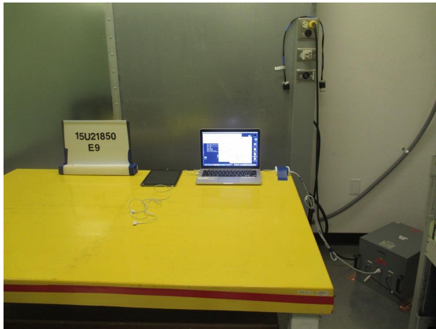
EUT WITH LAPTOP LINE CONDUCTED FRONT PHOTO
